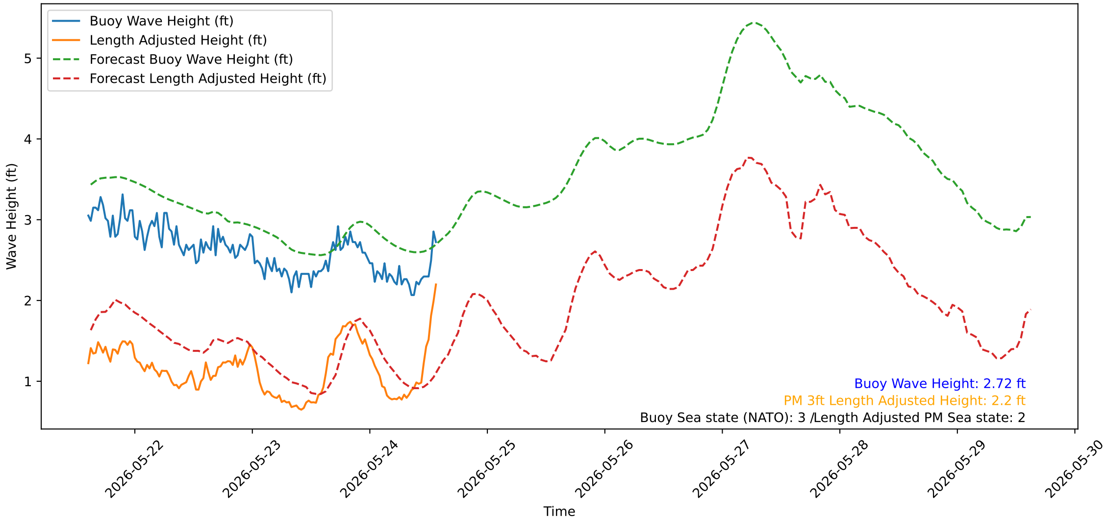
Wave Heights over Time for Green Beach at 2026-05-24 14:31:15
