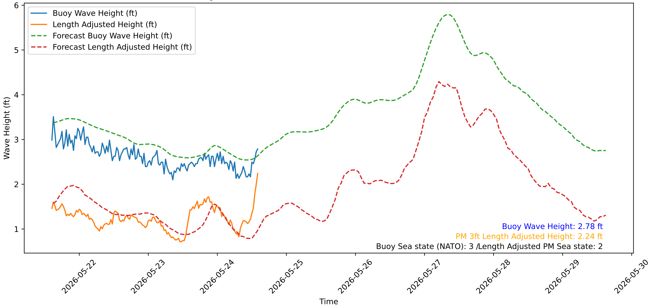
Wave Heights over Time for Oceanside Harbor at 2026-05-24 14:30:32
