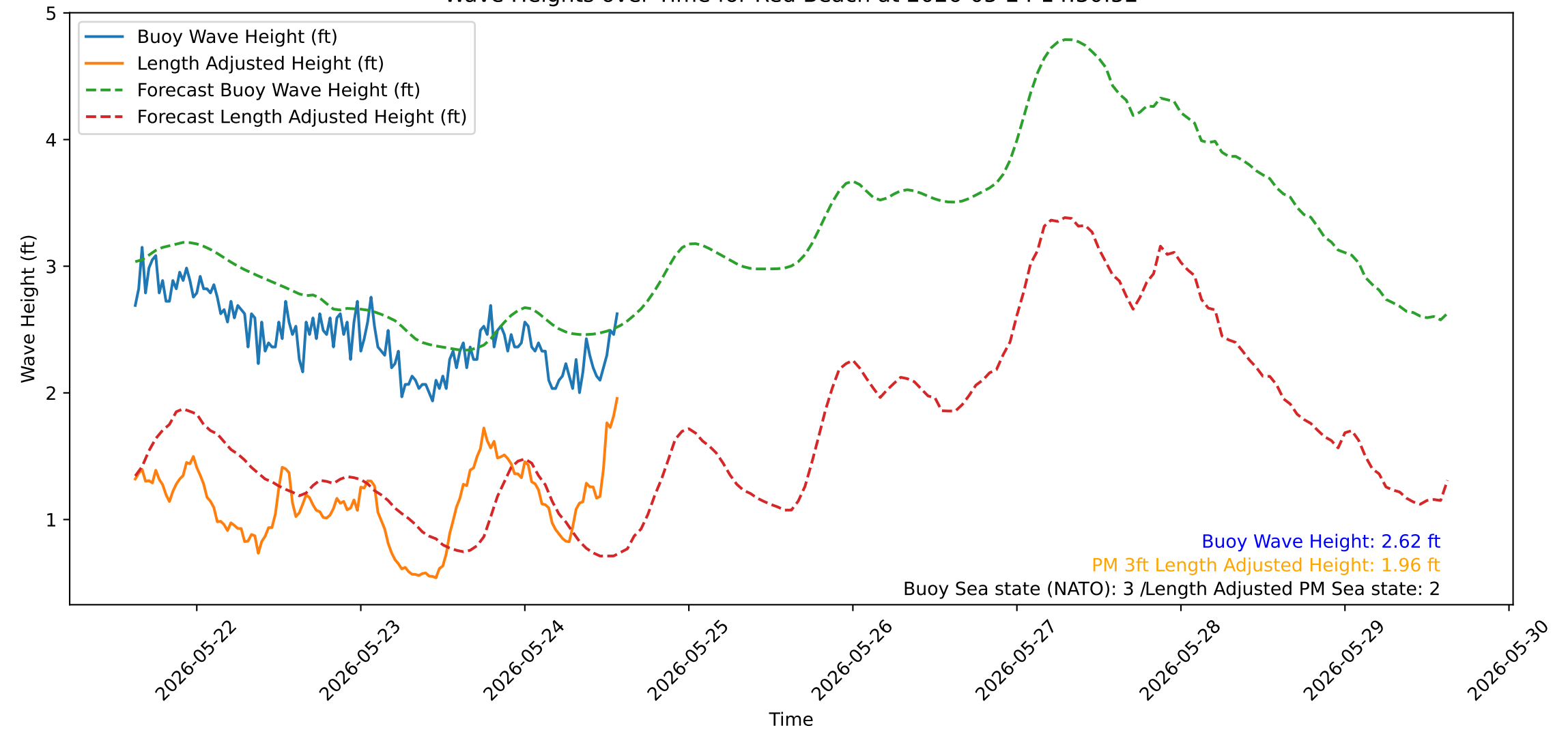
Wave Heights over Time for Red Beach at 2026-05-24 14:30:52
