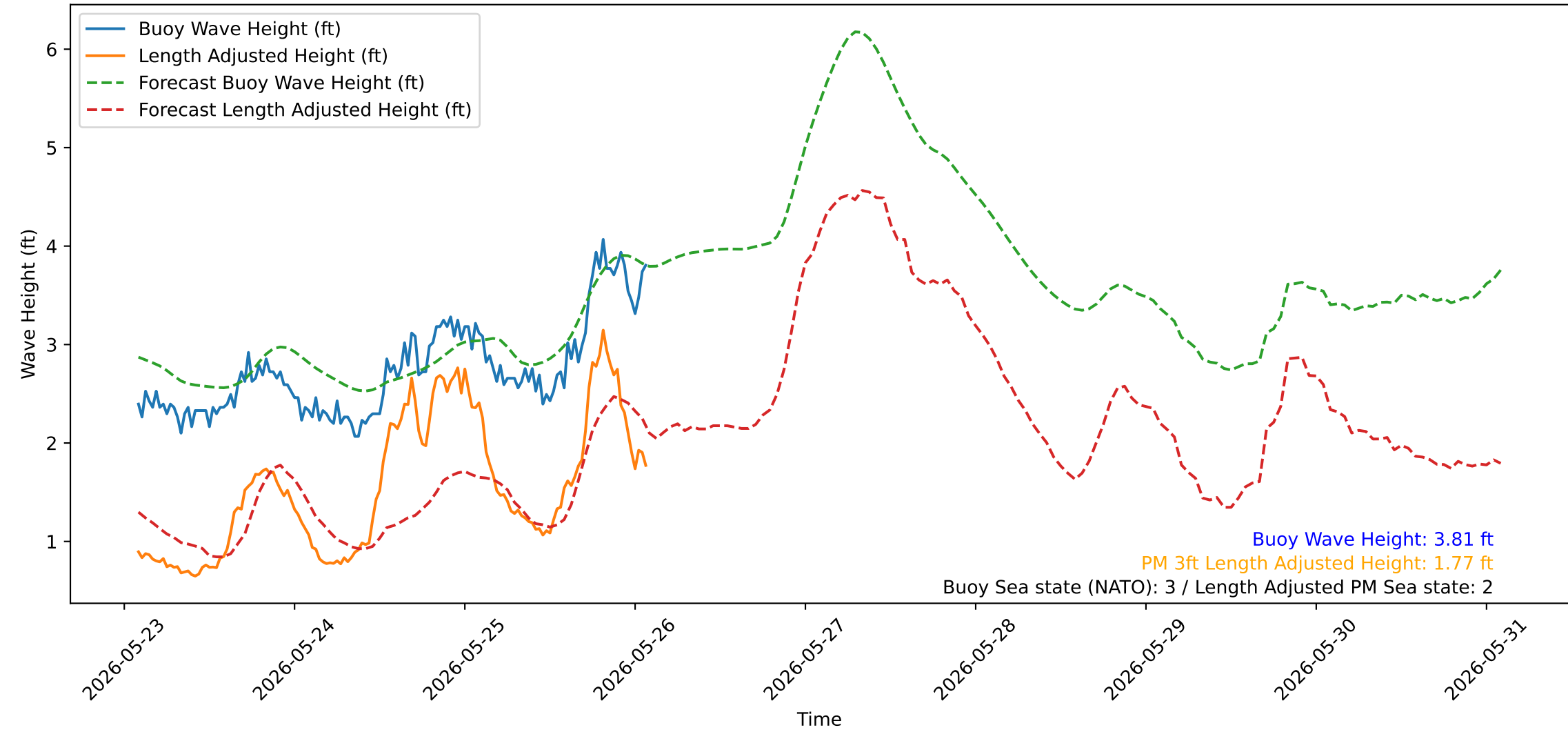
Wave Heights over Time for Green Beach at 2026-05-26 02:11:11
