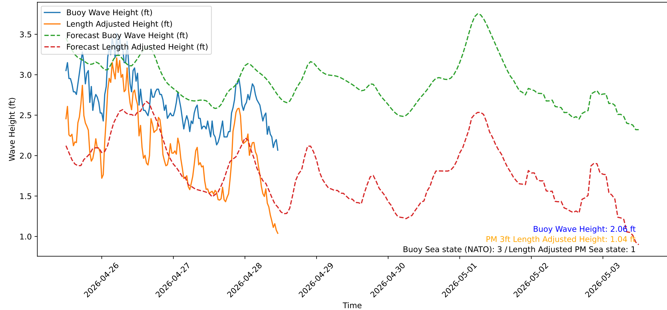
Wave Heights over Time for Green Beach at 2026-04-28 12:01:12
