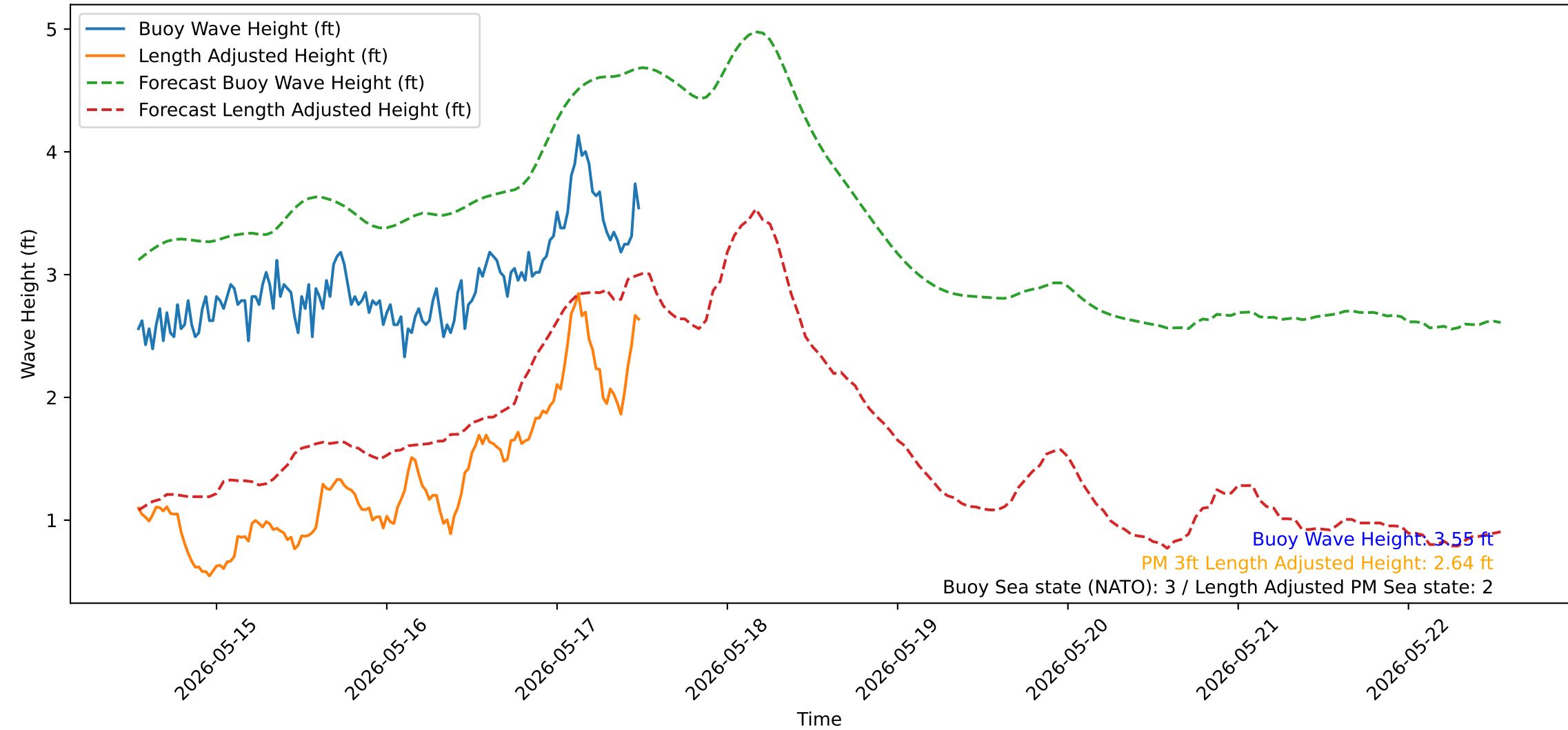
Wave Heights over Time for Red Beach at 2026-05-17 12:30:50
