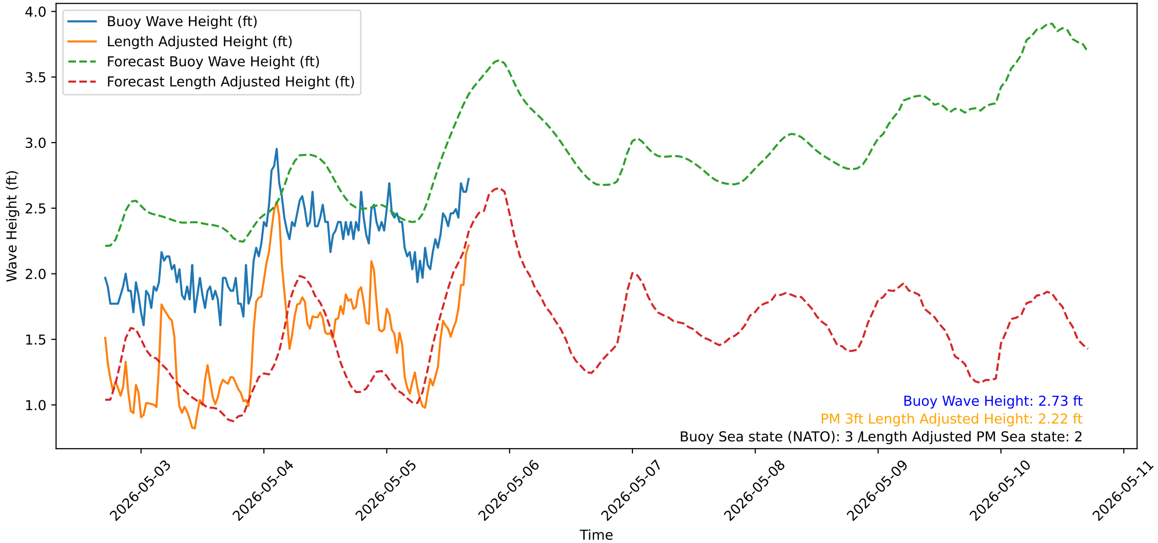
Wave Heights over Time for Red Beach at 2026-05-05 16:40:50
