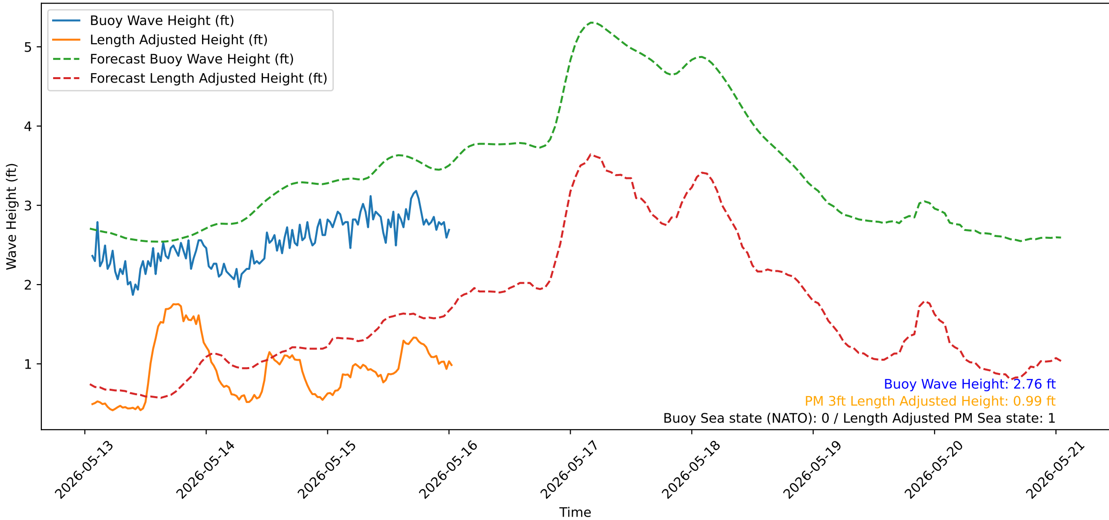
Wave Heights over Time for Red Beach at 2026-05-16 01:10:51
