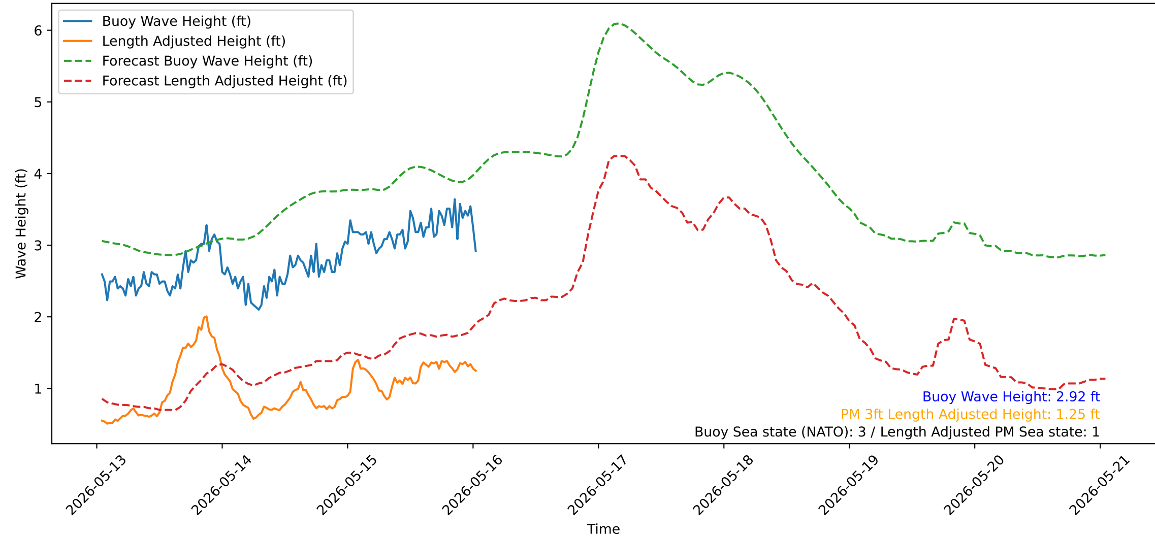
Wave Heights over Time for Green Beach at 2026-05-16 01:11:14
