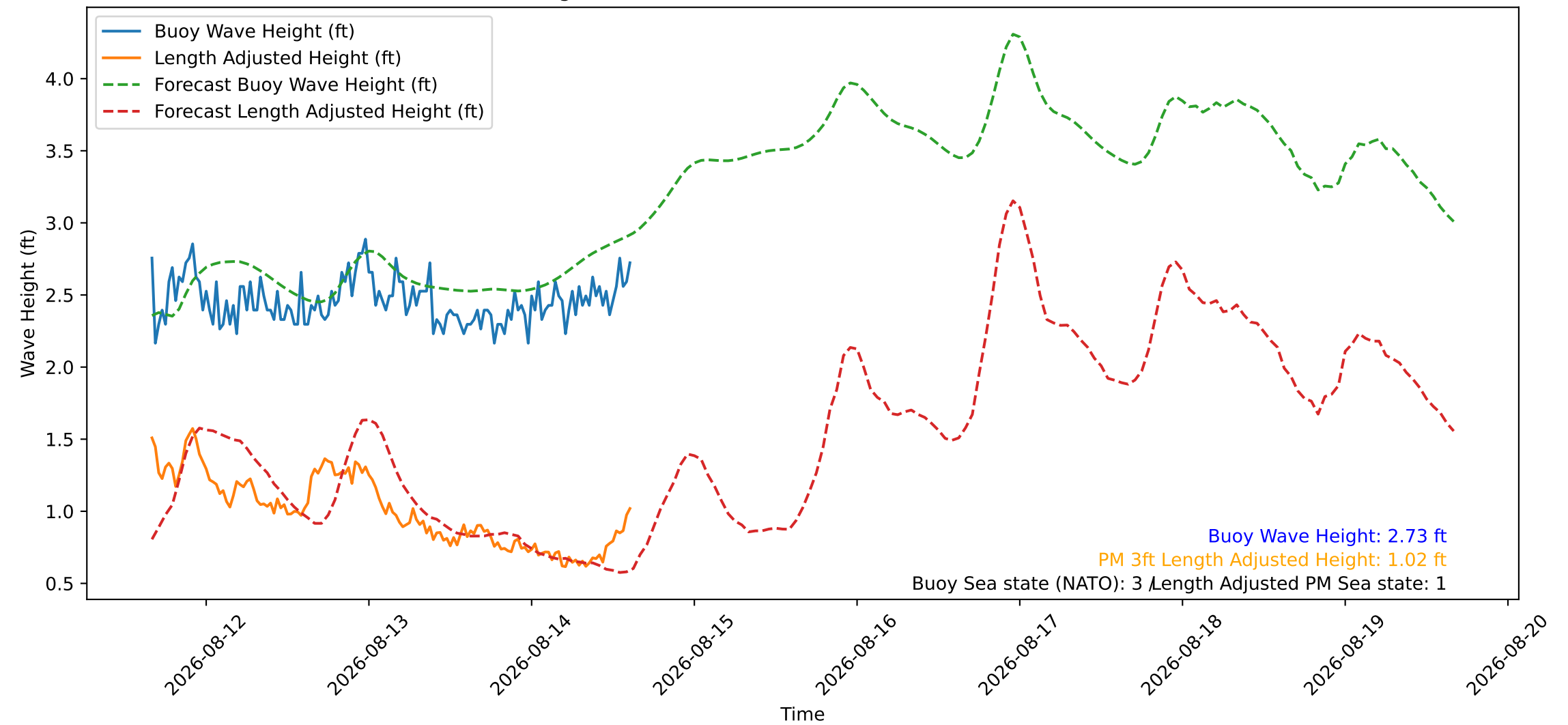
Wave Heights over Time for Red Beach at 2026-08-14 15:40:46
