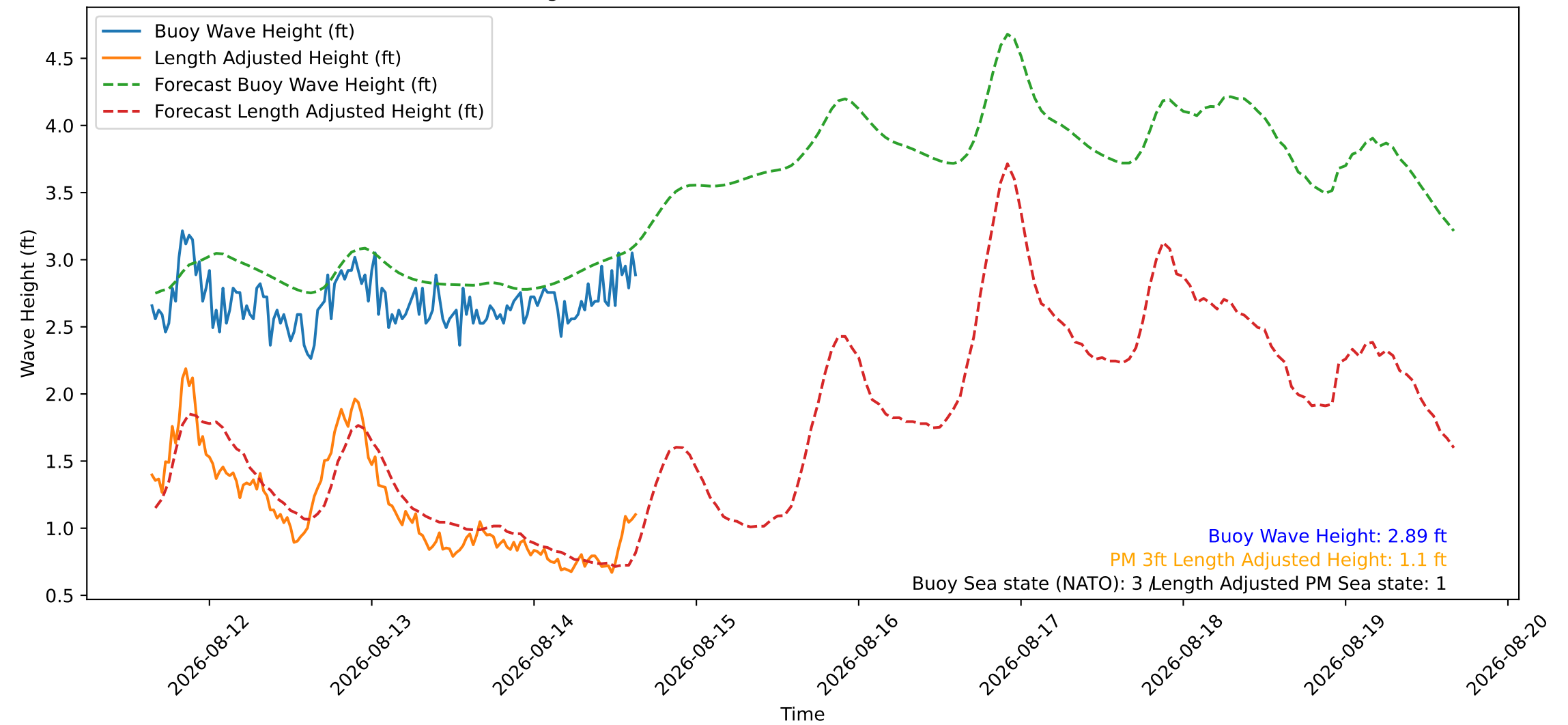
Wave Heights over Time for Green Beach at 2026-08-14 15:41:09
