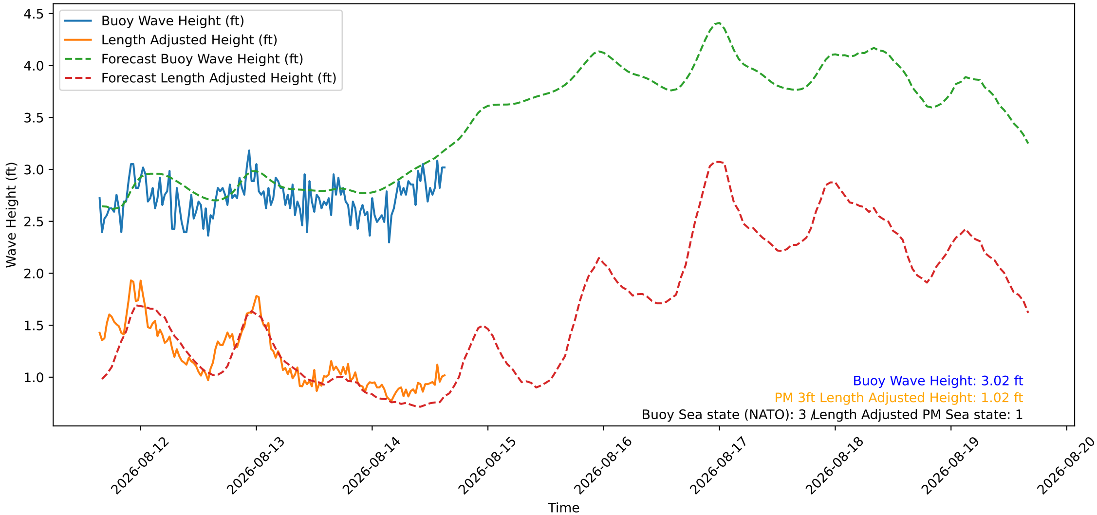
Wave Heights over Time for Oceanside Harbor at 2026-08-14 15:40:27
