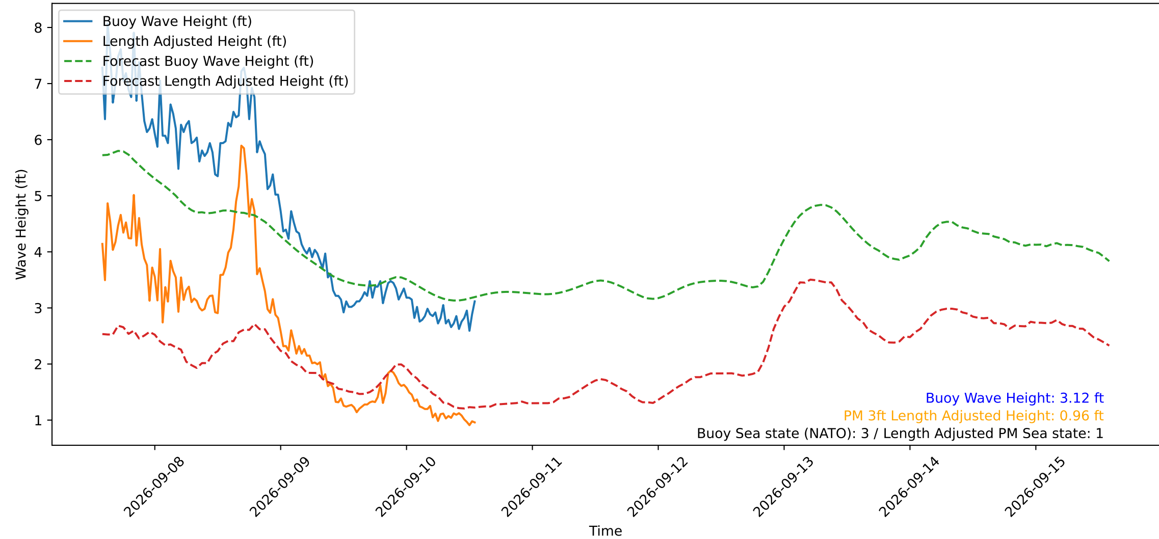
Wave Heights over Time for Green Beach at 2026-09-10 13:51:14
