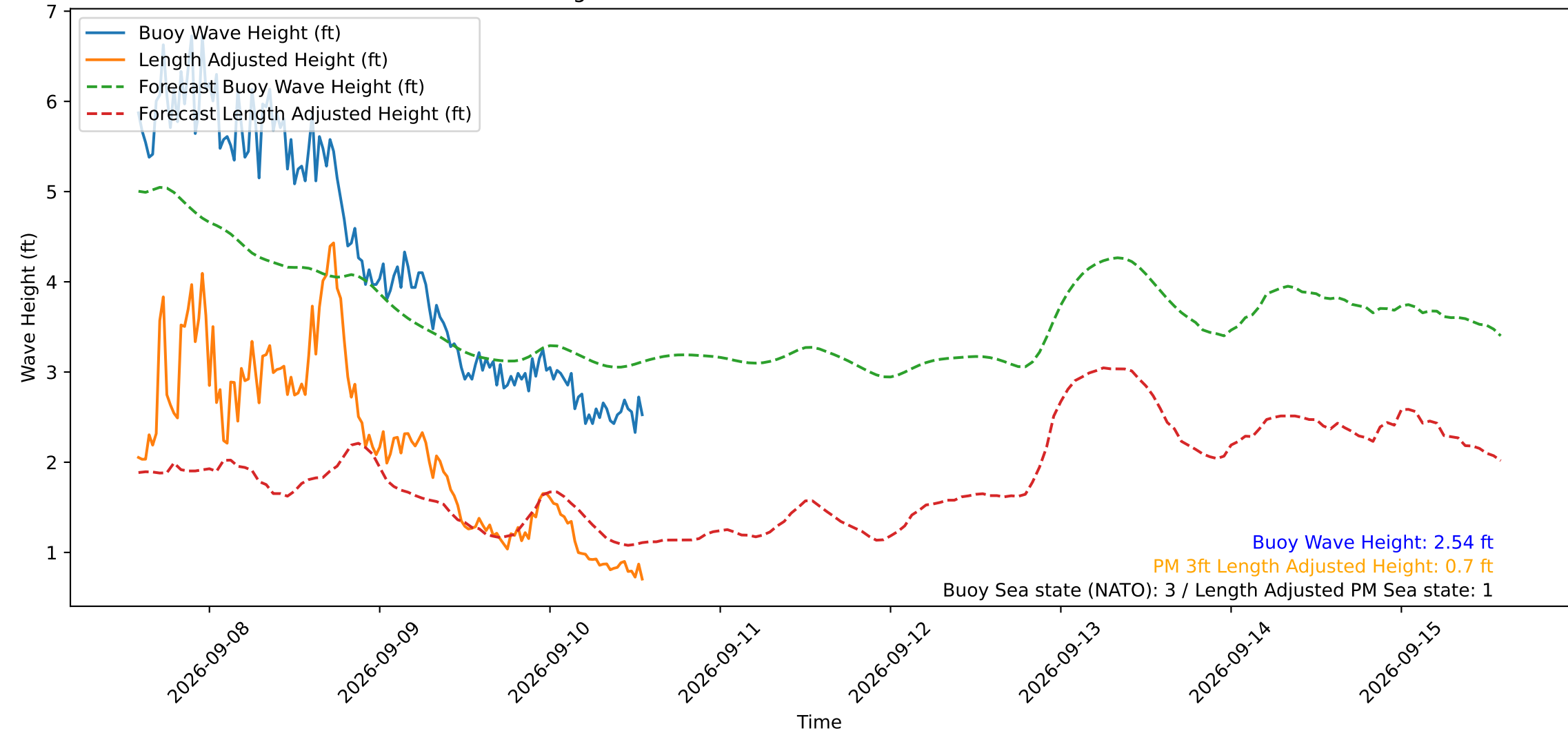
Wave Heights over Time for Red Beach at 2026-09-10 13:50:50
