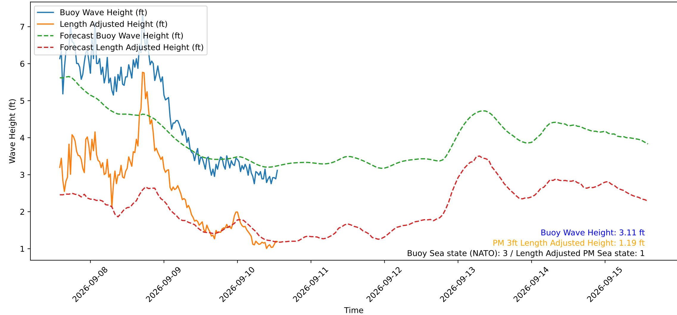
Wave Heights over Time for Oceanside Harbor at 2026-09-10 13:50:29
