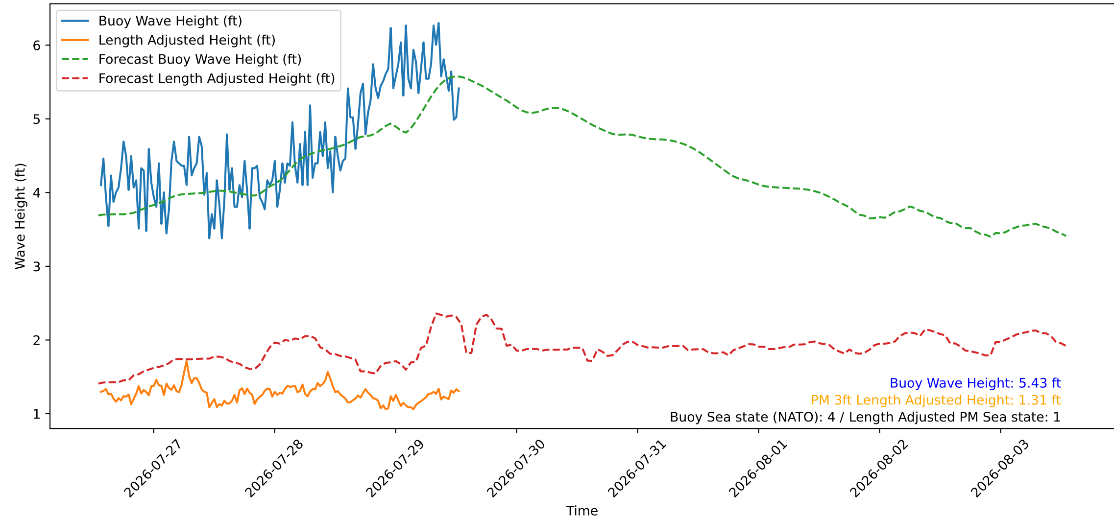
Wave Heights over Time for Green Beach at 2026-07-29 13:21:10
