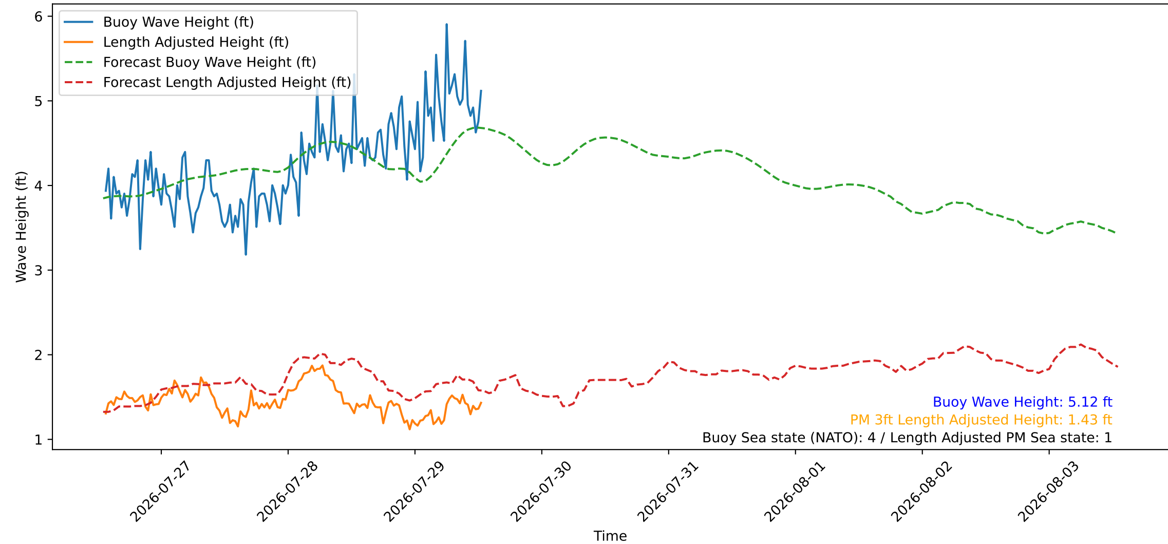
Wave Heights over Time for Oceanside Harbor at 2026-07-29 13:20:26
