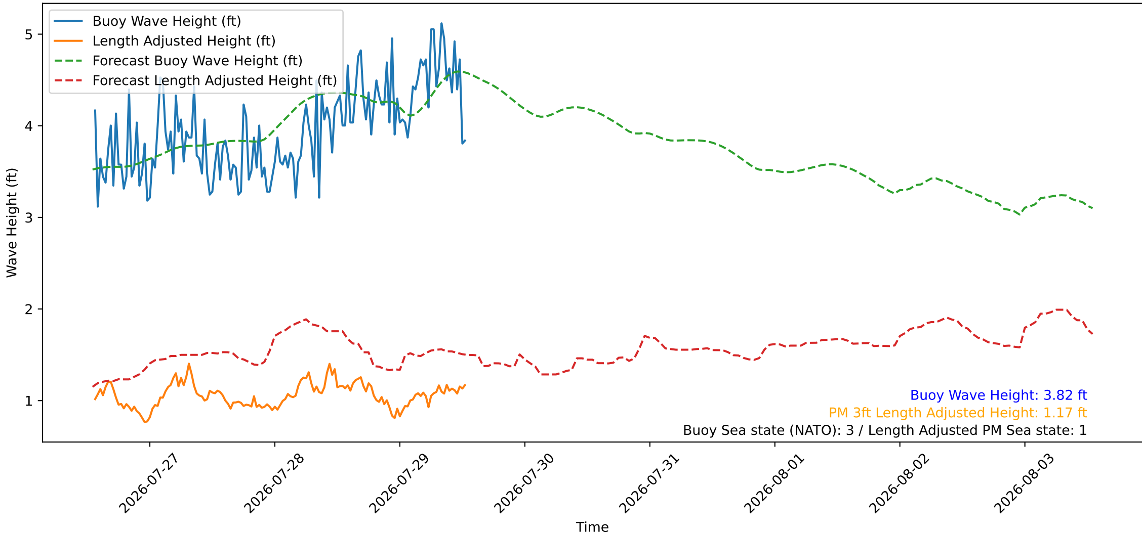
Wave Heights over Time for Red Beach at 2026-07-29 13:20:47
