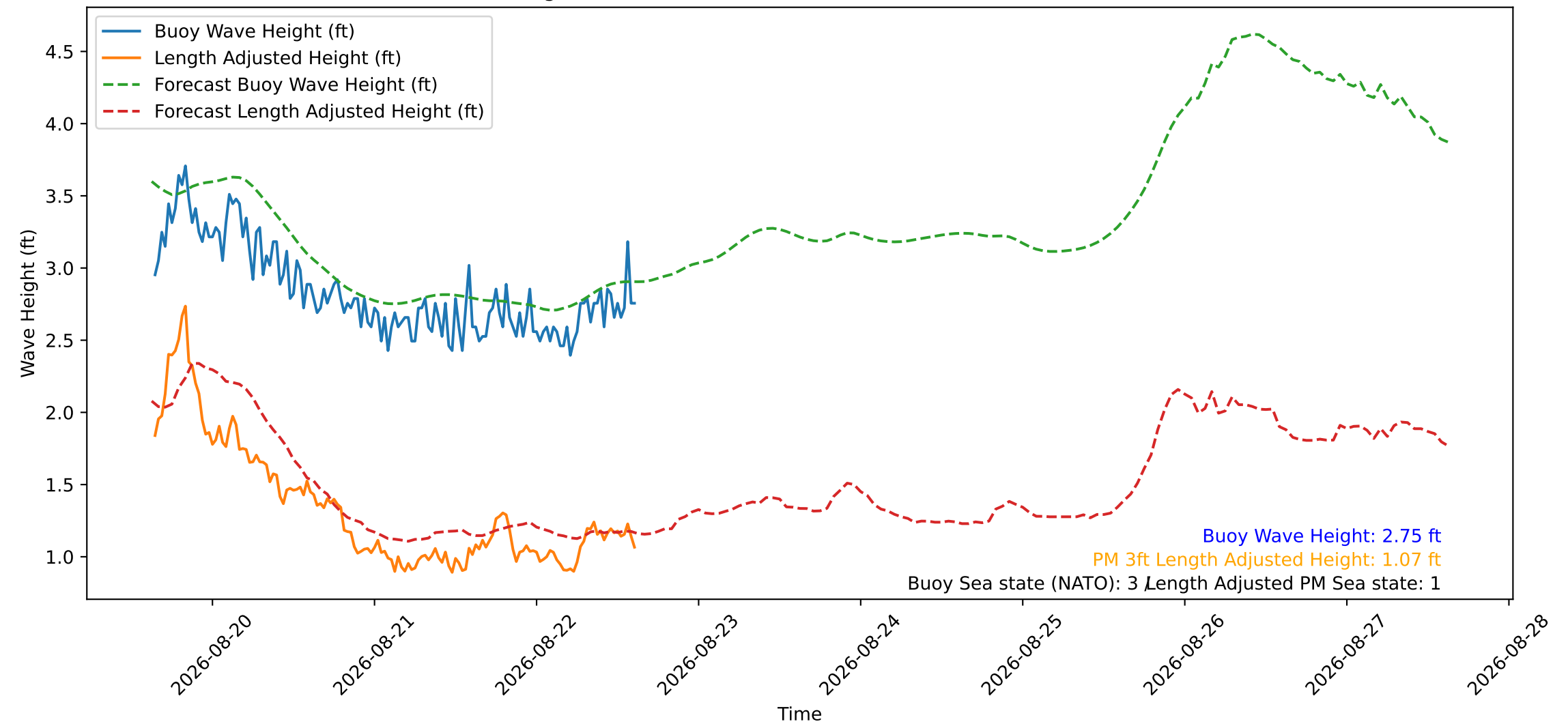
Wave Heights over Time for Green Beach at 2026-08-22 15:11:12
