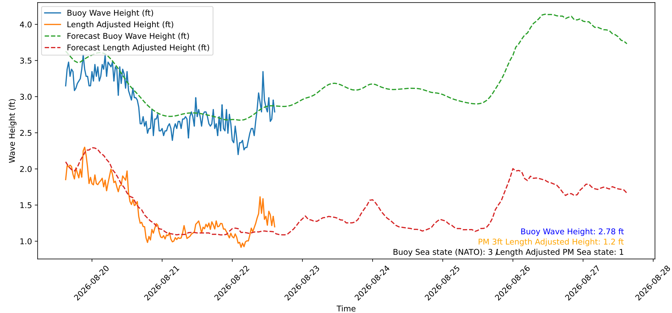
Wave Heights over Time for Oceanside Harbor at 2026-08-22 15:10:30
