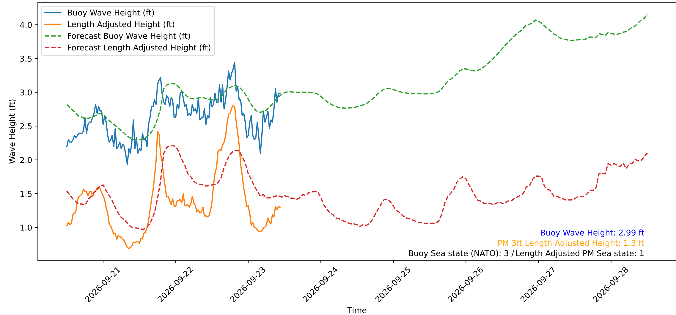
Wave Heights over Time for Green Beach at 2026-09-23 11:31:11
