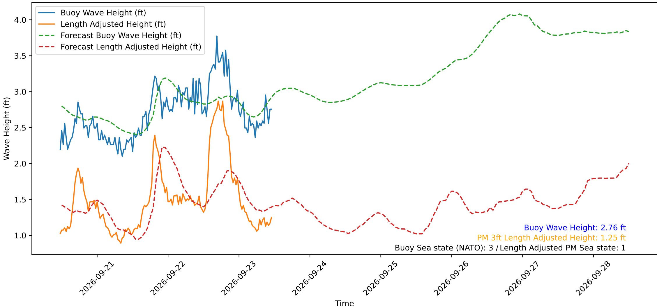
Wave Heights over Time for Oceanside Harbor at 2026-09-23 11:30:29
