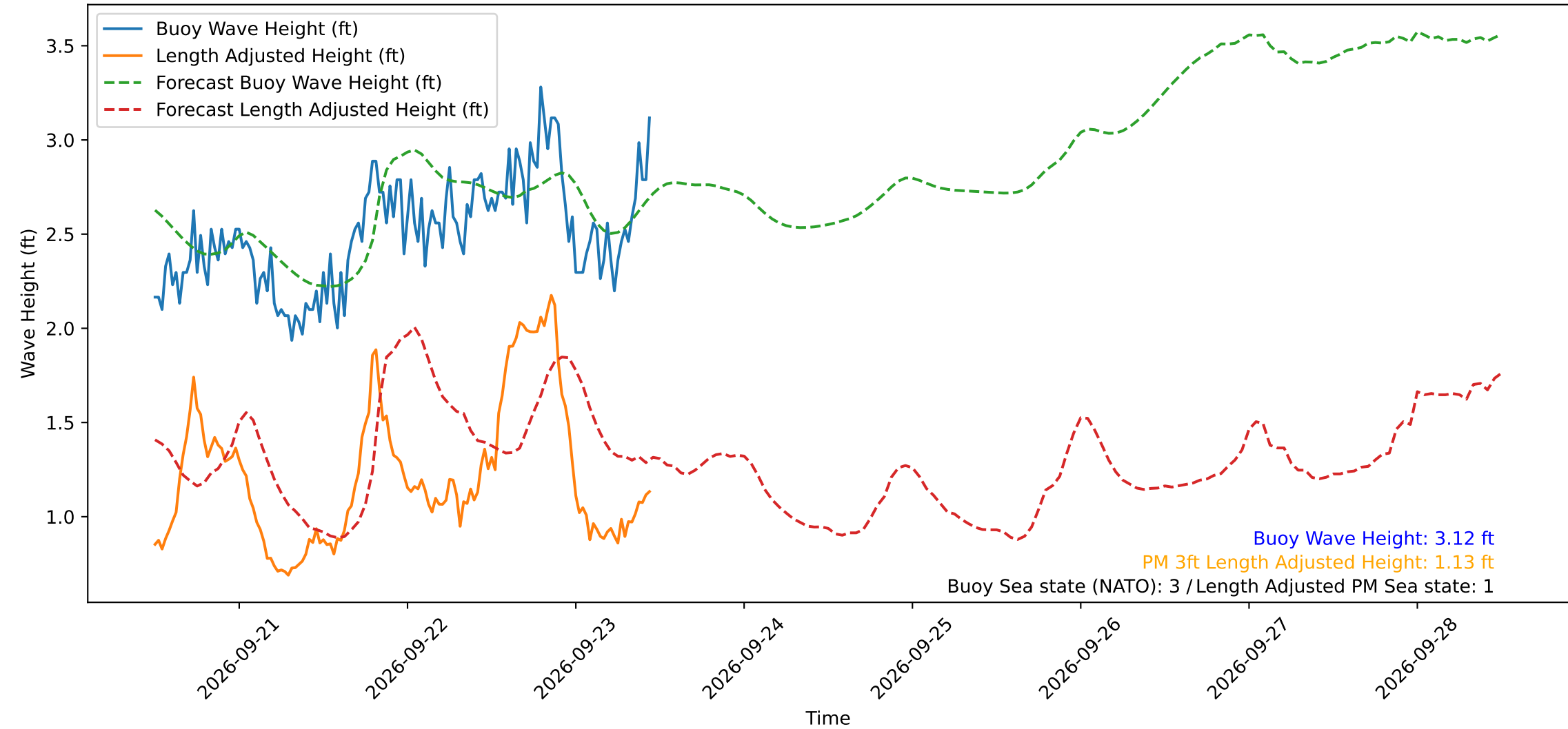
Wave Heights over Time for Red Beach at 2026-09-23 11:30:49
