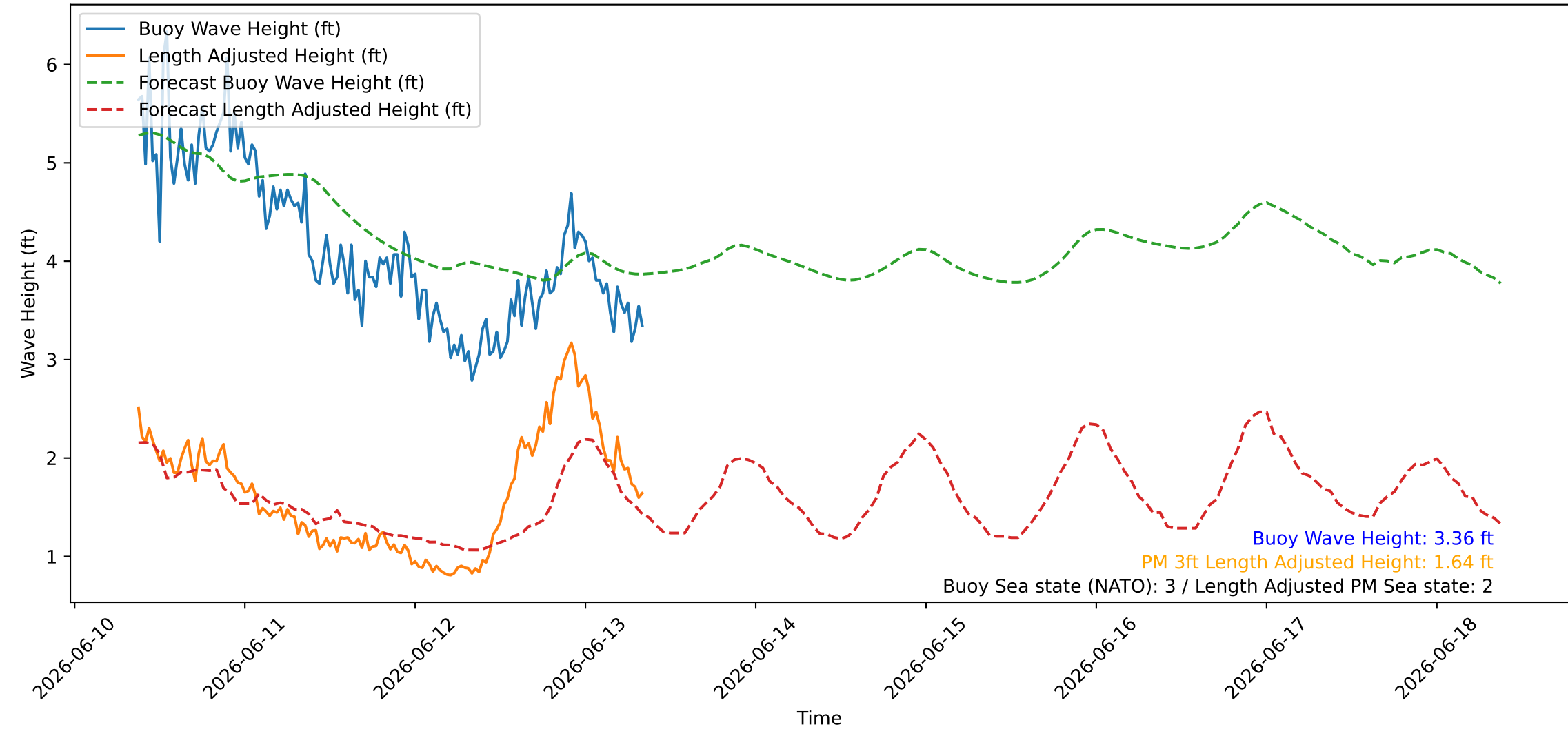
Wave Heights over Time for Oceanside Harbor at 2026-06-13 08:50:26
