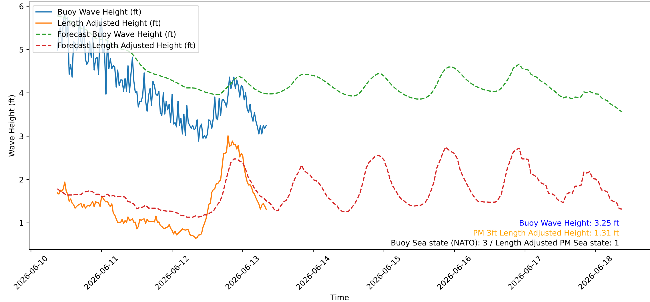
Wave Heights over Time for Green Beach at 2026-06-13 08:51:09
