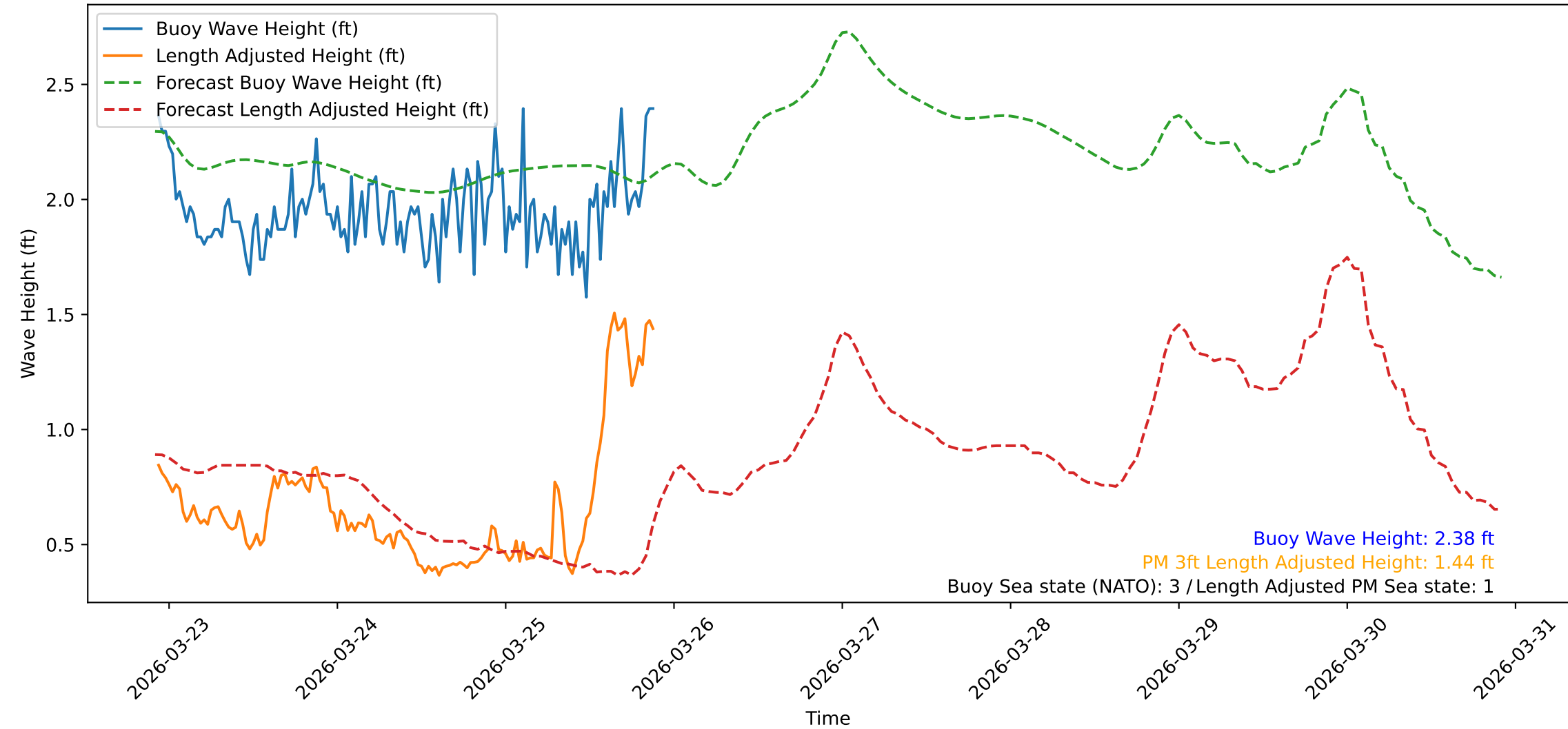
Wave Heights over Time for Red Beach at 2026-03-25 22:00:47
