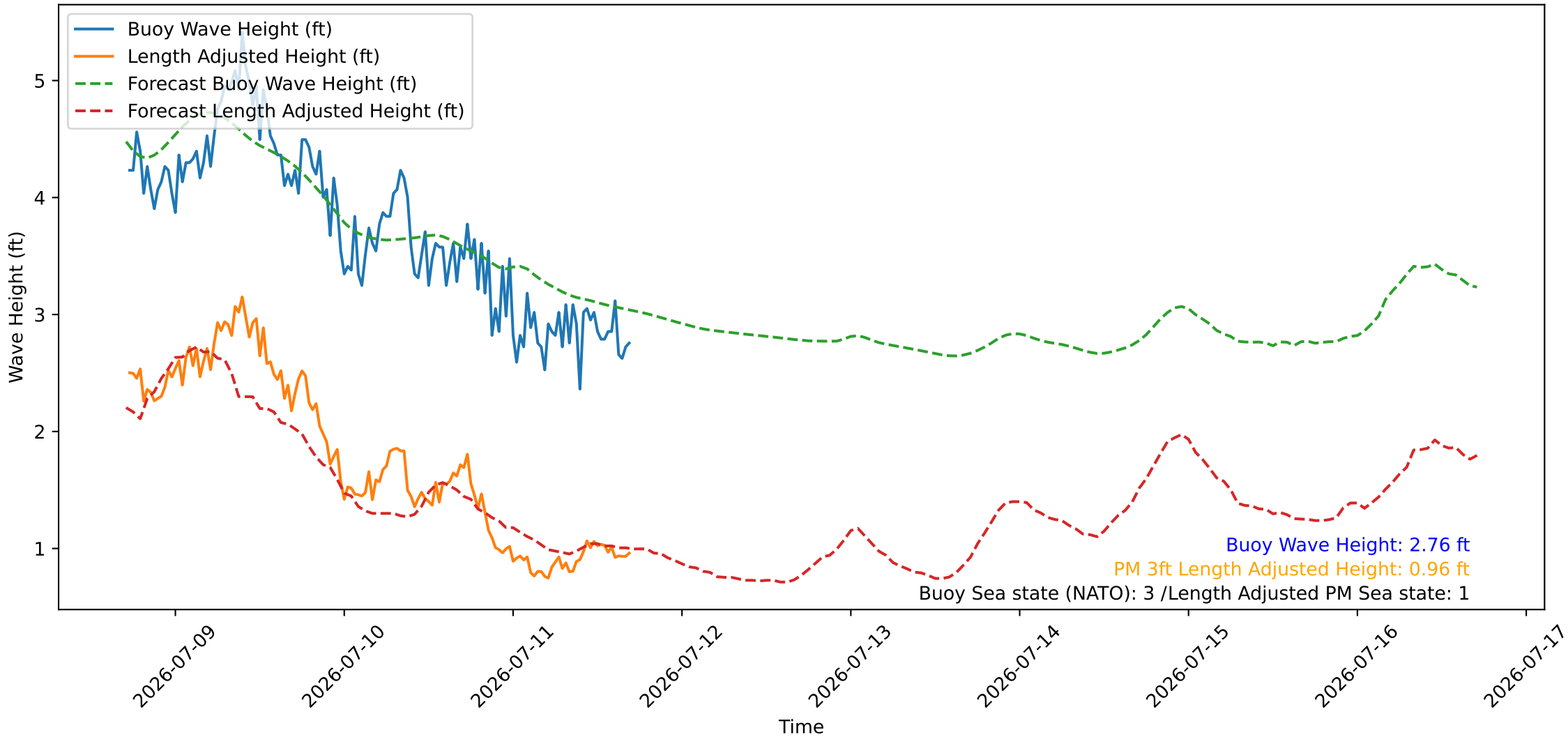
Wave Heights over Time for Oceanside Harbor at 2026-07-11 17:20:26
