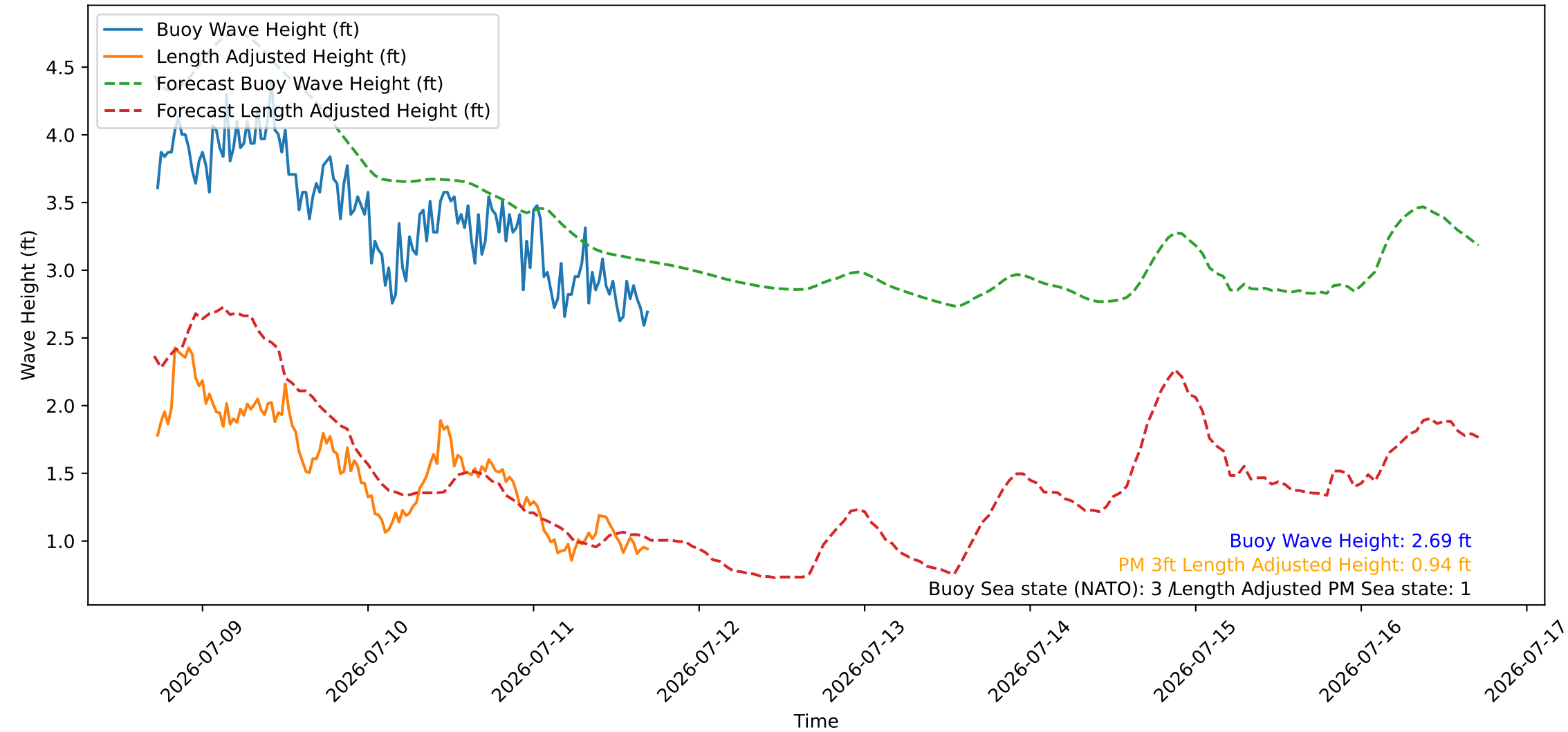
Wave Heights over Time for Green Beach at 2026-07-11 17:21:08
