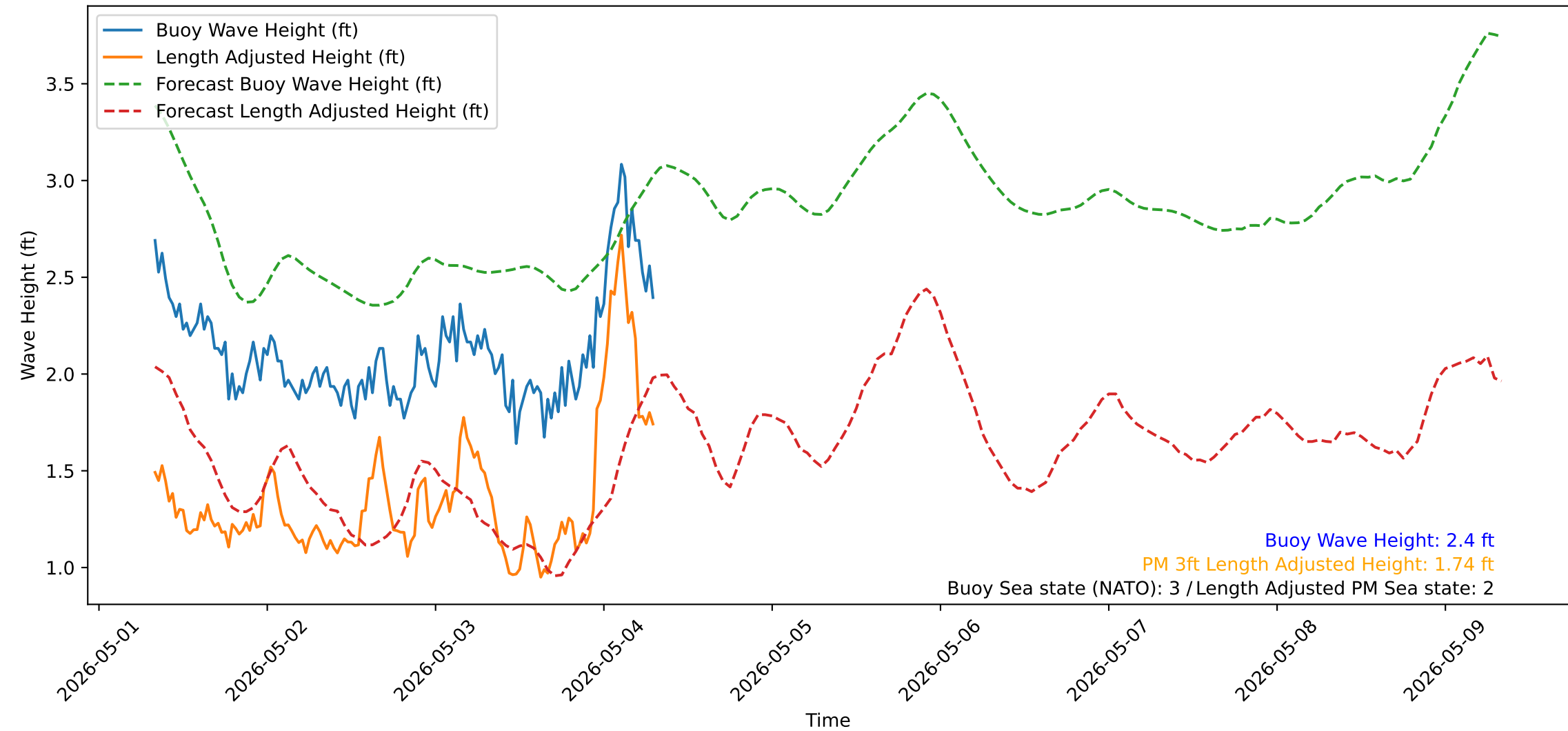
Wave Heights over Time for Oceanside Harbor at 2026-05-04 08:00:31
