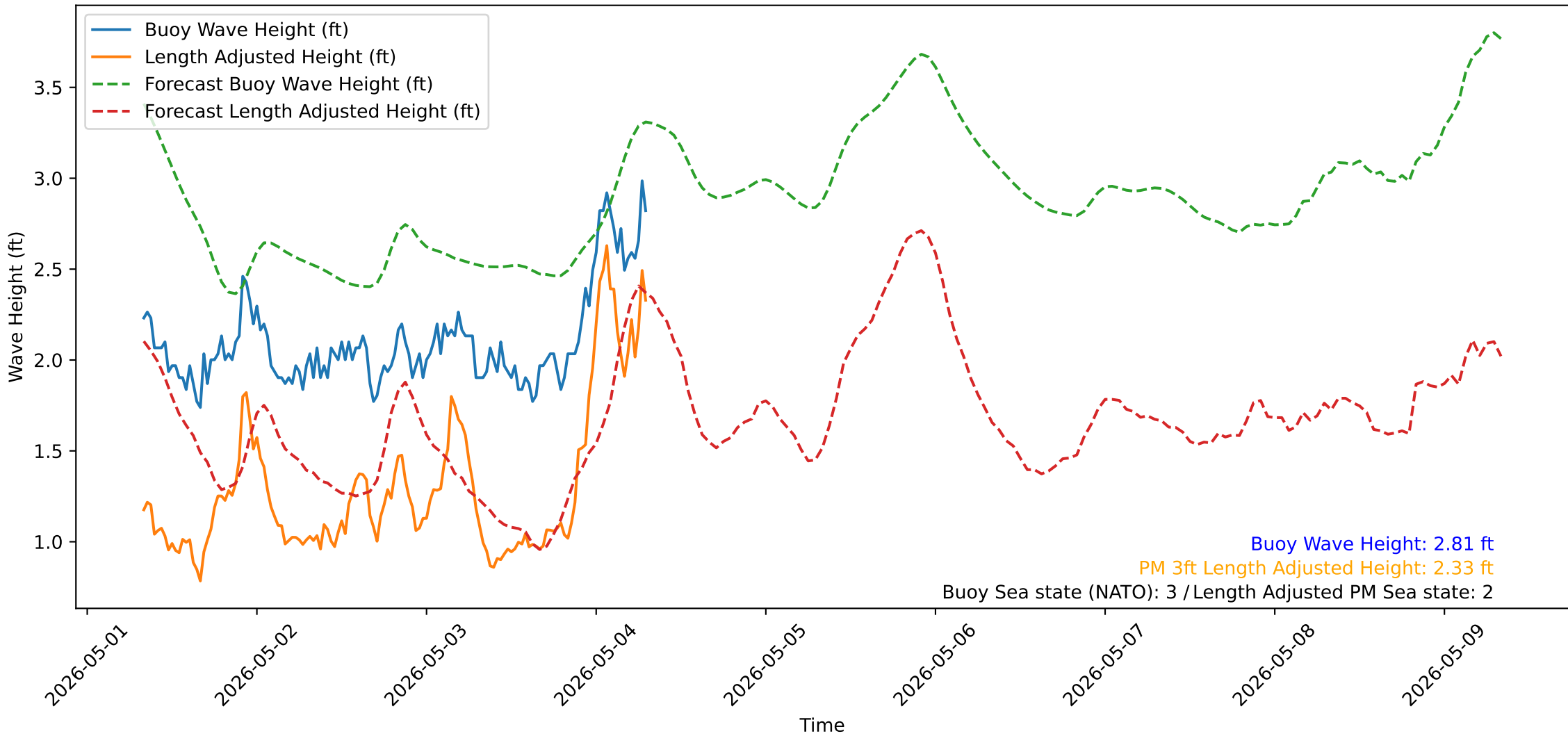
Wave Heights over Time for Green Beach at 2026-05-04 08:01:12
