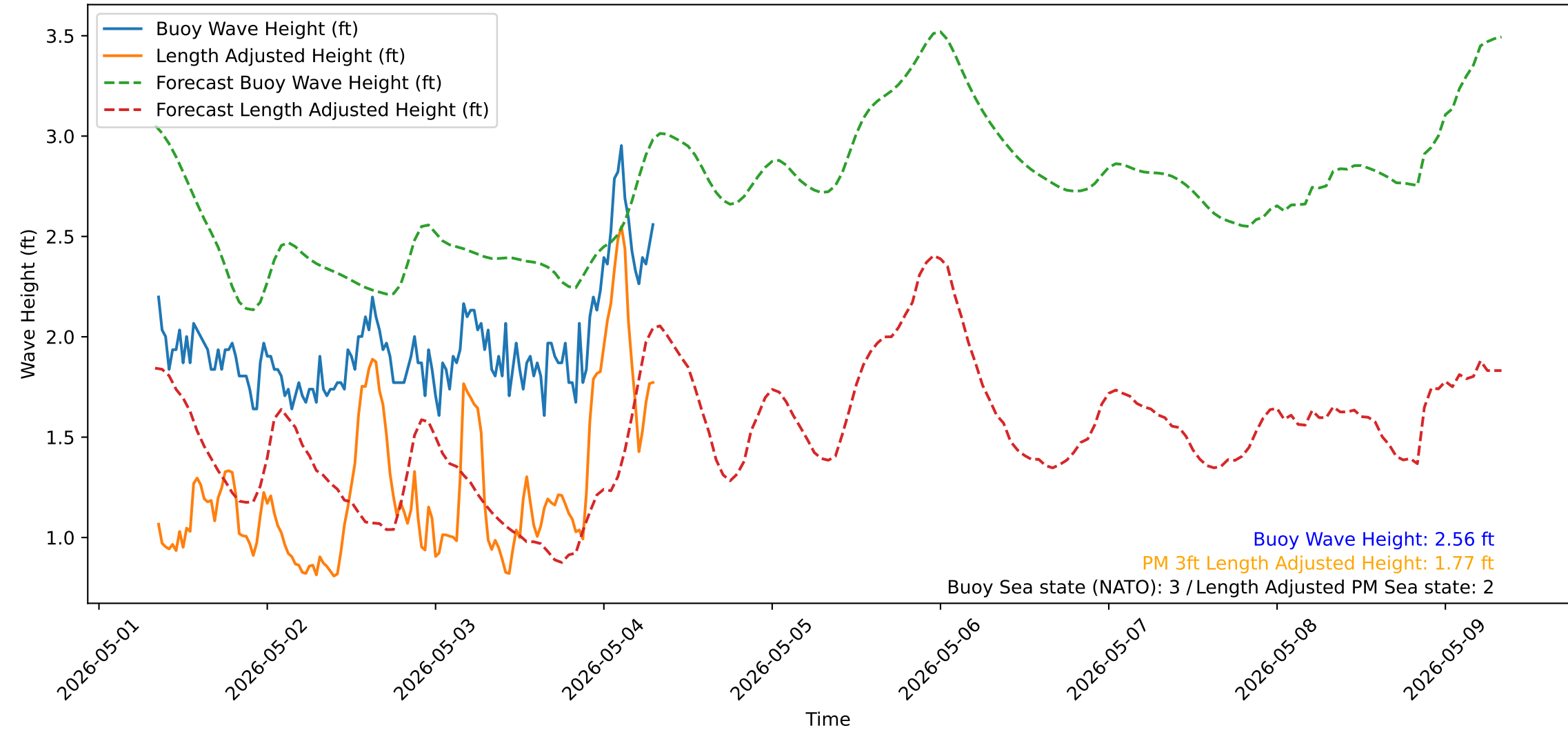
Wave Heights over Time for Red Beach at 2026-05-04 08:00:50
