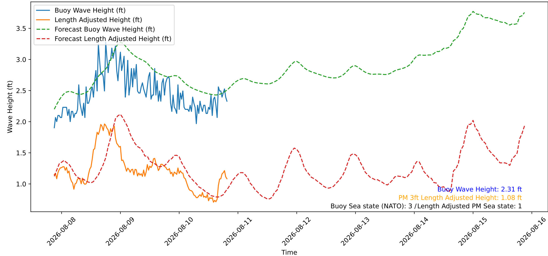
Wave Heights over Time for Oceanside Harbor at 2026-08-10 20:50:26
