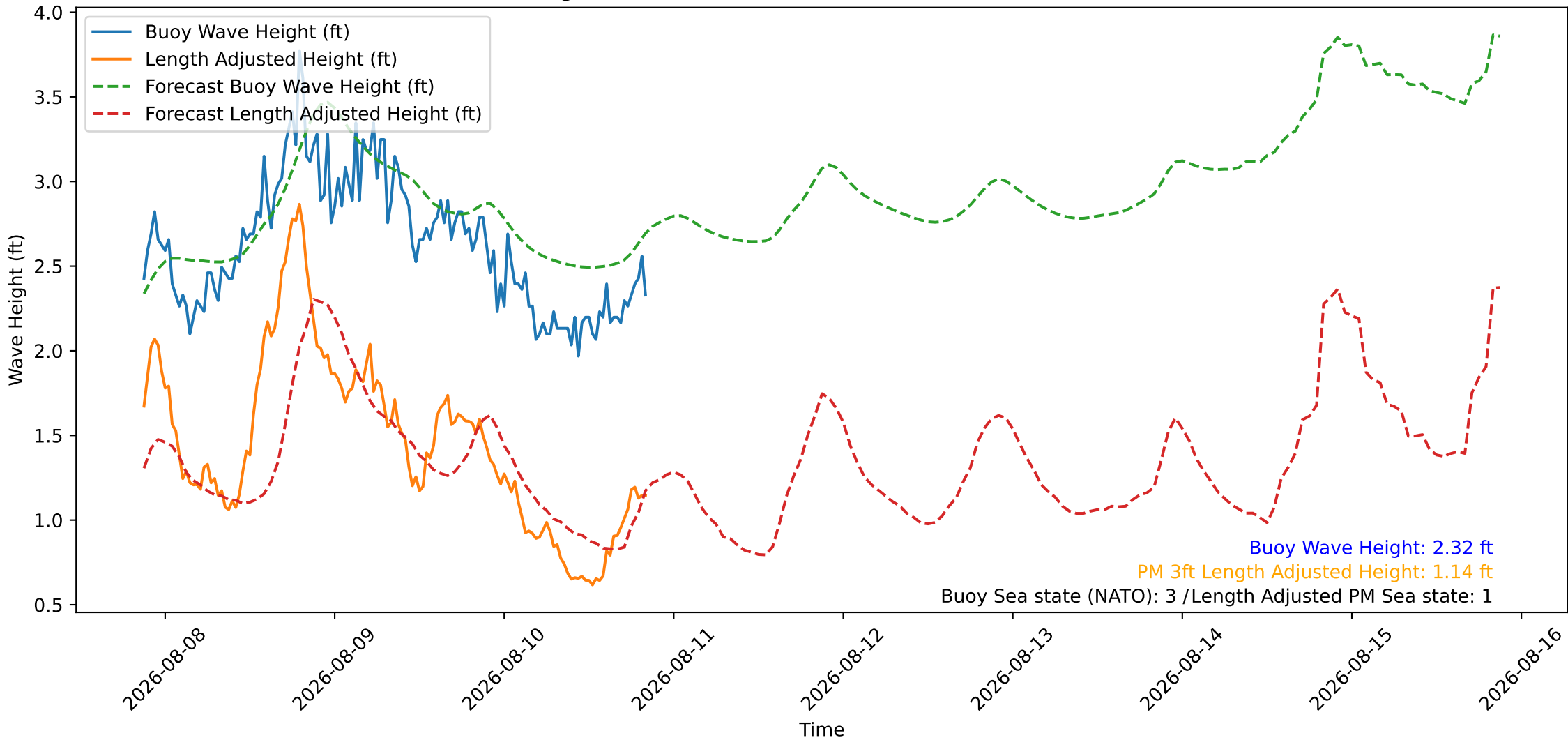
Wave Heights over Time for Green Beach at 2026-08-10 20:51:10
