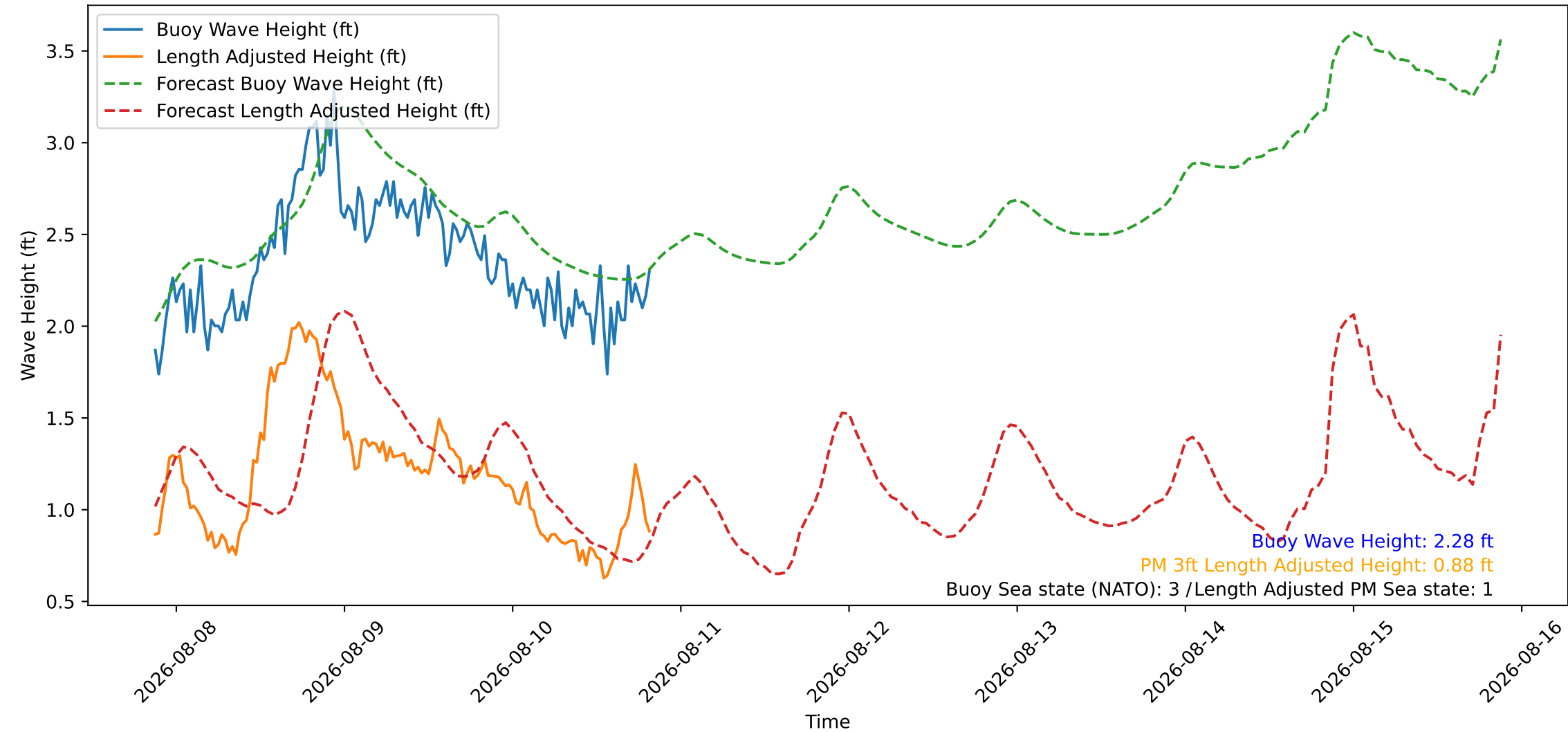
Wave Heights over Time for Red Beach at 2026-08-10 20:50:47
