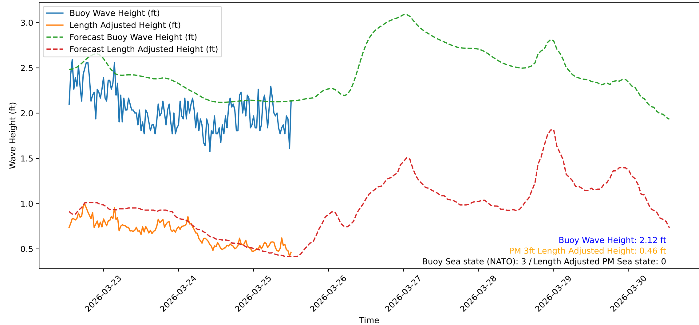
Wave Heights over Time for Oceanside Harbor at 2026-03-25 12:50:31
