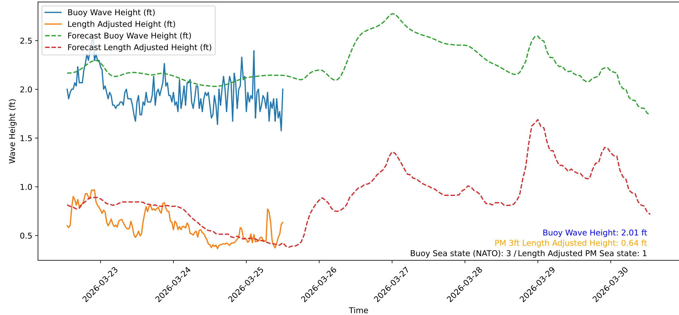
Wave Heights over Time for Red Beach at 2026-03-25 12:50:47
