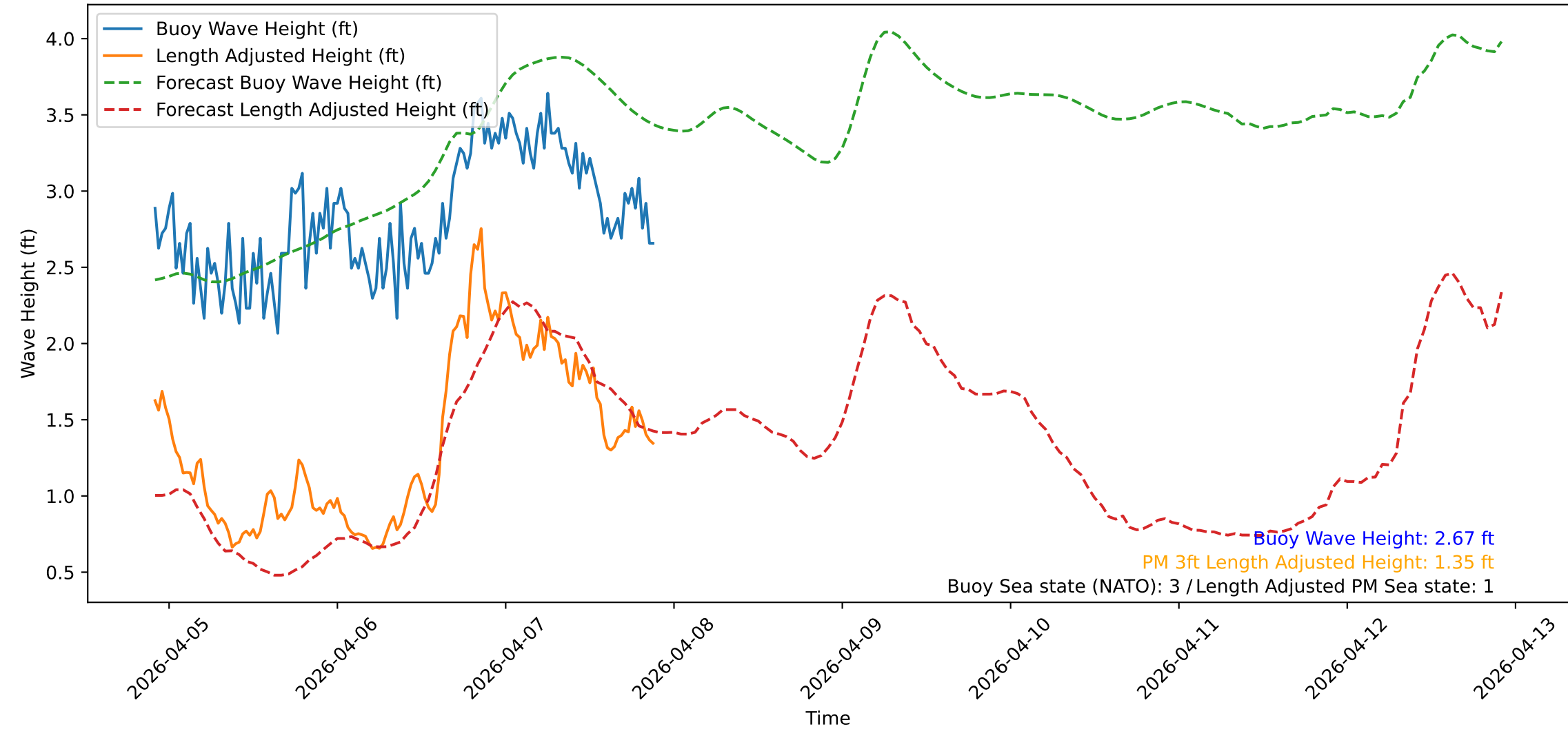
Wave Heights over Time for Oceanside Harbor at 2026-04-07 21:50:32
