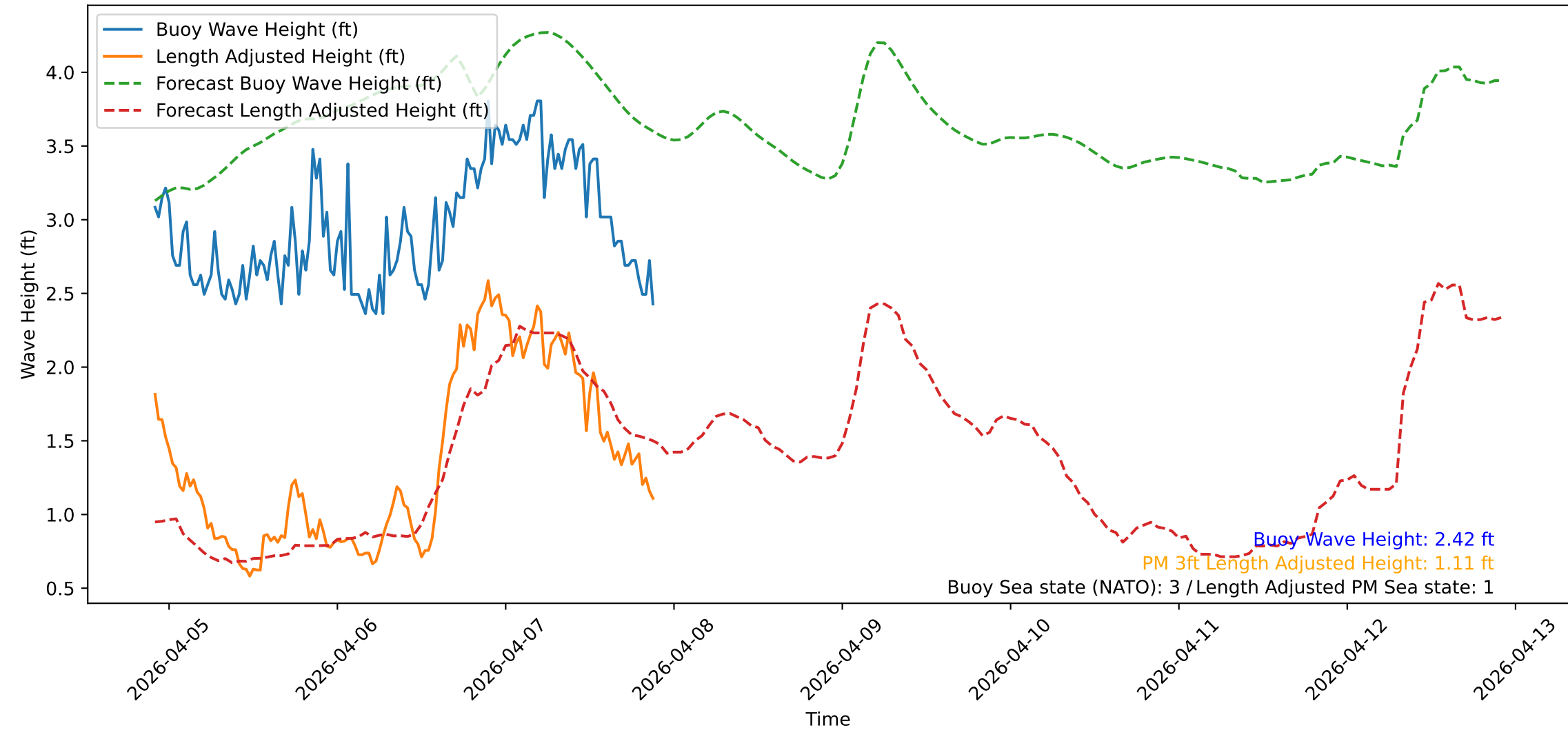
Wave Heights over Time for Green Beach at 2026-04-07 21:51:12
