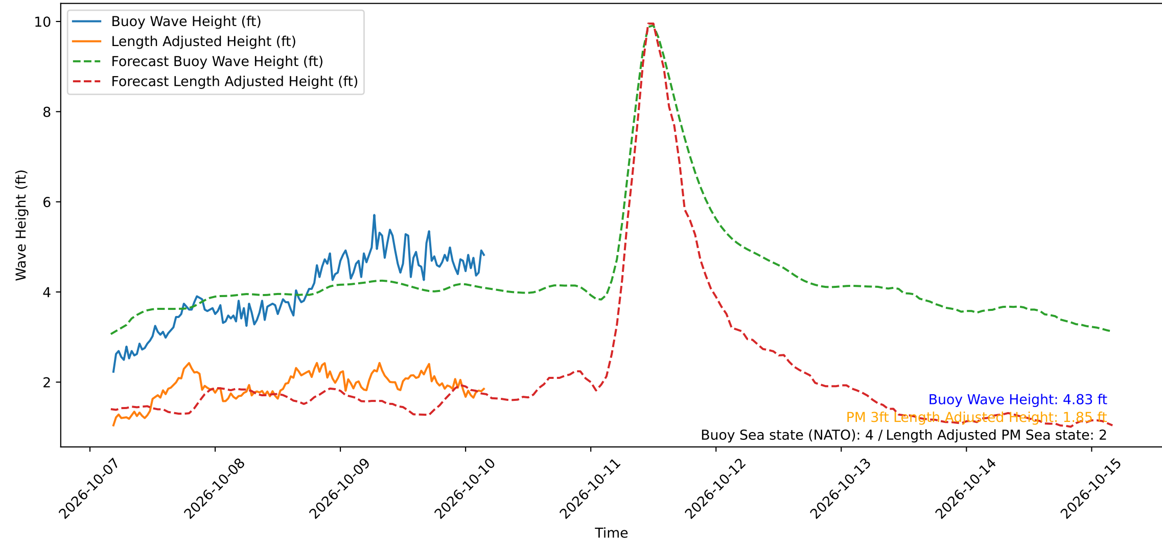
Wave Heights over Time for Red Beach at 2026-10-10 04:20:51
