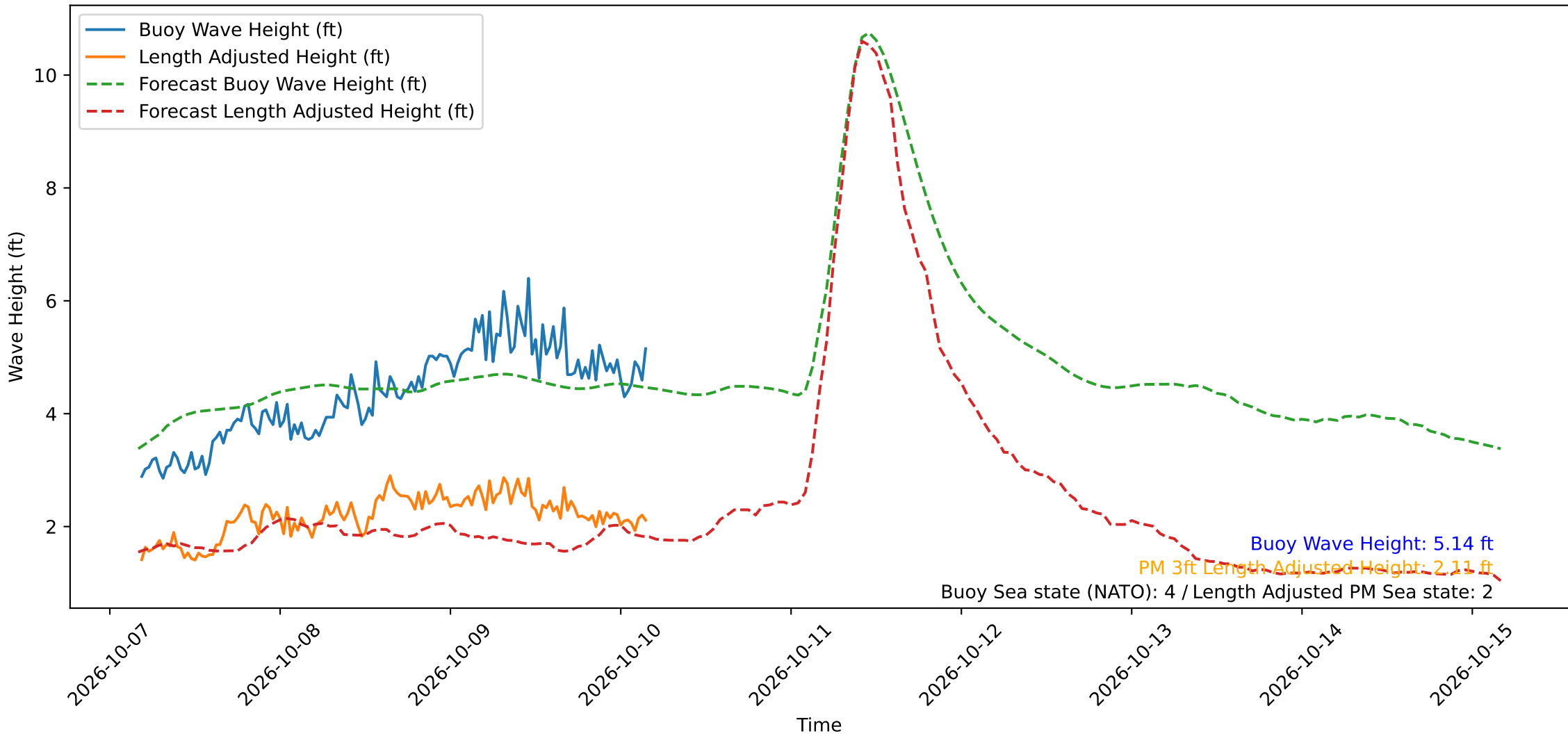
Wave Heights over Time for Oceanside Harbor at 2026-10-10 04:20:29
