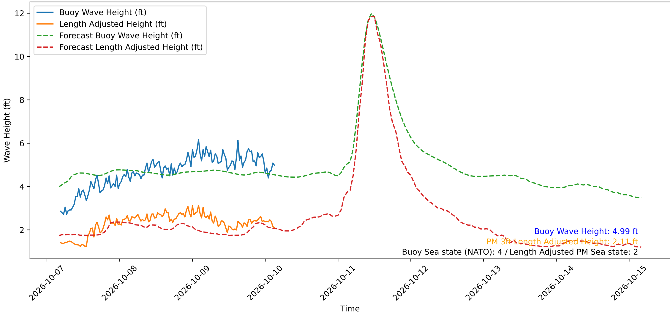
Wave Heights over Time for Green Beach at 2026-10-10 04:21:14
