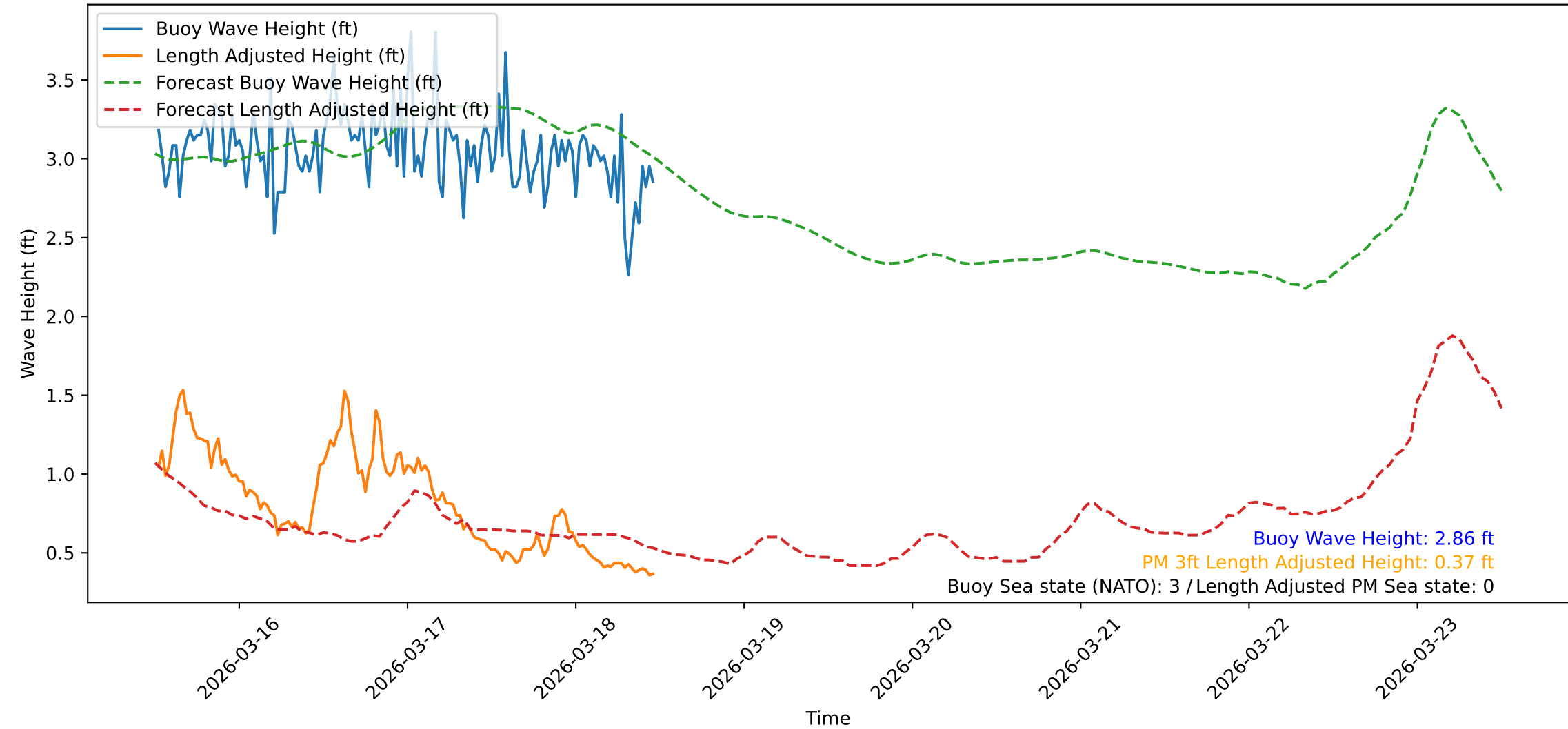
Wave Heights over Time for Red Beach at 2026-03-18 12:00:47
