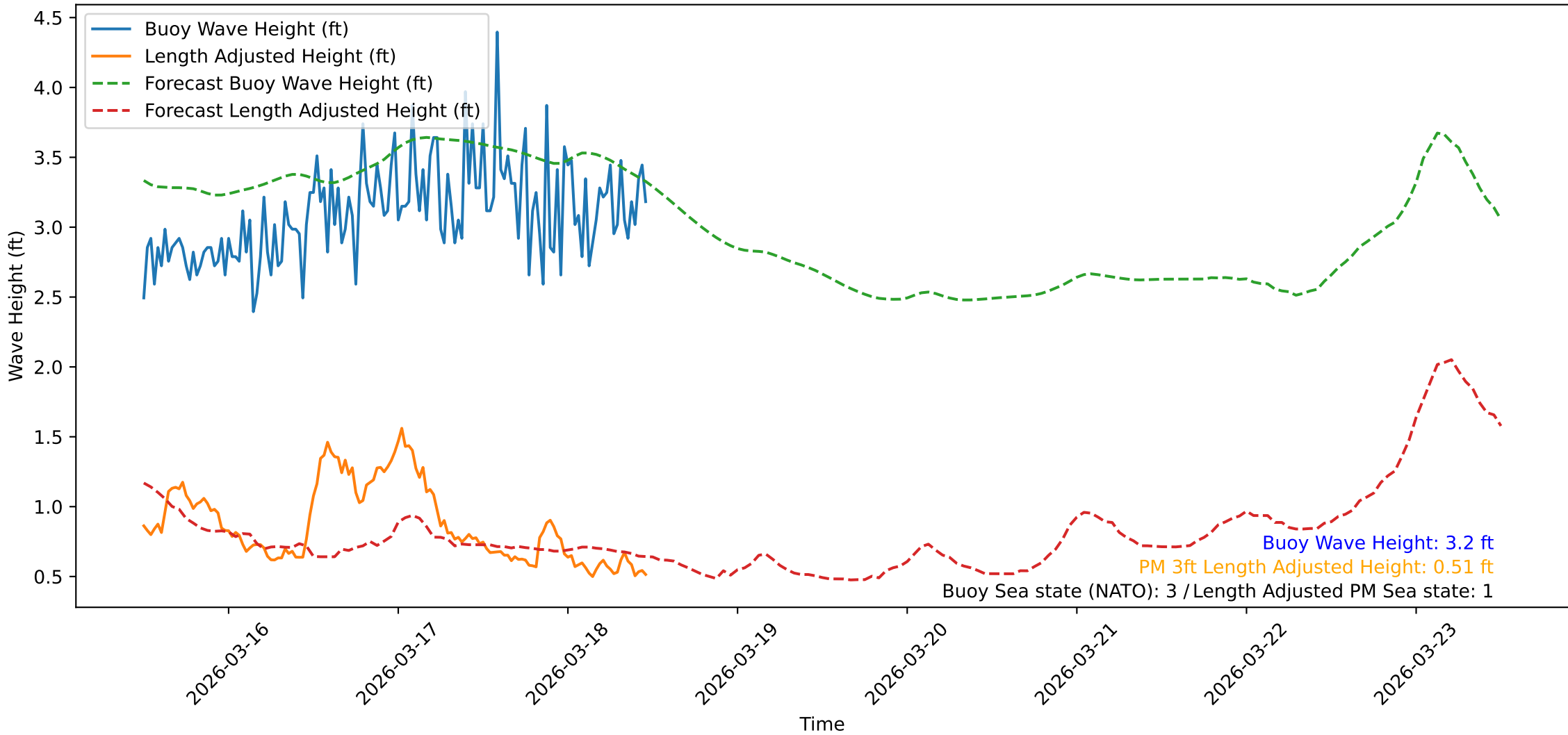
Wave Heights over Time for Oceanside Harbor at 2026-03-18 12:00:31
