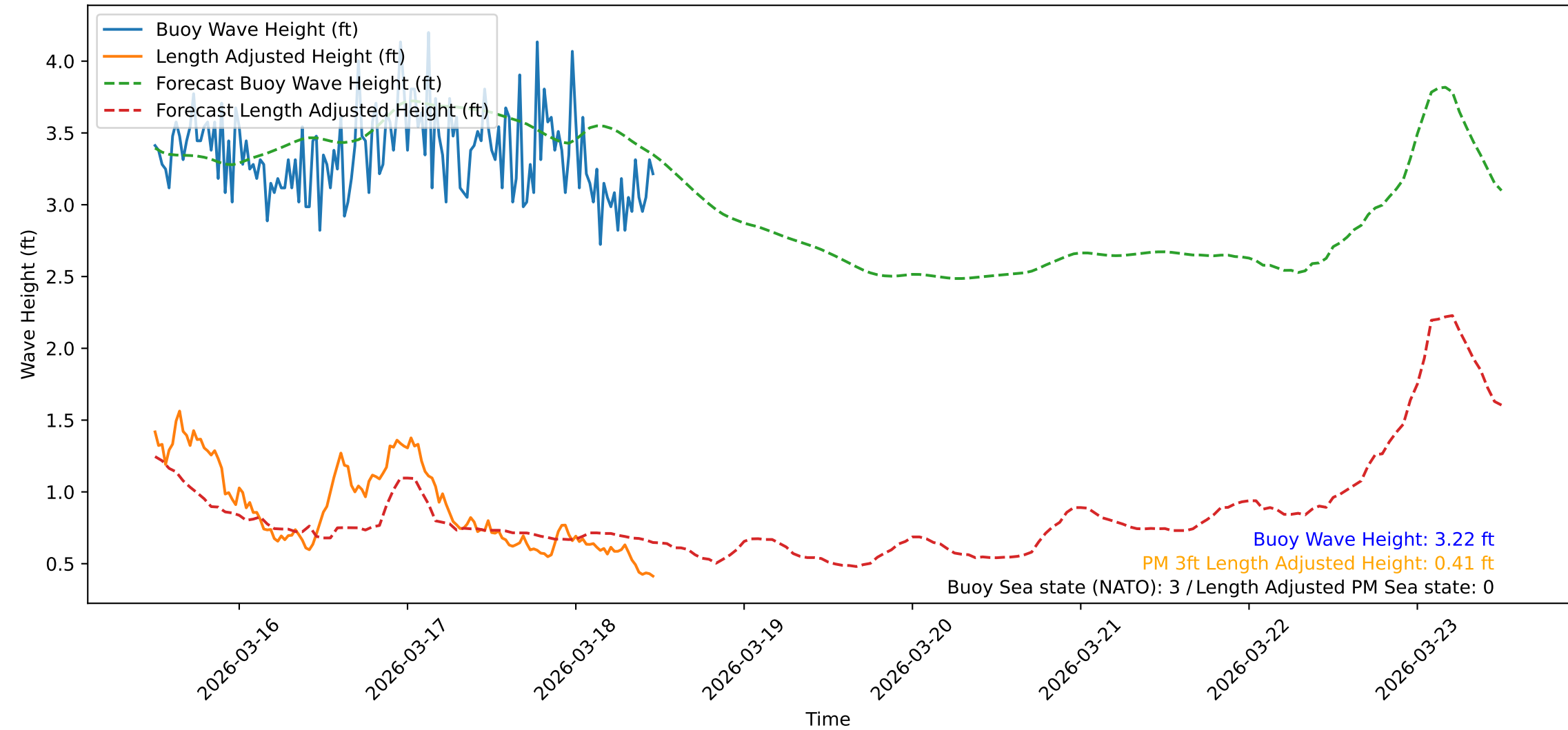
Wave Heights over Time for Green Beach at 2026-03-18 12:01:10
