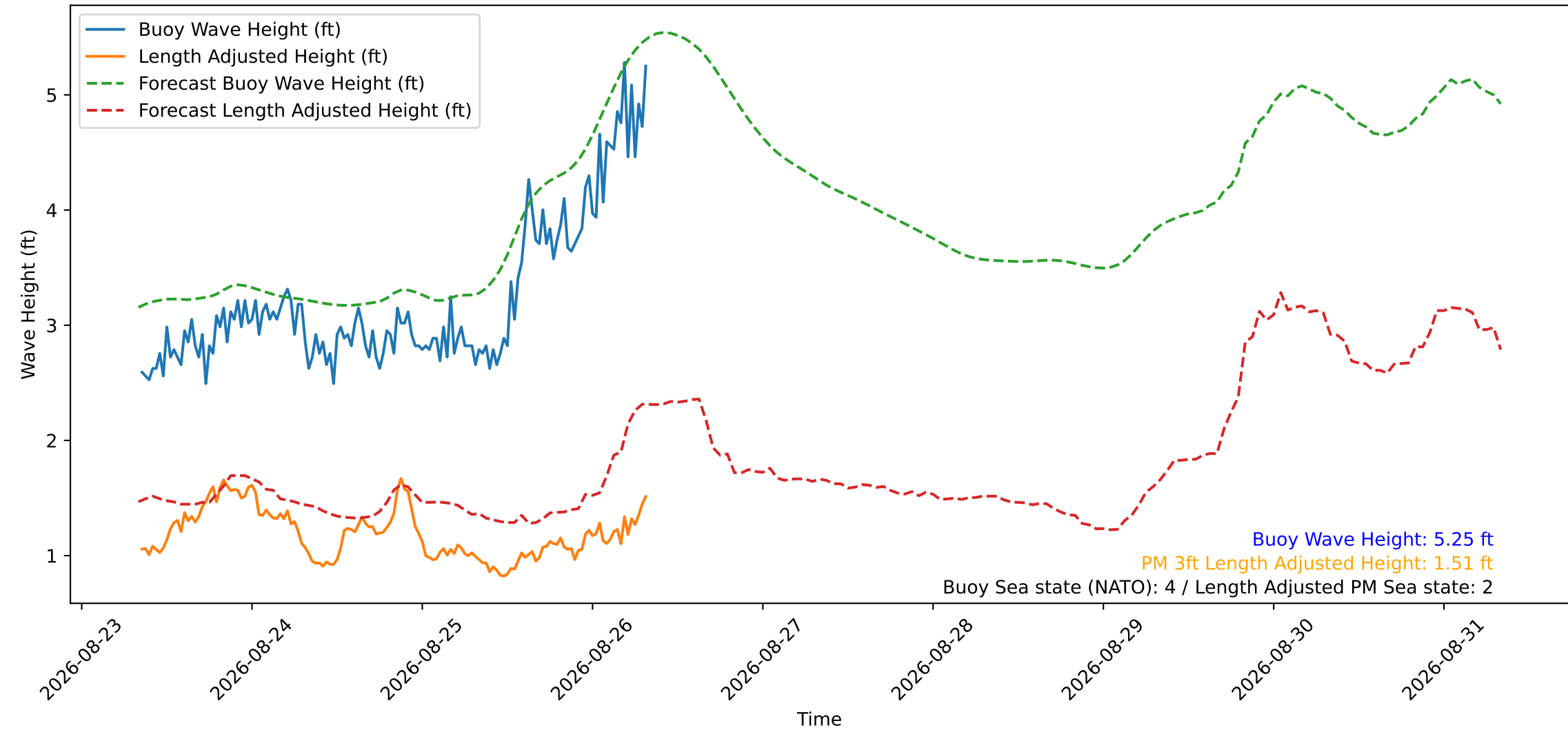
Wave Heights over Time for Green Beach at 2026-08-26 08:21:16
