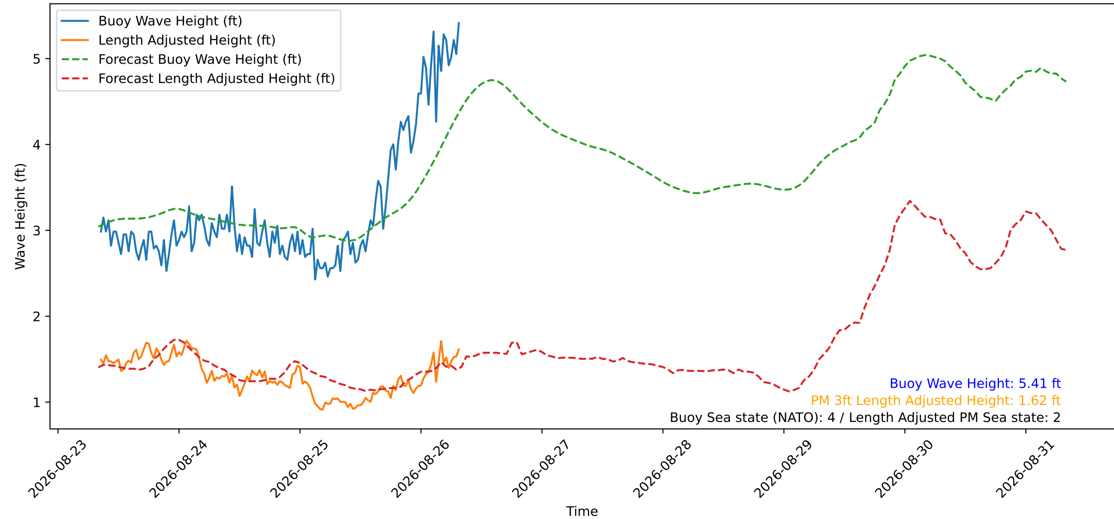
Wave Heights over Time for Oceanside Harbor at 2026-08-26 08:20:31
