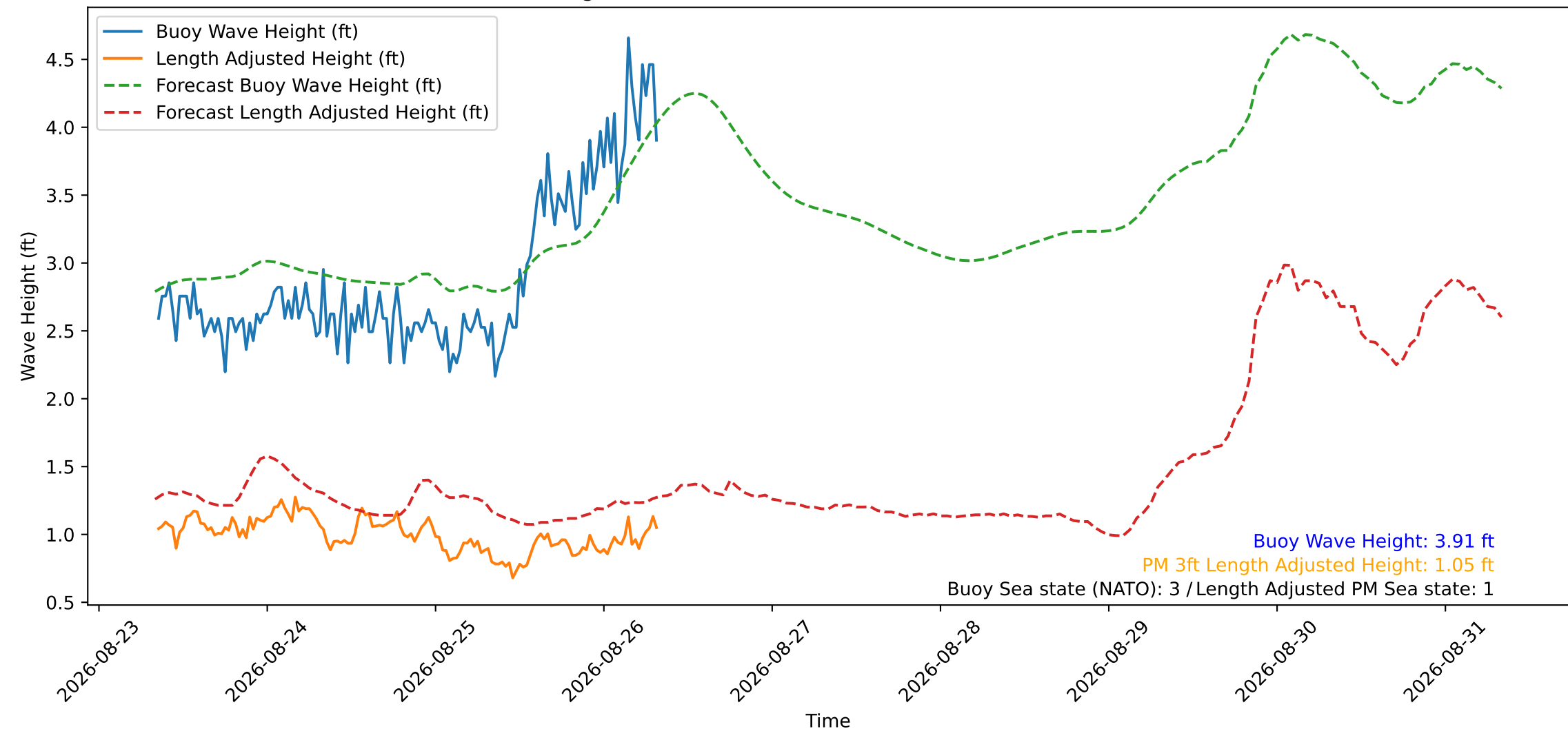
Wave Heights over Time for Red Beach at 2026-08-26 08:20:52
