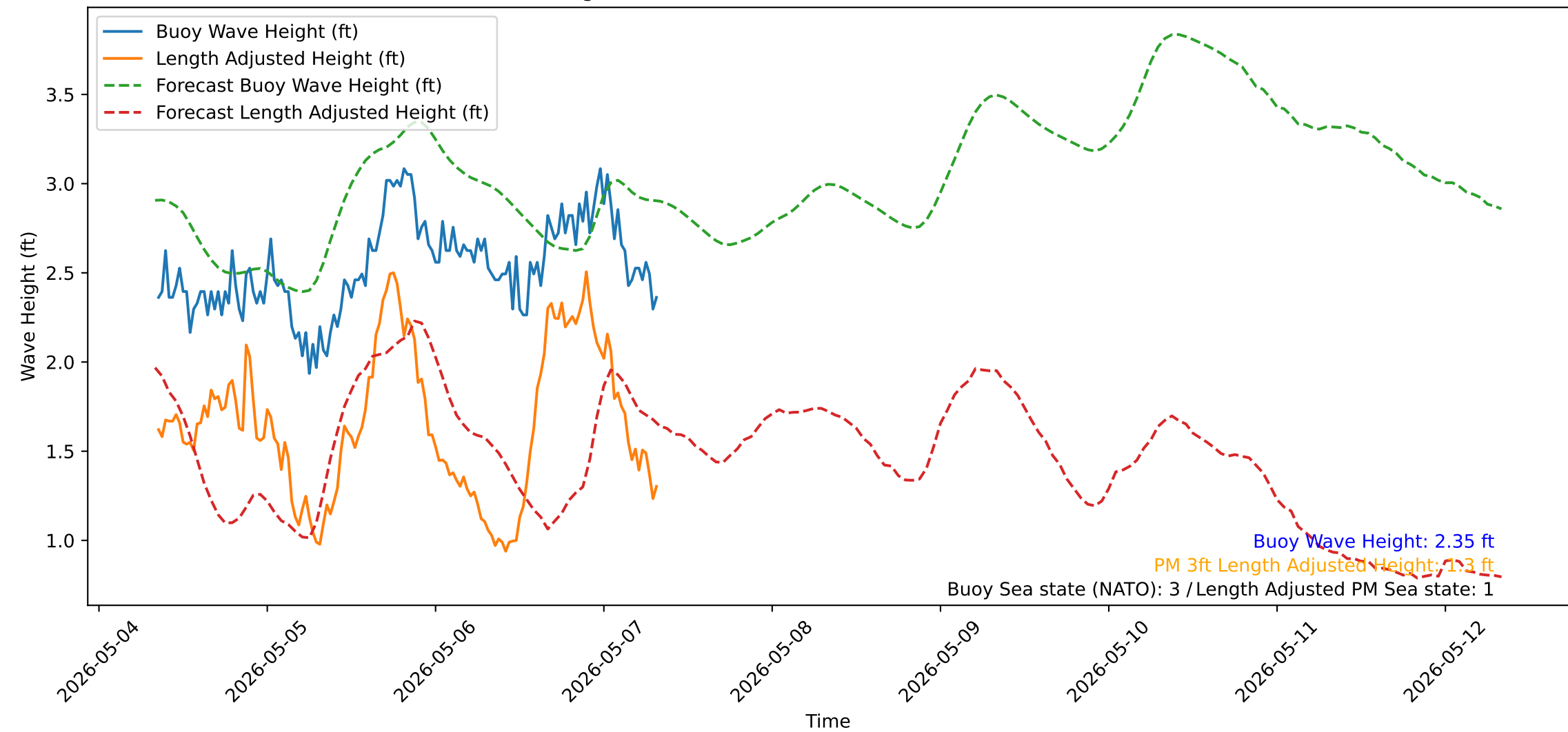
Wave Heights over Time for Red Beach at 2026-05-07 08:20:51
