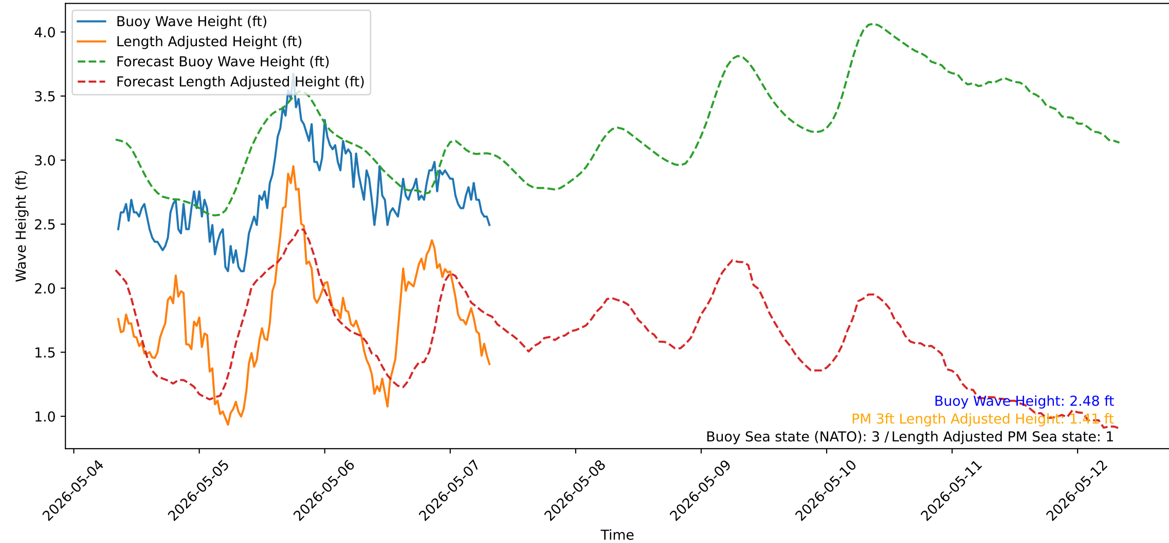
Wave Heights over Time for Green Beach at 2026-05-07 08:21:14
