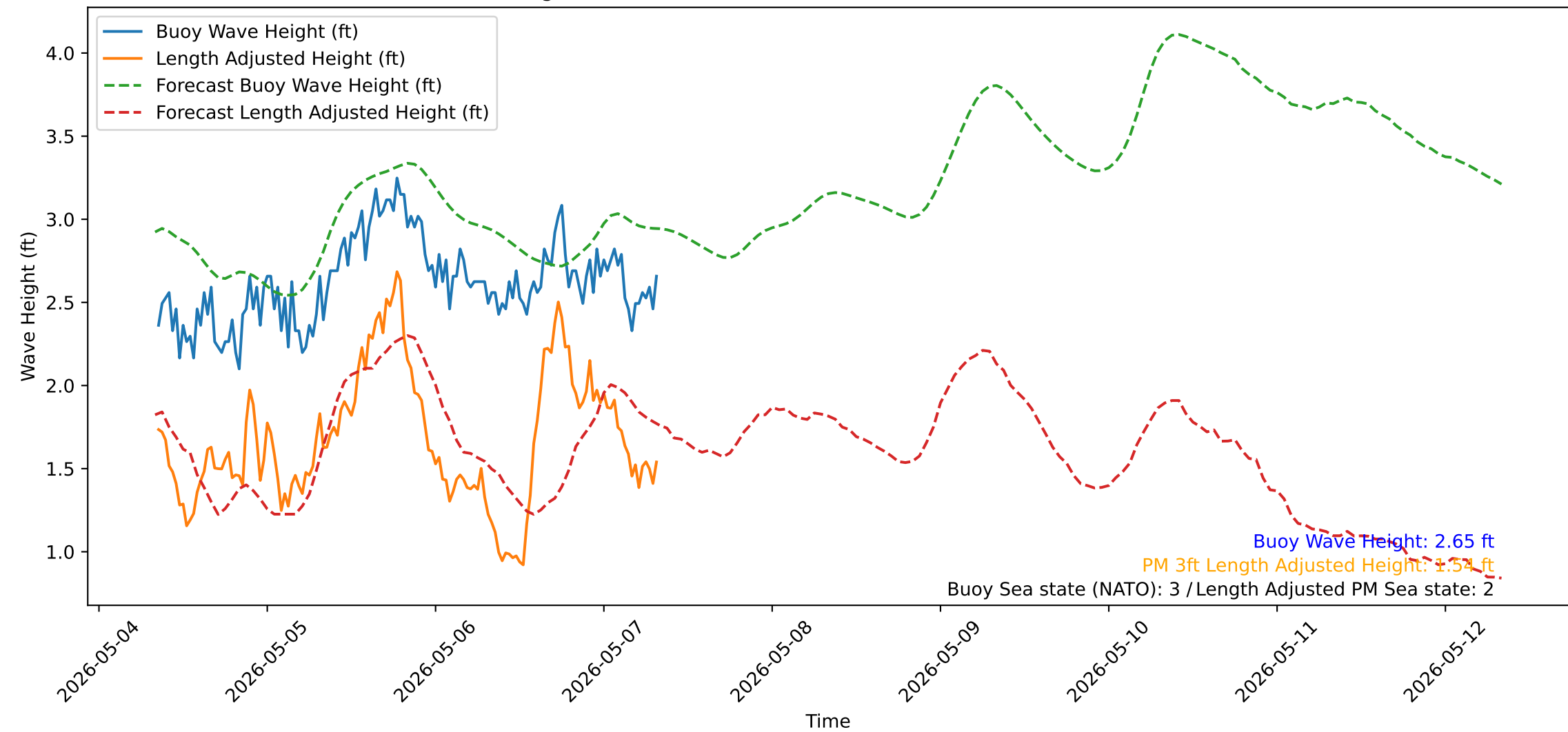
Wave Heights over Time for Oceanside Harbor at 2026-05-07 08:20:30
