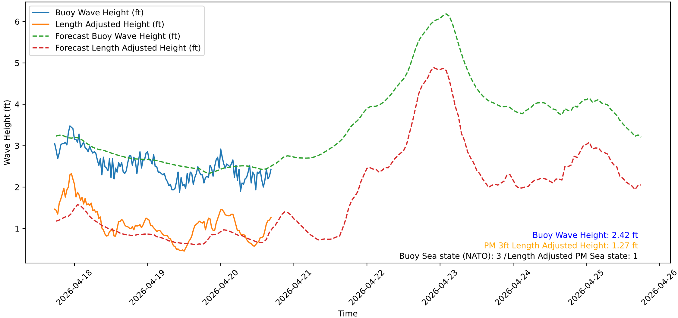
Wave Heights over Time for Green Beach at 2026-04-20 17:31:12
