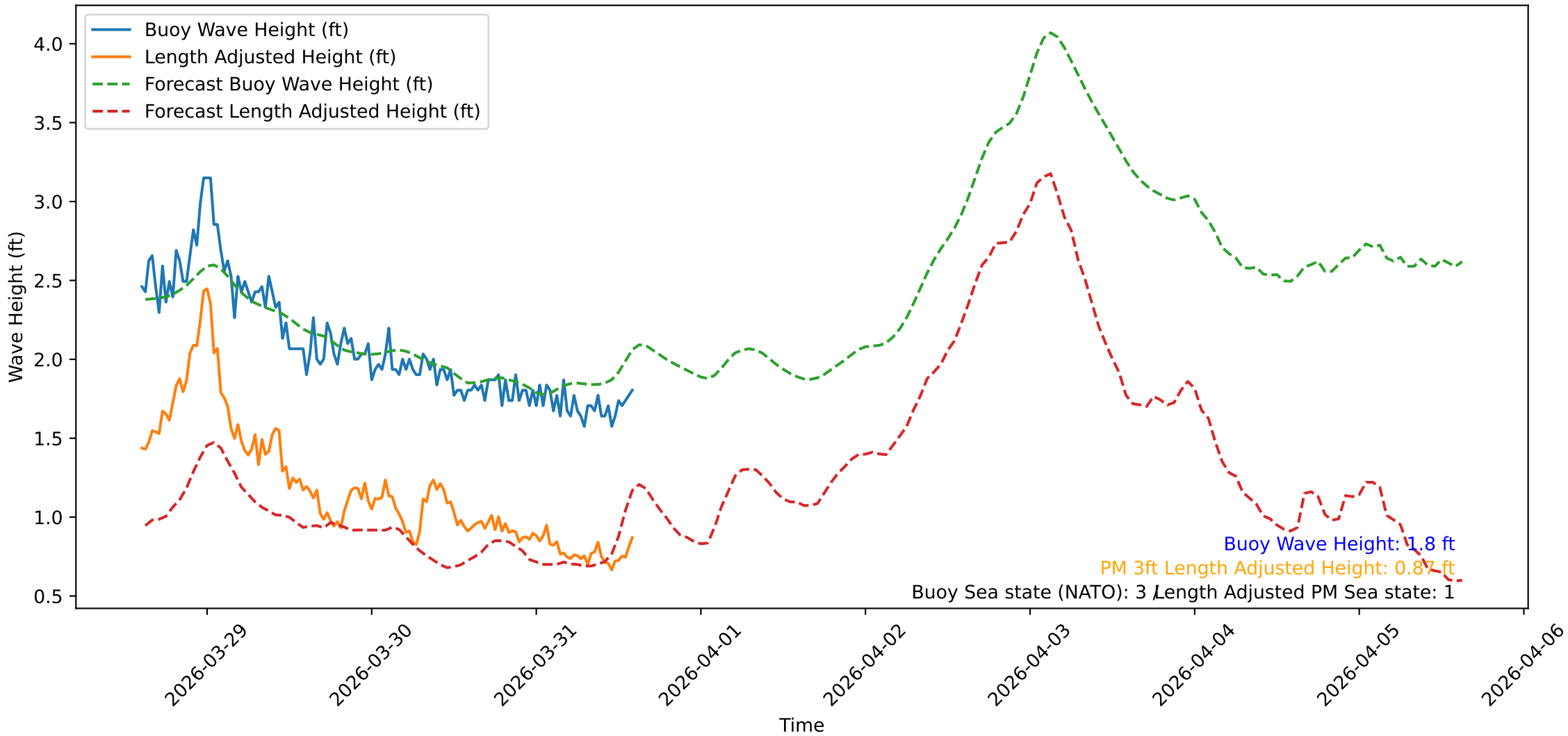
Wave Heights over Time for Oceanside Harbor at 2026-03-31 14:40:31
