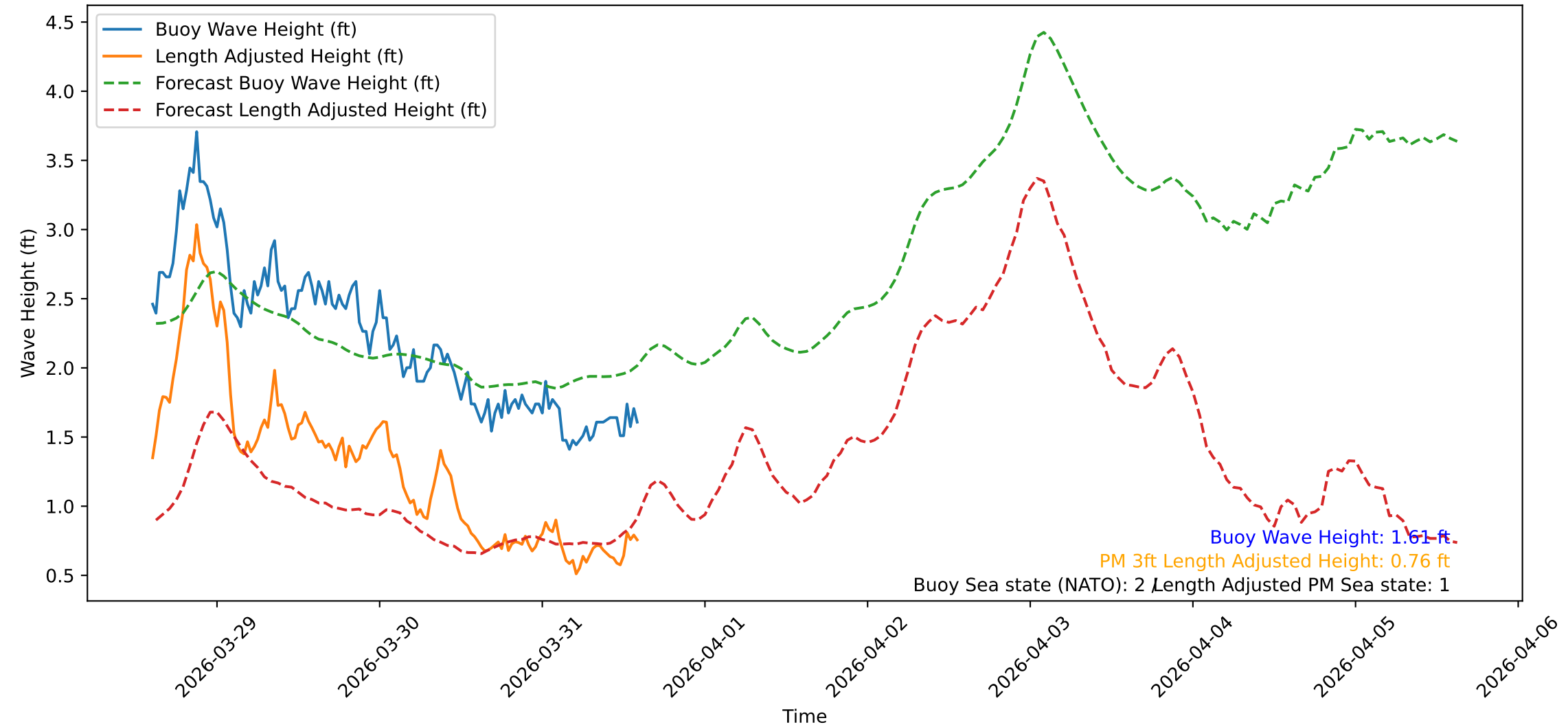
Wave Heights over Time for Green Beach at 2026-03-31 14:41:10
