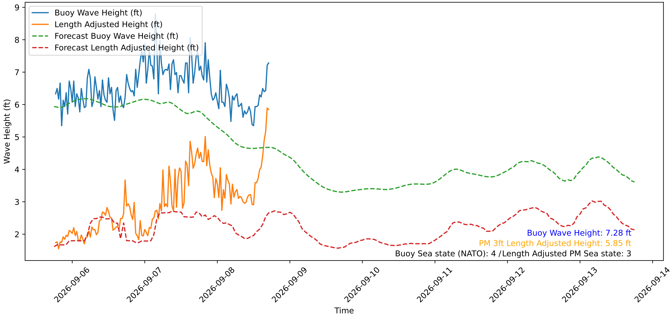
Wave Heights over Time for Green Beach at 2026-09-08 18:01:12
