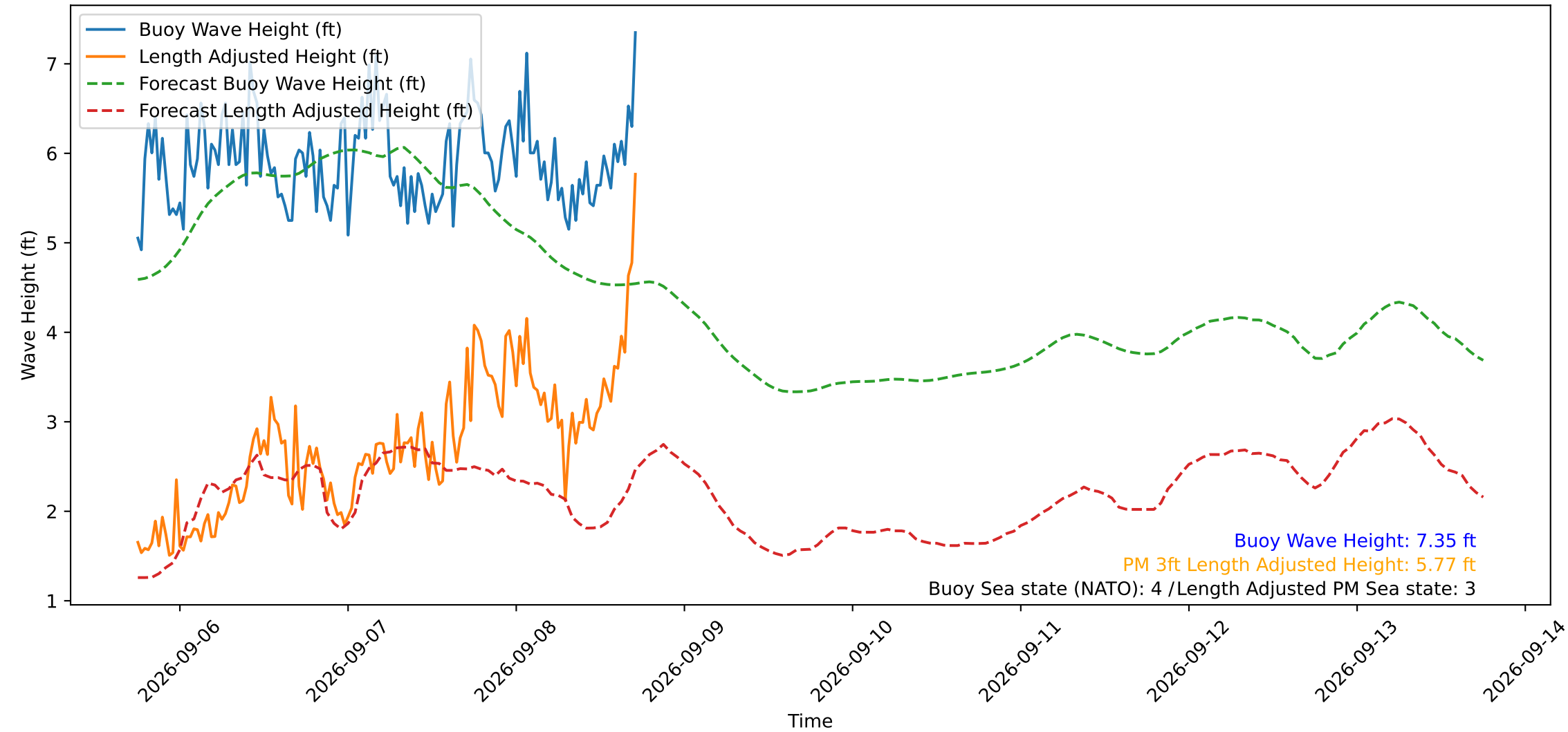
Wave Heights over Time for Oceanside Harbor at 2026-09-08 18:00:30
