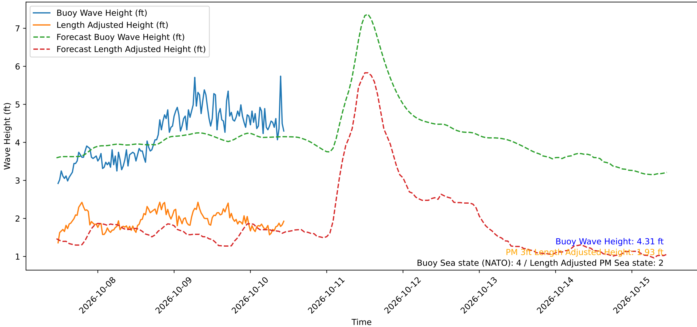
Wave Heights over Time for Red Beach at 2026-10-10 11:10:49
