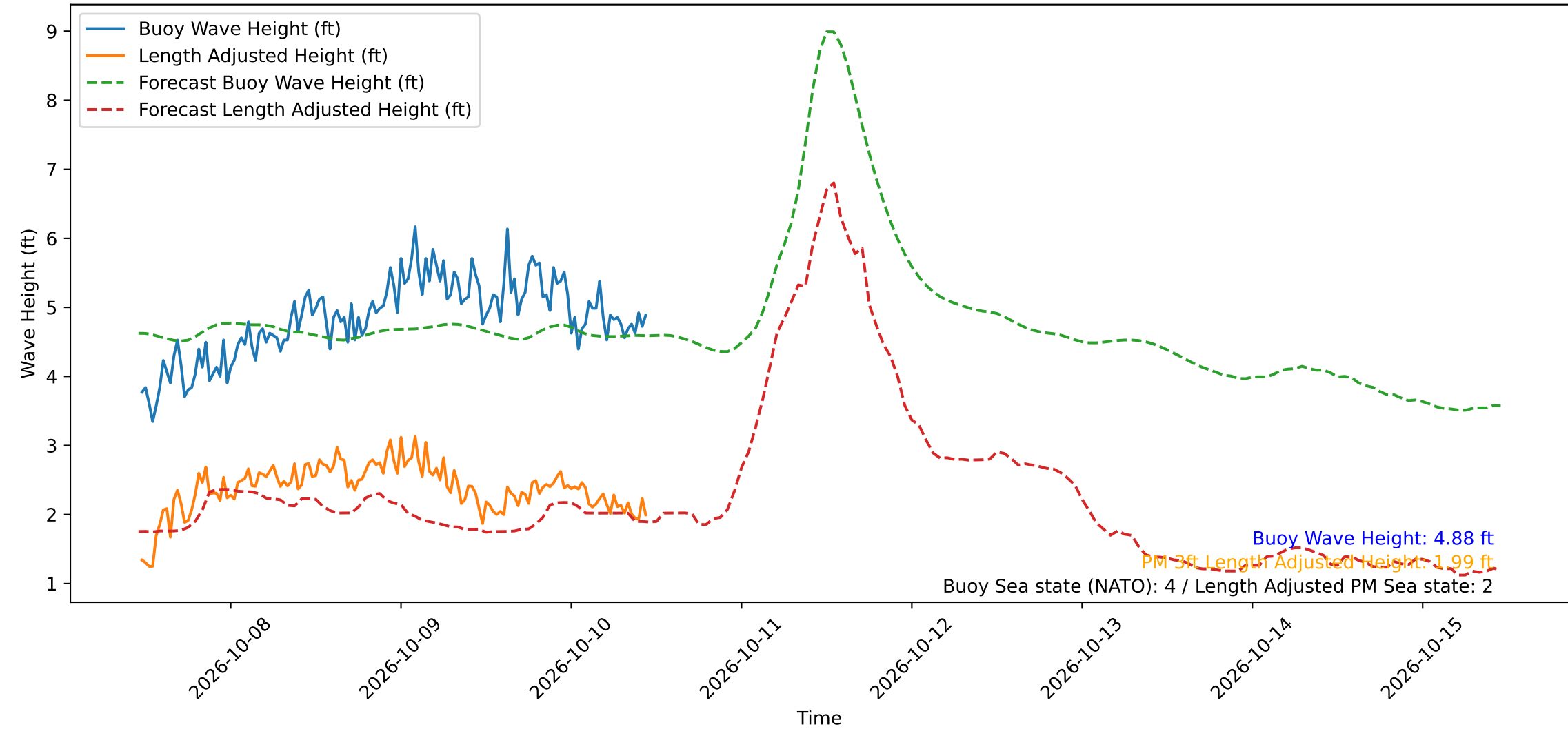
Wave Heights over Time for Green Beach at 2026-10-10 11:11:11
