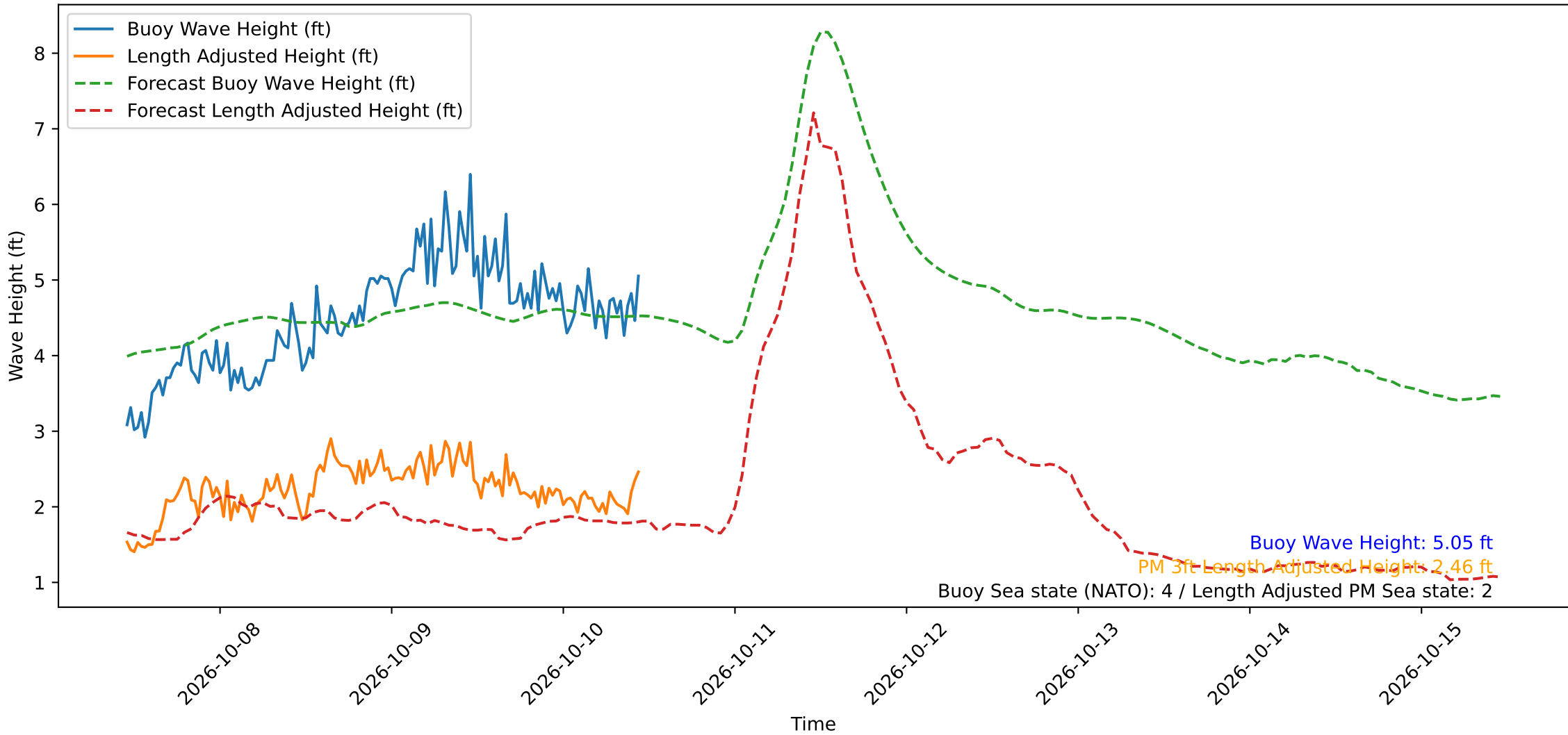
Wave Heights over Time for Oceanside Harbor at 2026-10-10 11:10:29
