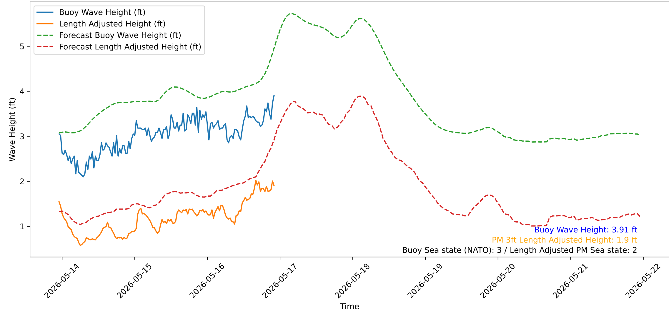
Wave Heights over Time for Green Beach at 2026-05-16 22:51:15
