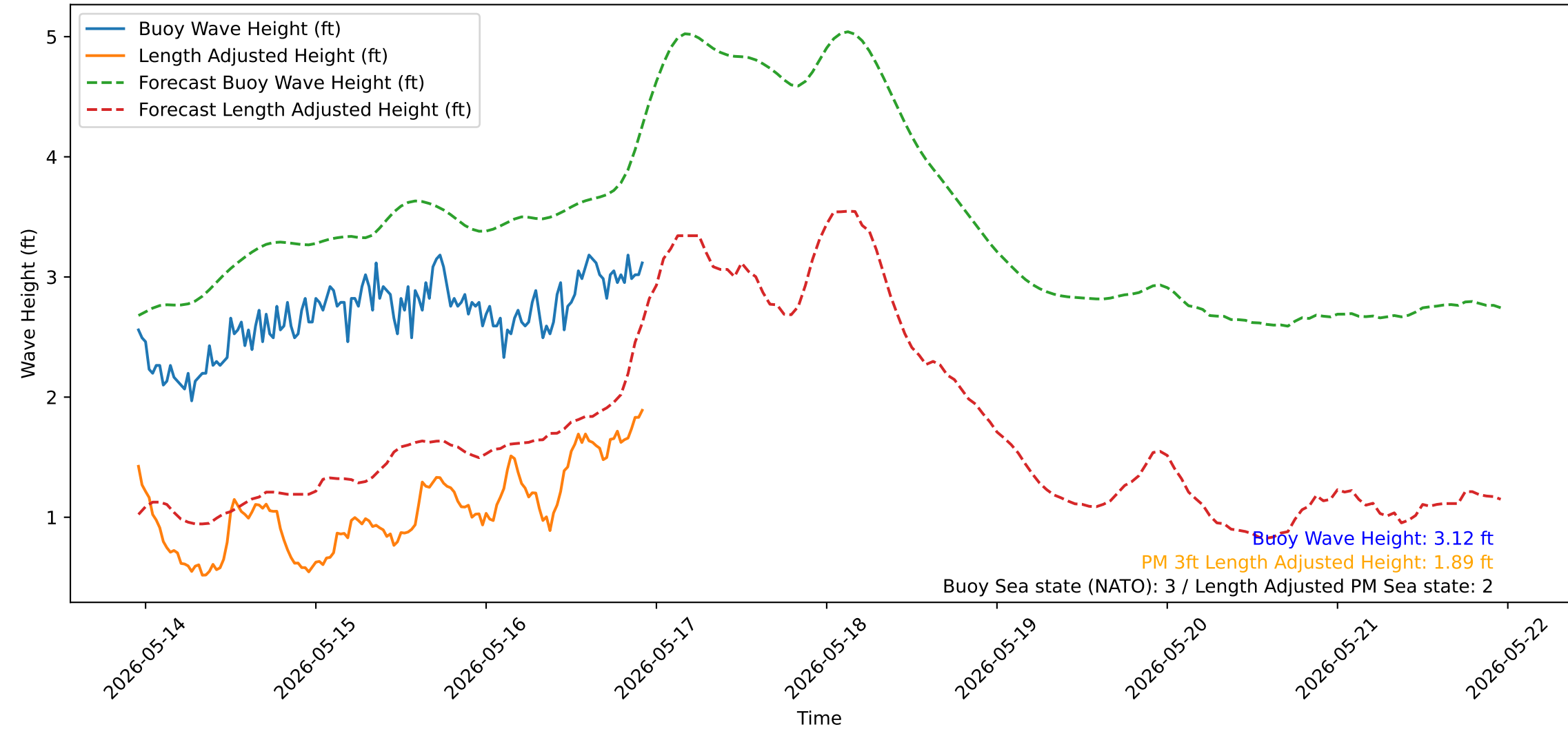
Wave Heights over Time for Red Beach at 2026-05-16 22:50:52
