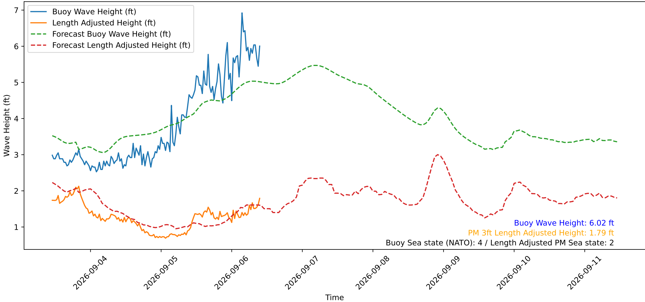
Wave Heights over Time for Red Beach at 2026-09-06 10:30:49
