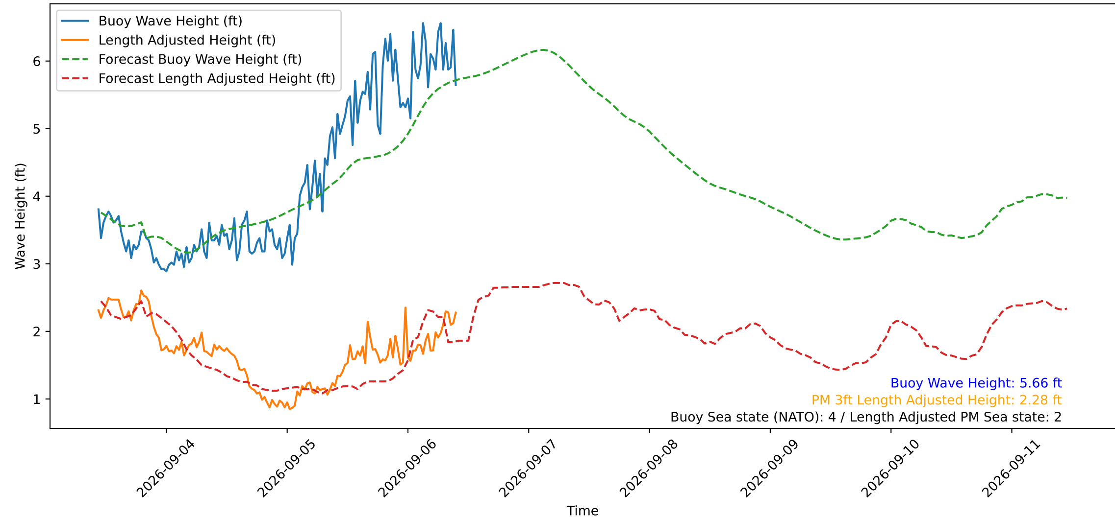
Wave Heights over Time for Oceanside Harbor at 2026-09-06 10:30:29
