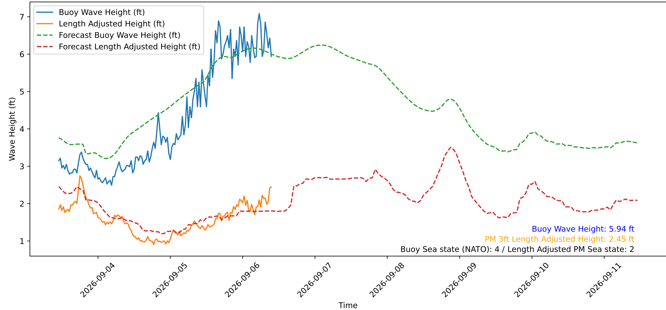
Wave Heights over Time for Green Beach at 2026-09-06 10:31:11
