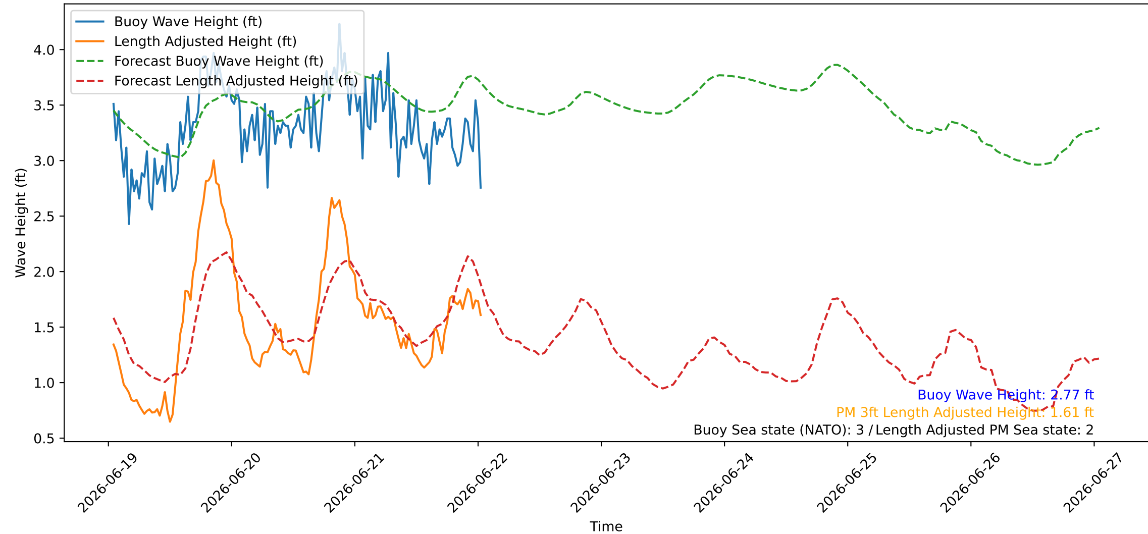
Wave Heights over Time for Green Beach at 2026-06-22 01:11:08
