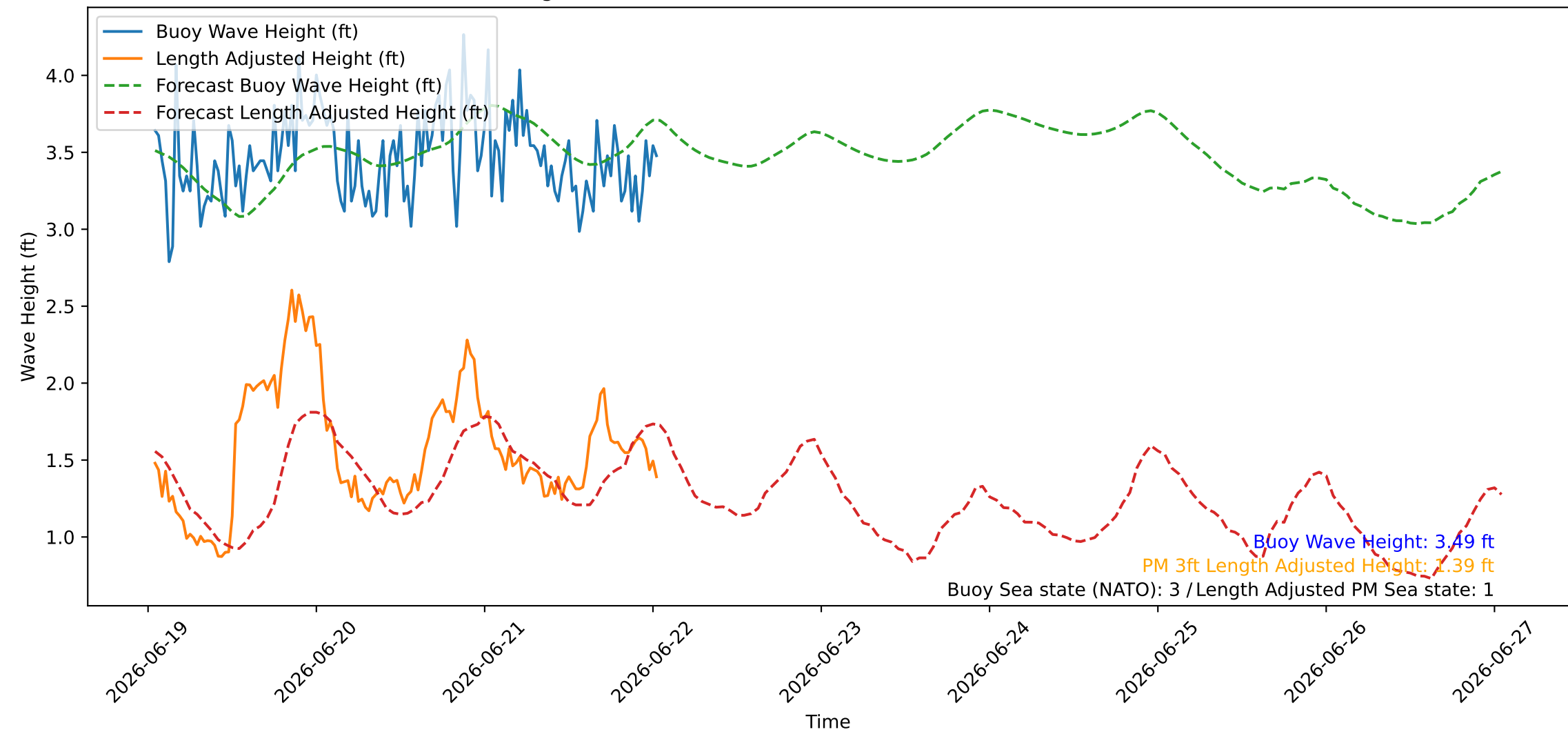
Wave Heights over Time for Oceanside Harbor at 2026-06-22 01:10:26
