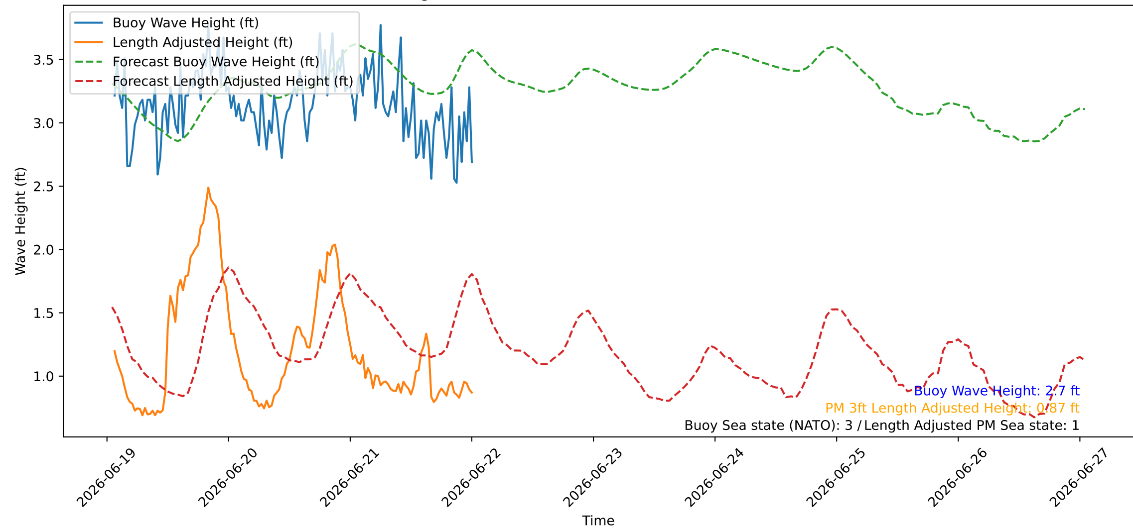
Wave Heights over Time for Red Beach at 2026-06-22 01:10:45
