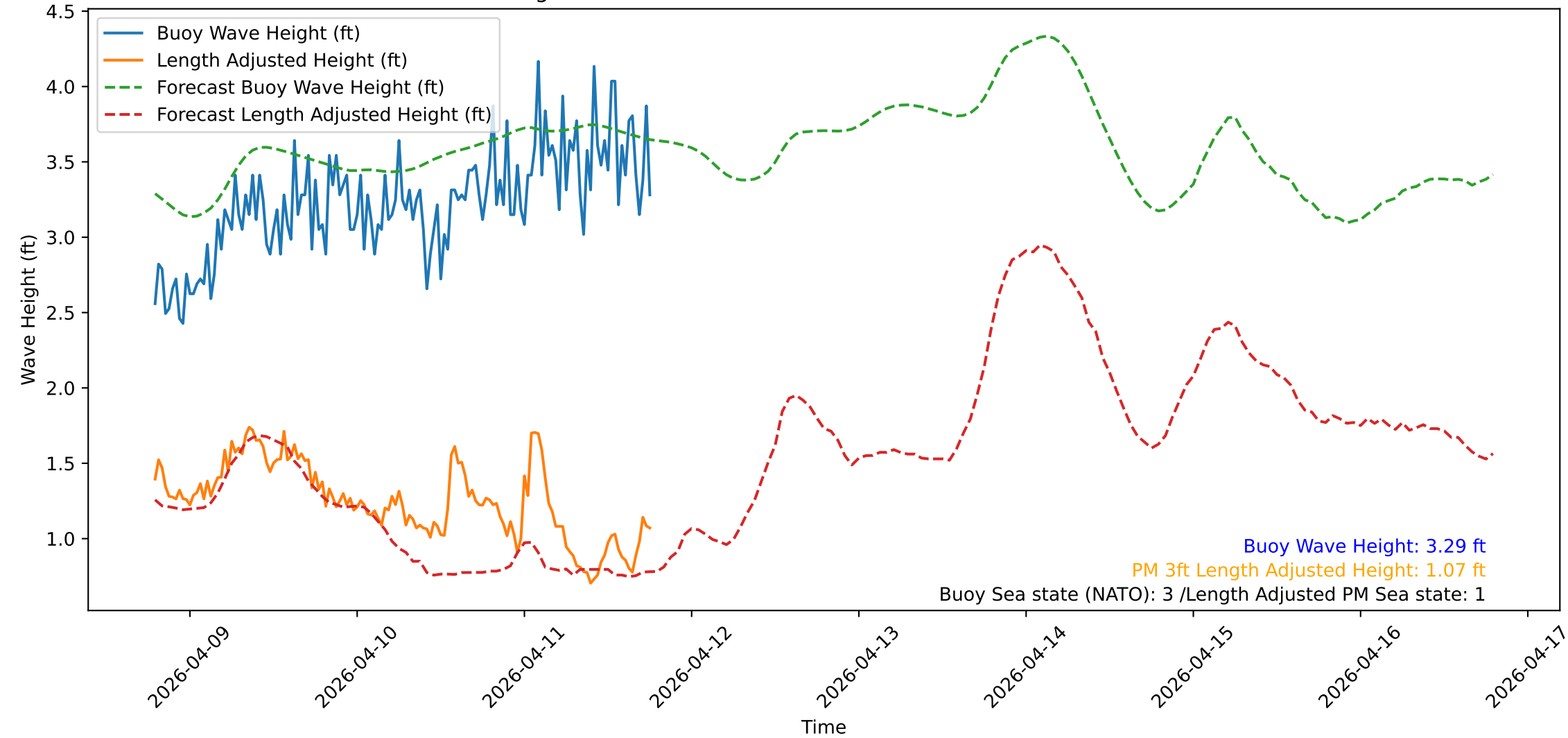
Wave Heights over Time for Oceanside Harbor at 2026-04-11 18:50:31
