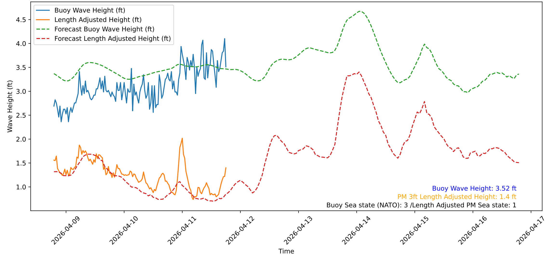
Wave Heights over Time for Green Beach at 2026-04-11 18:51:14
