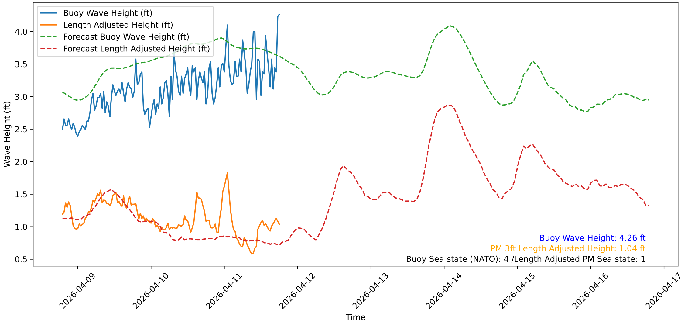
Wave Heights over Time for Red Beach at 2026-04-11 18:50:51
