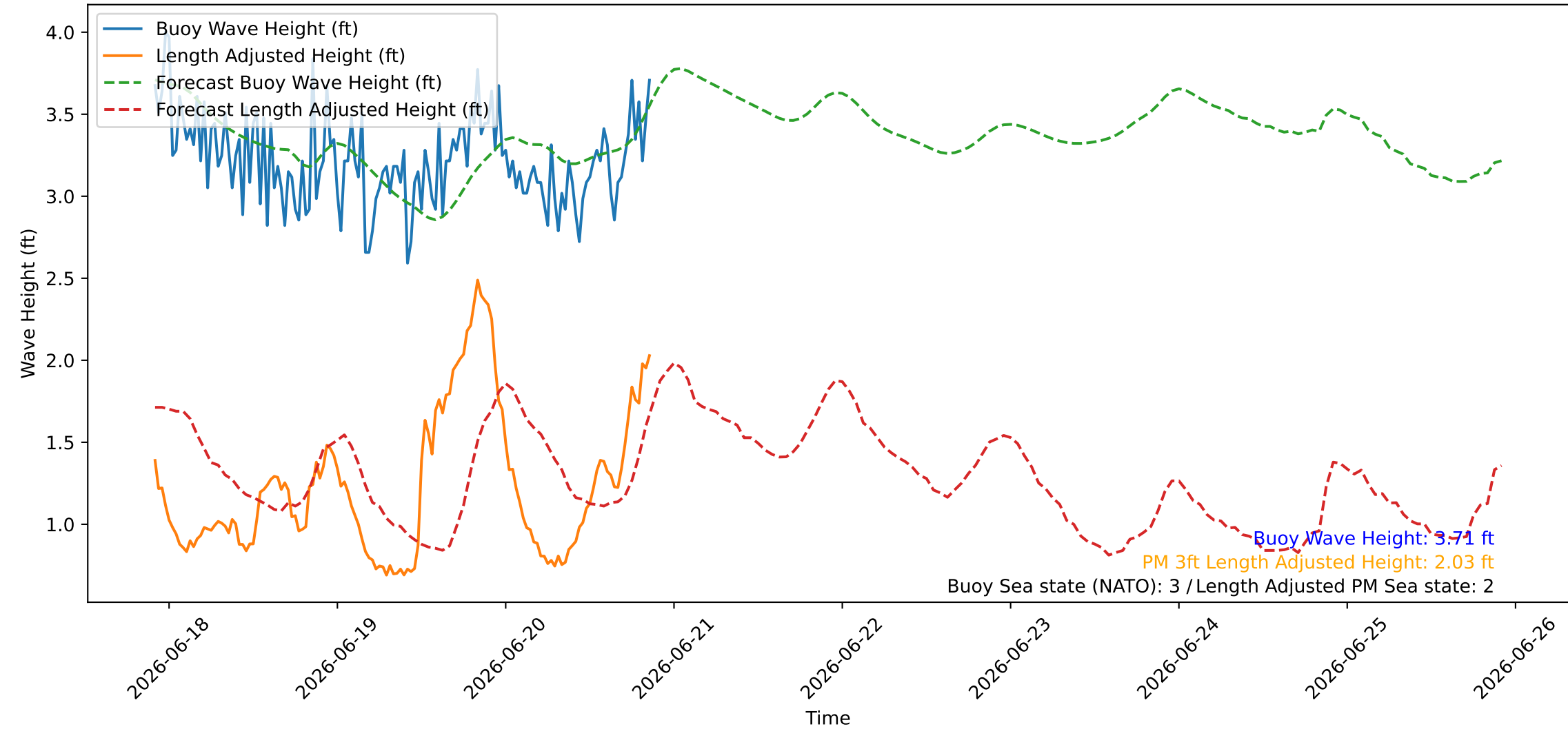
Wave Heights over Time for Red Beach at 2026-06-20 21:30:45
