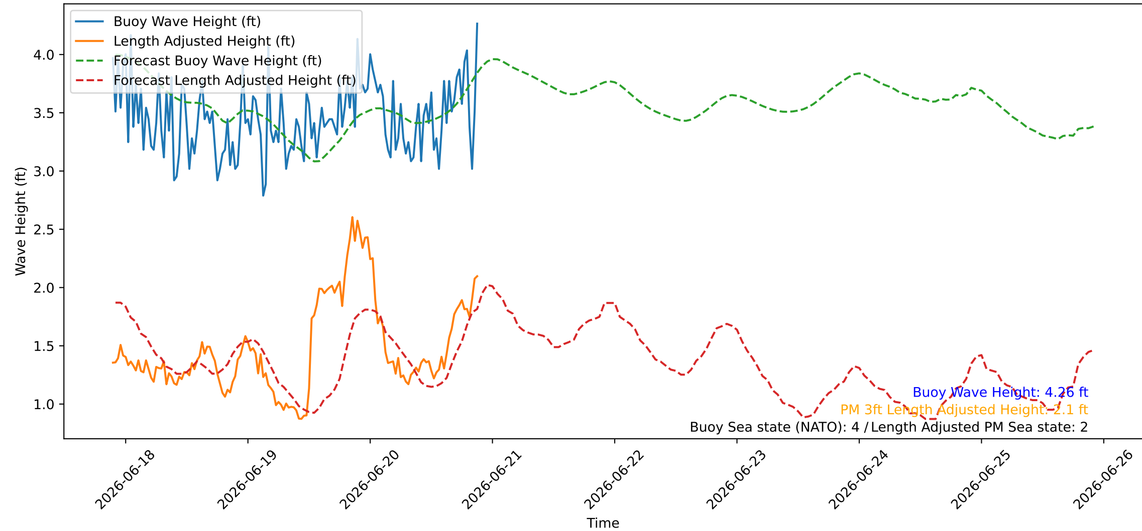
Wave Heights over Time for Oceanside Harbor at 2026-06-20 21:30:26
