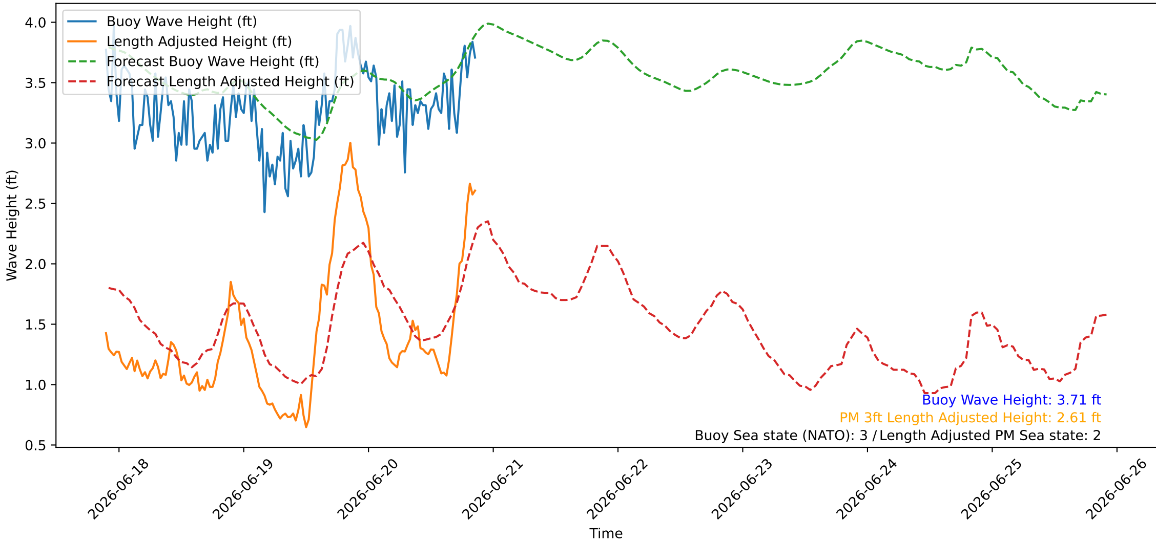
Wave Heights over Time for Green Beach at 2026-06-20 21:31:08
