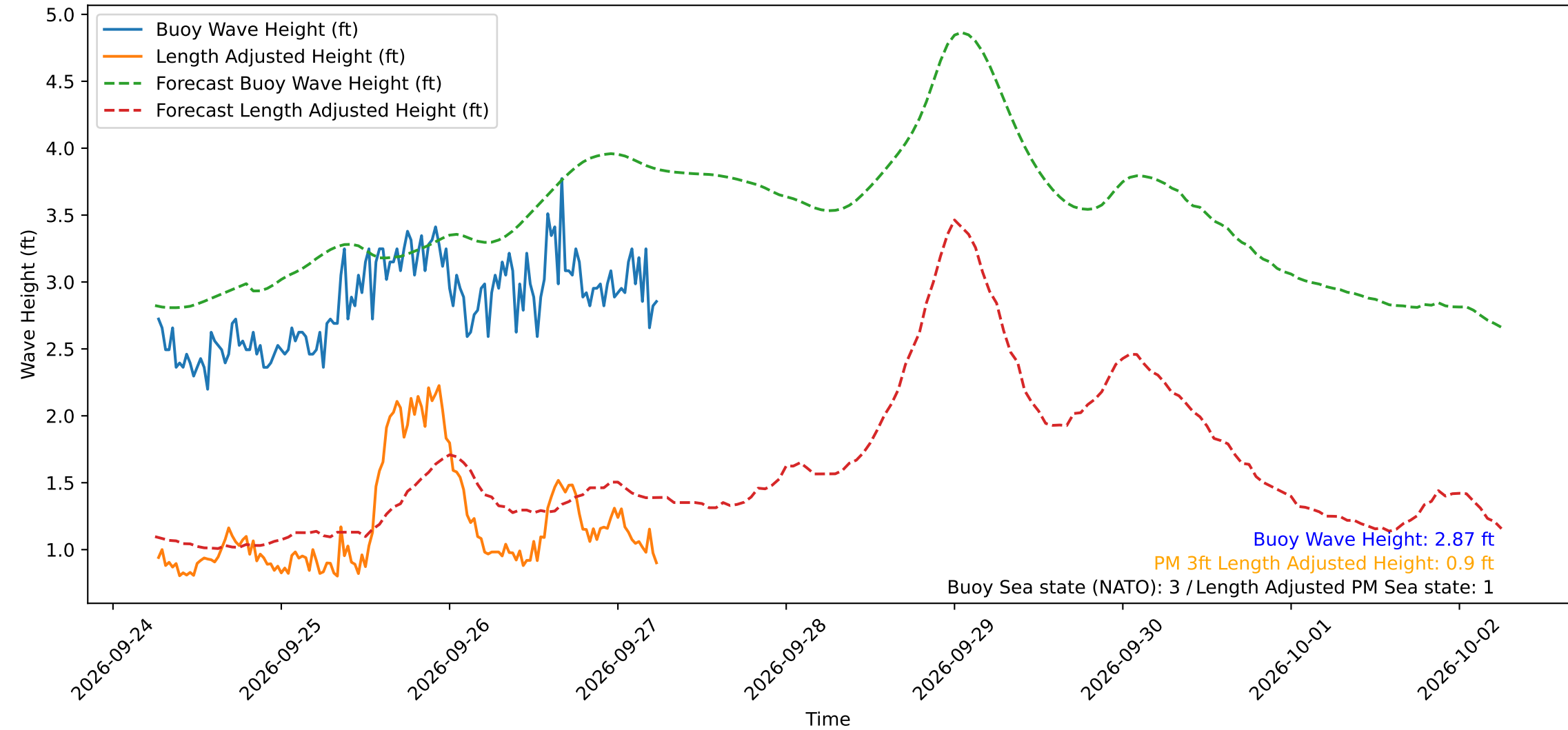
Wave Heights over Time for Oceanside Harbor at 2026-09-27 06:20:29
