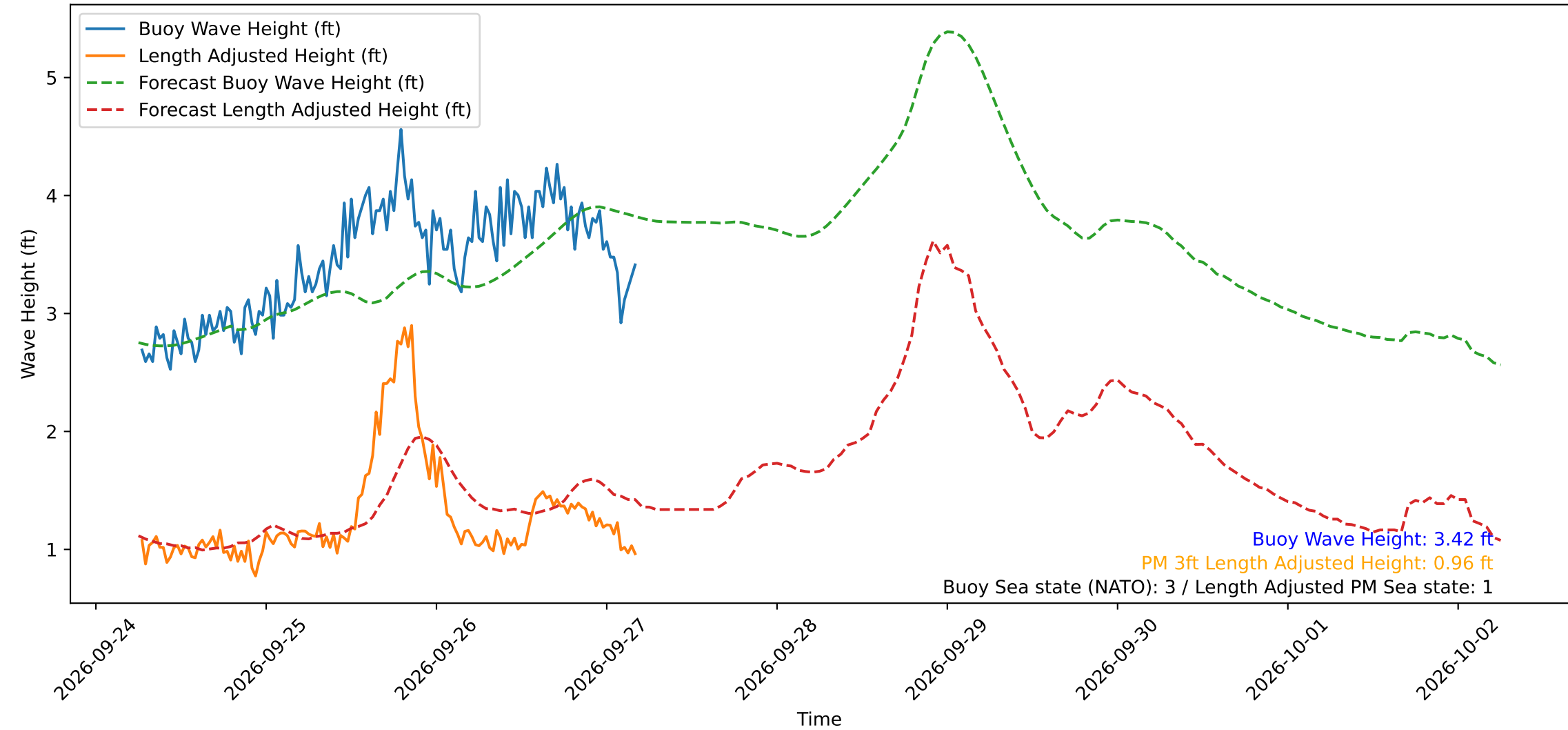
Wave Heights over Time for Green Beach at 2026-09-27 06:21:14
