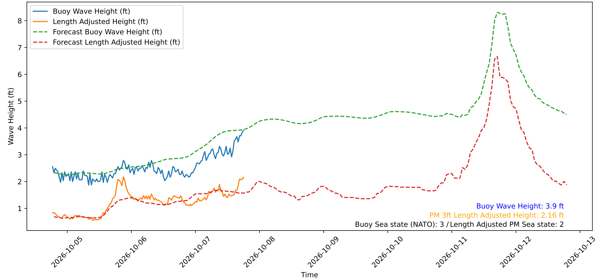
Wave Heights over Time for Oceanside Harbor at 2026-10-07 18:40:30
