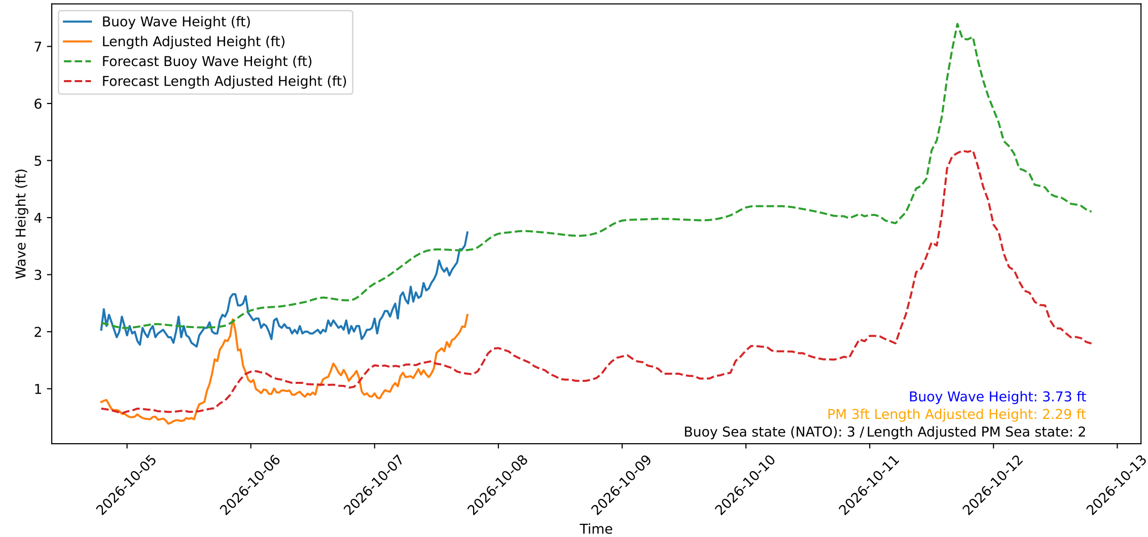
Wave Heights over Time for Red Beach at 2026-10-07 18:40:49
