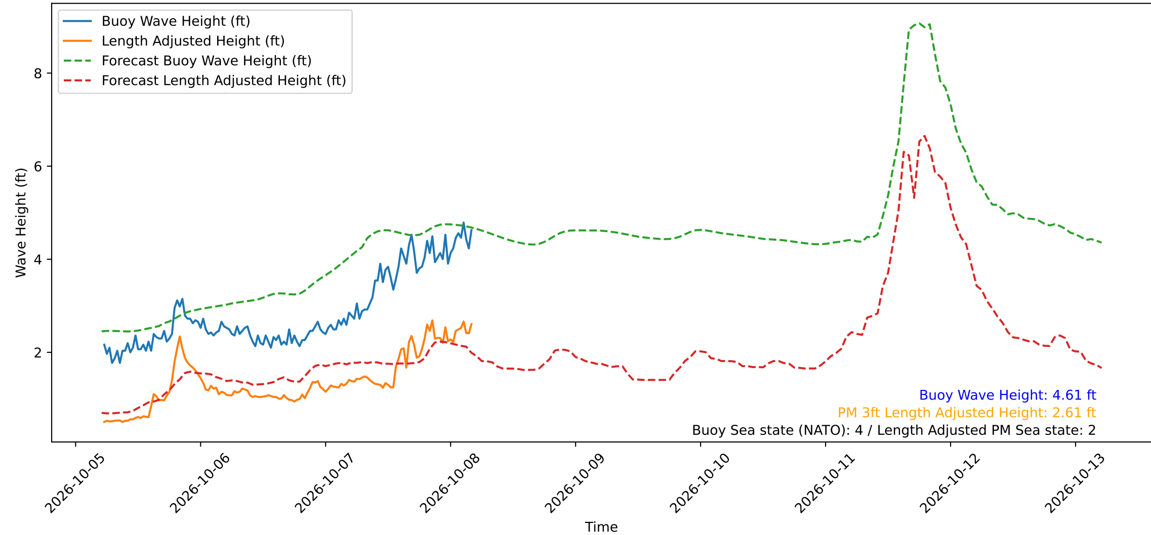
Wave Heights over Time for Green Beach at 2026-10-08 05:21:13
