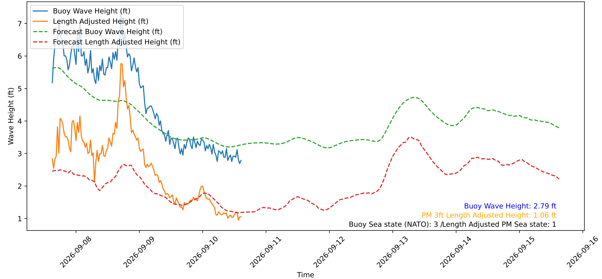
Wave Heights over Time for Oceanside Harbor at 2026-09-10 15:00:30
