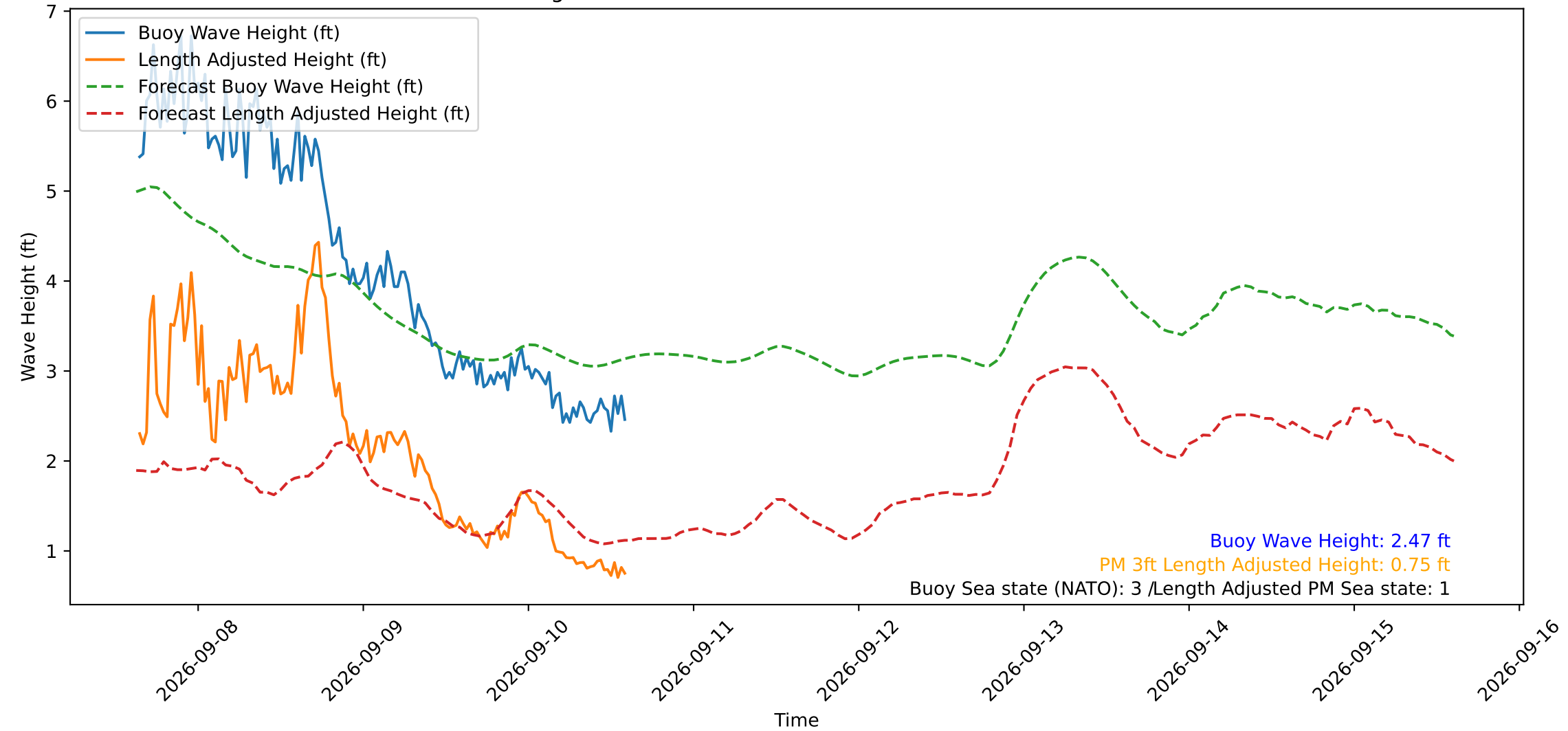
Wave Heights over Time for Red Beach at 2026-09-10 15:00:49
