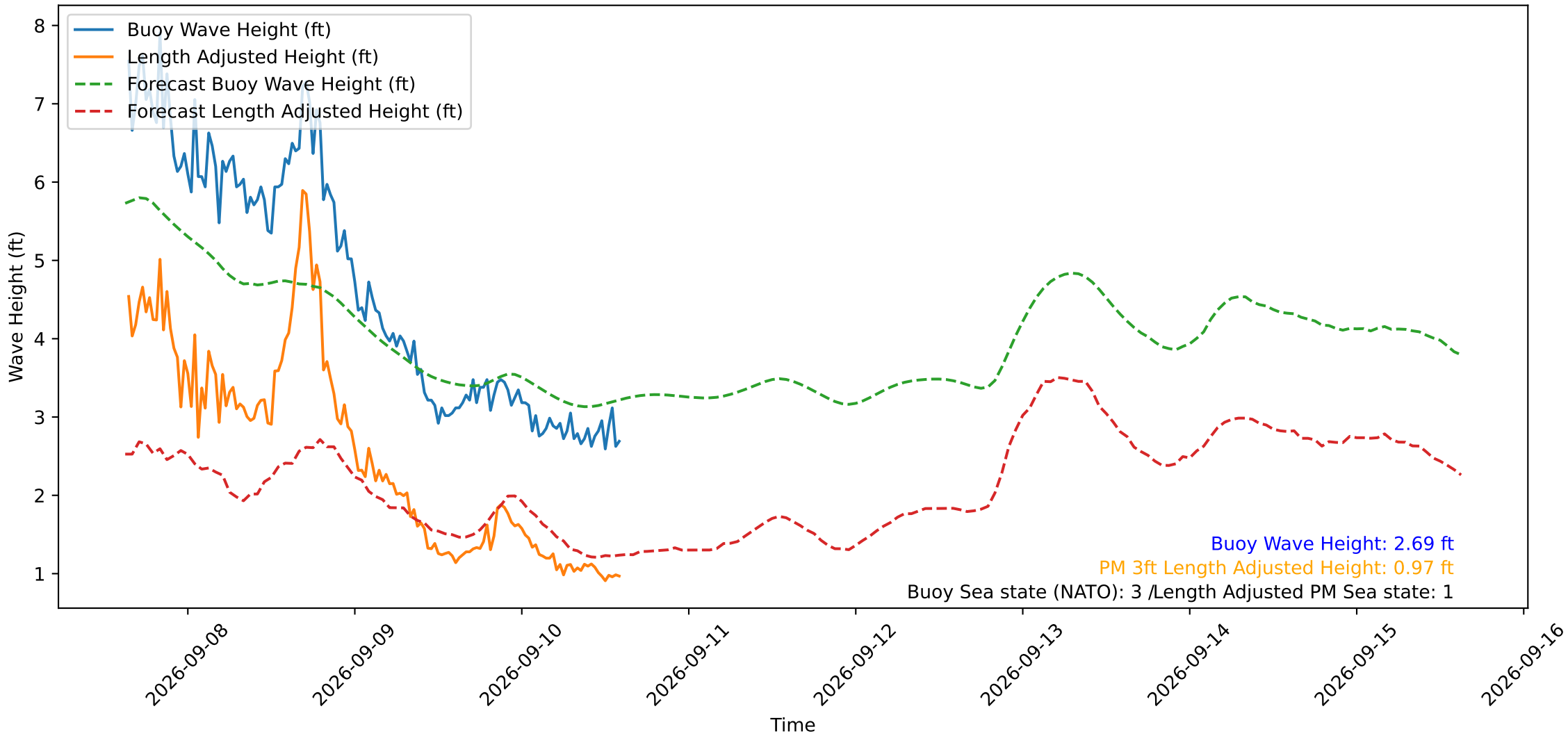
Wave Heights over Time for Green Beach at 2026-09-10 15:01:12
