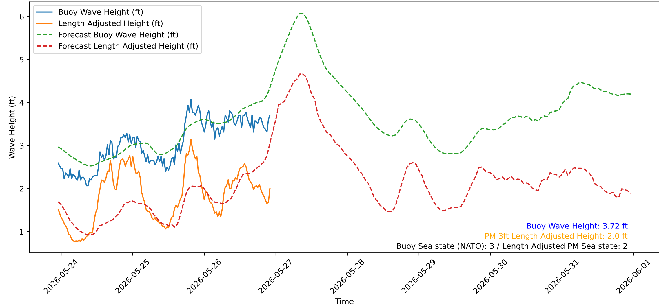
Wave Heights over Time for Green Beach at 2026-05-26 22:51:09
