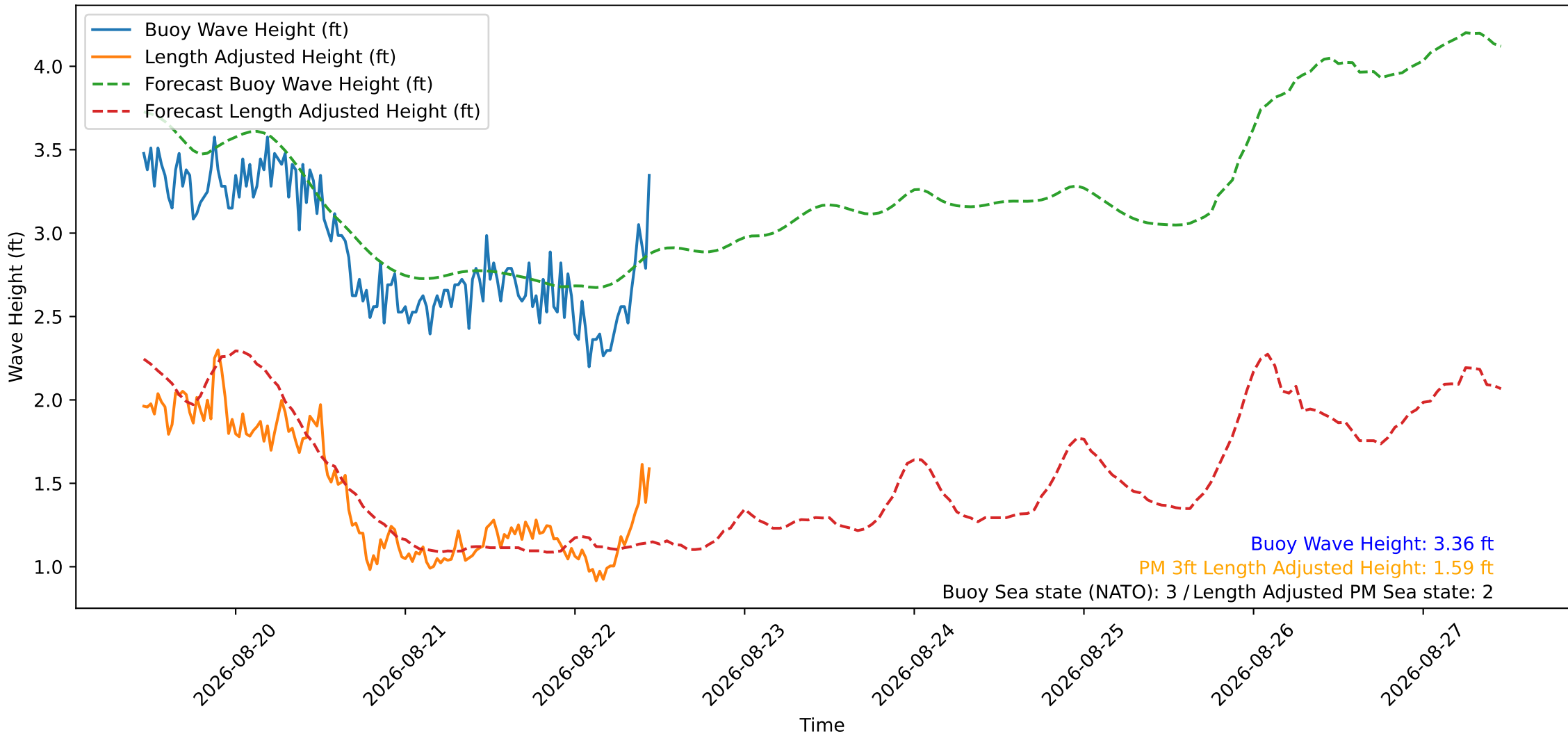
Wave Heights over Time for Oceanside Harbor at 2026-08-22 11:00:29
