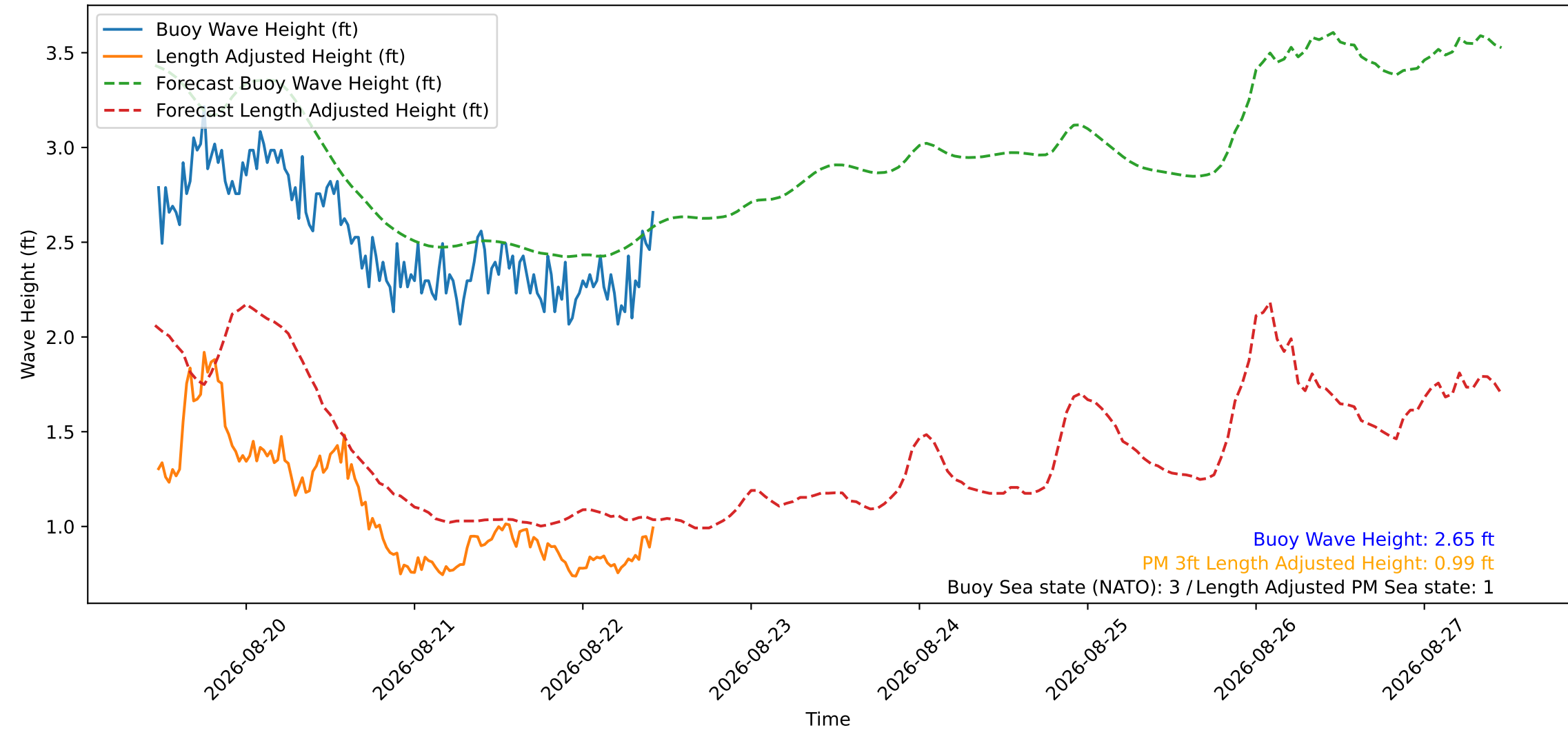
Wave Heights over Time for Red Beach at 2026-08-22 11:00:49
