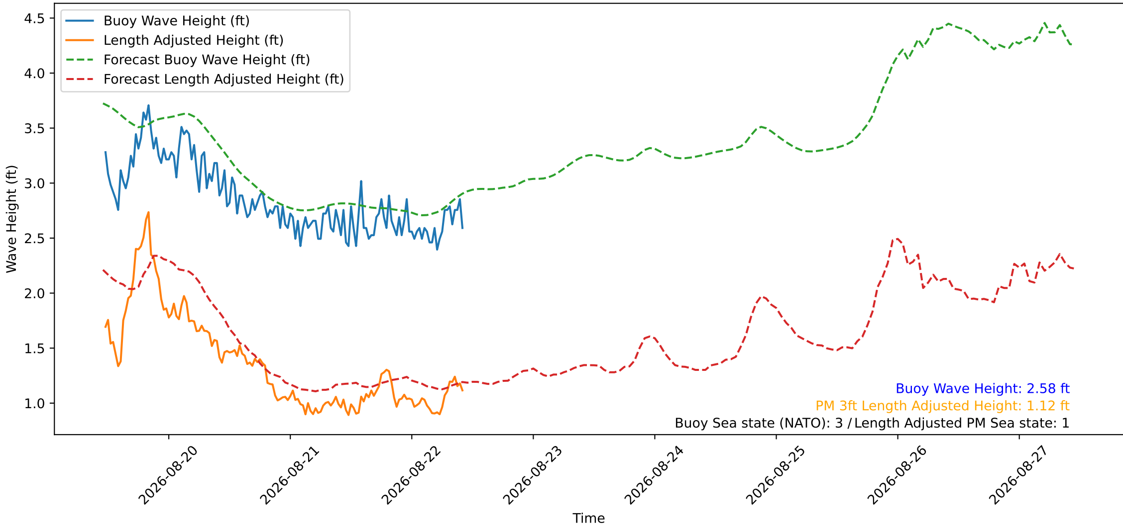
Wave Heights over Time for Green Beach at 2026-08-22 11:01:12
