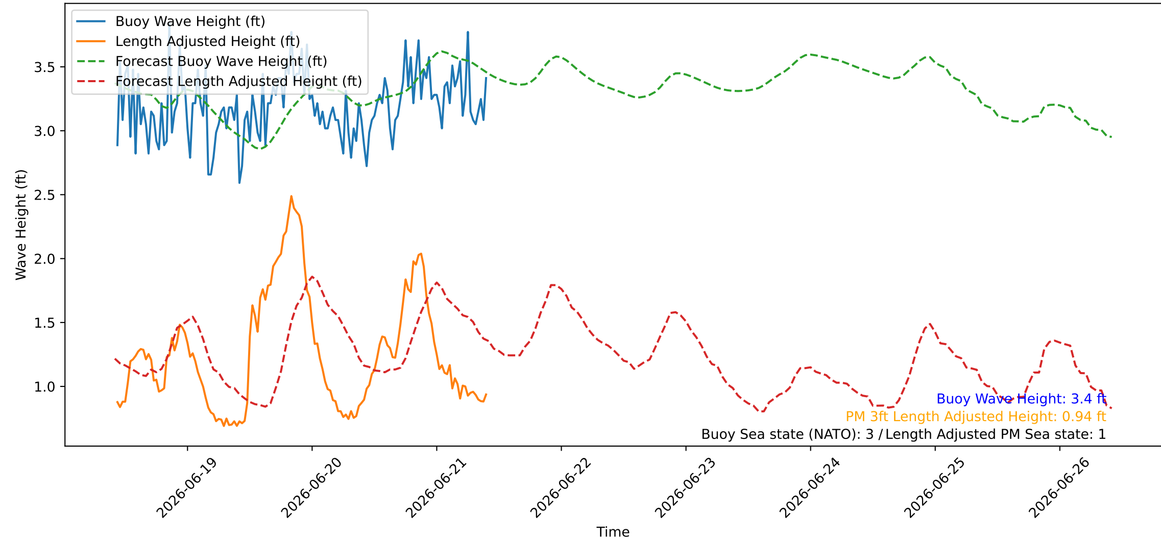
Wave Heights over Time for Red Beach at 2026-06-21 10:10:45
