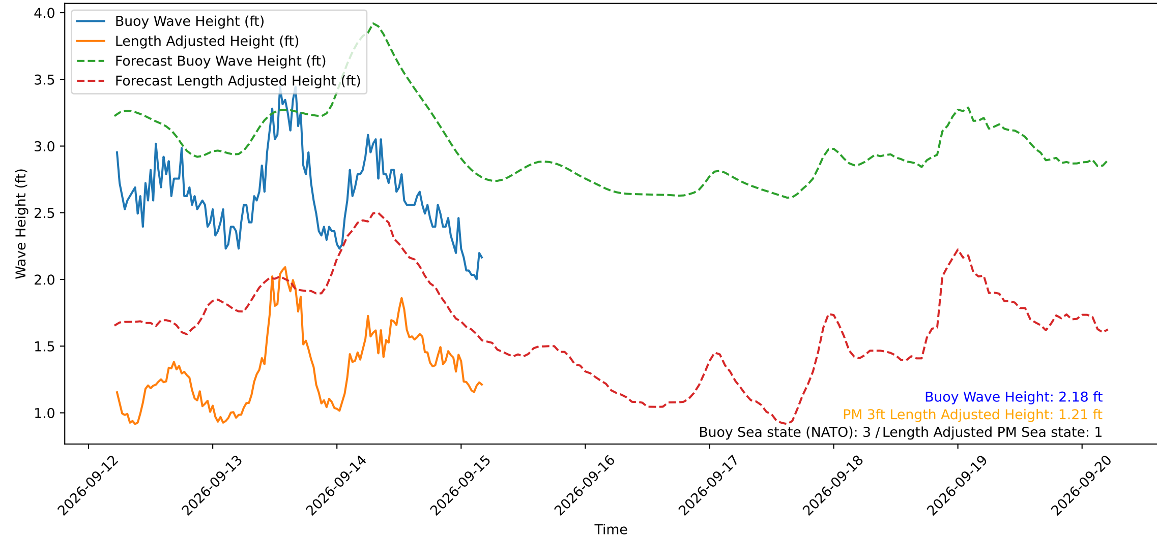
Wave Heights over Time for Red Beach at 2026-09-15 05:00:49
