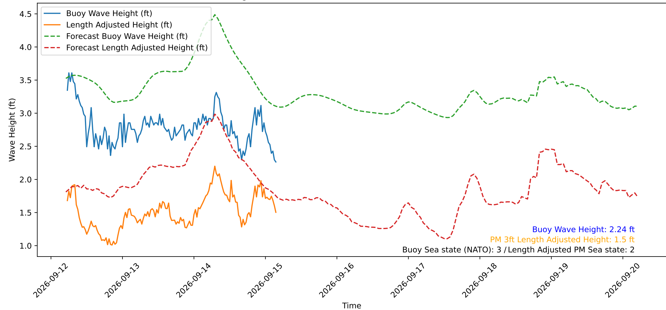
Wave Heights over Time for Green Beach at 2026-09-15 05:01:12
