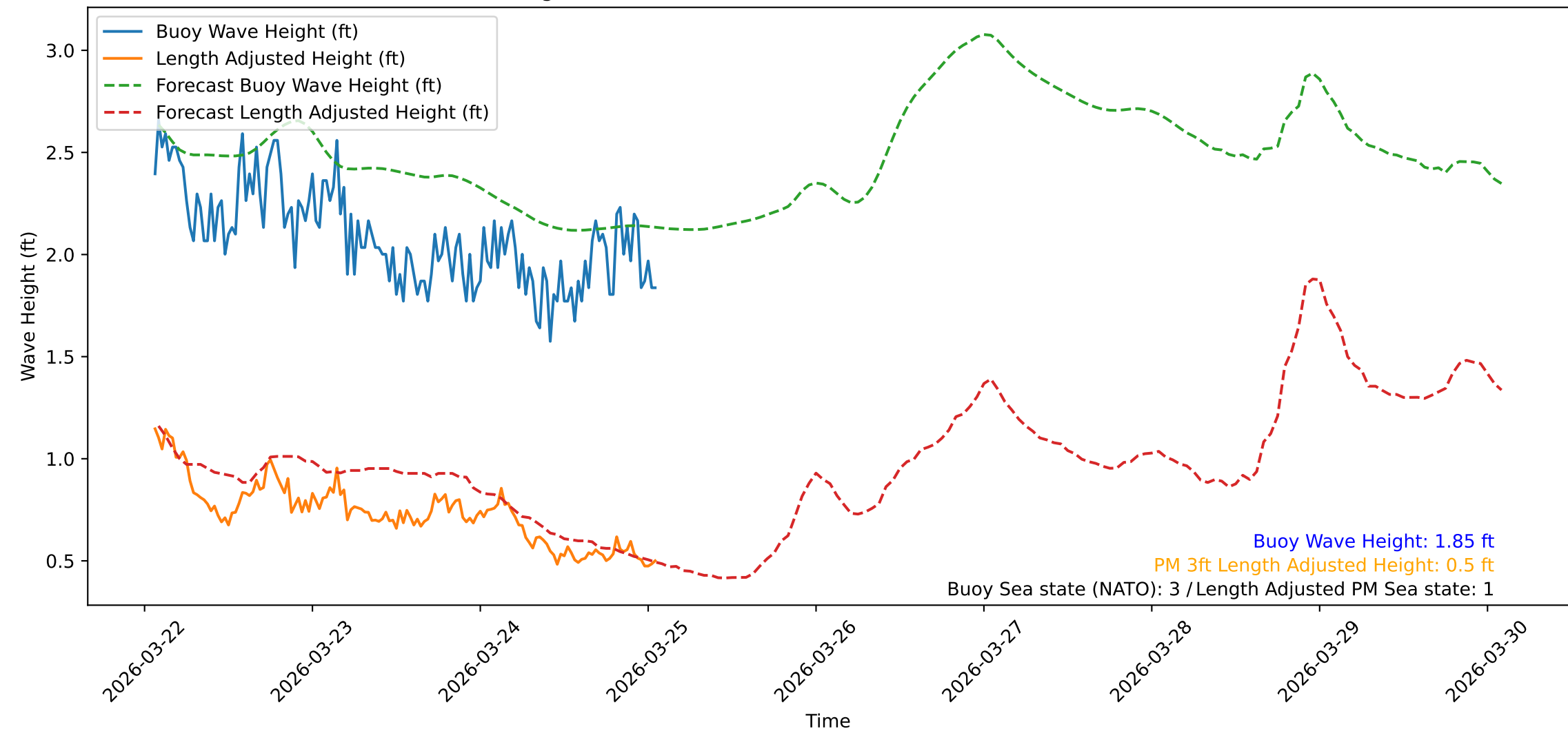
Wave Heights over Time for Oceanside Harbor at 2026-03-25 01:40:32
