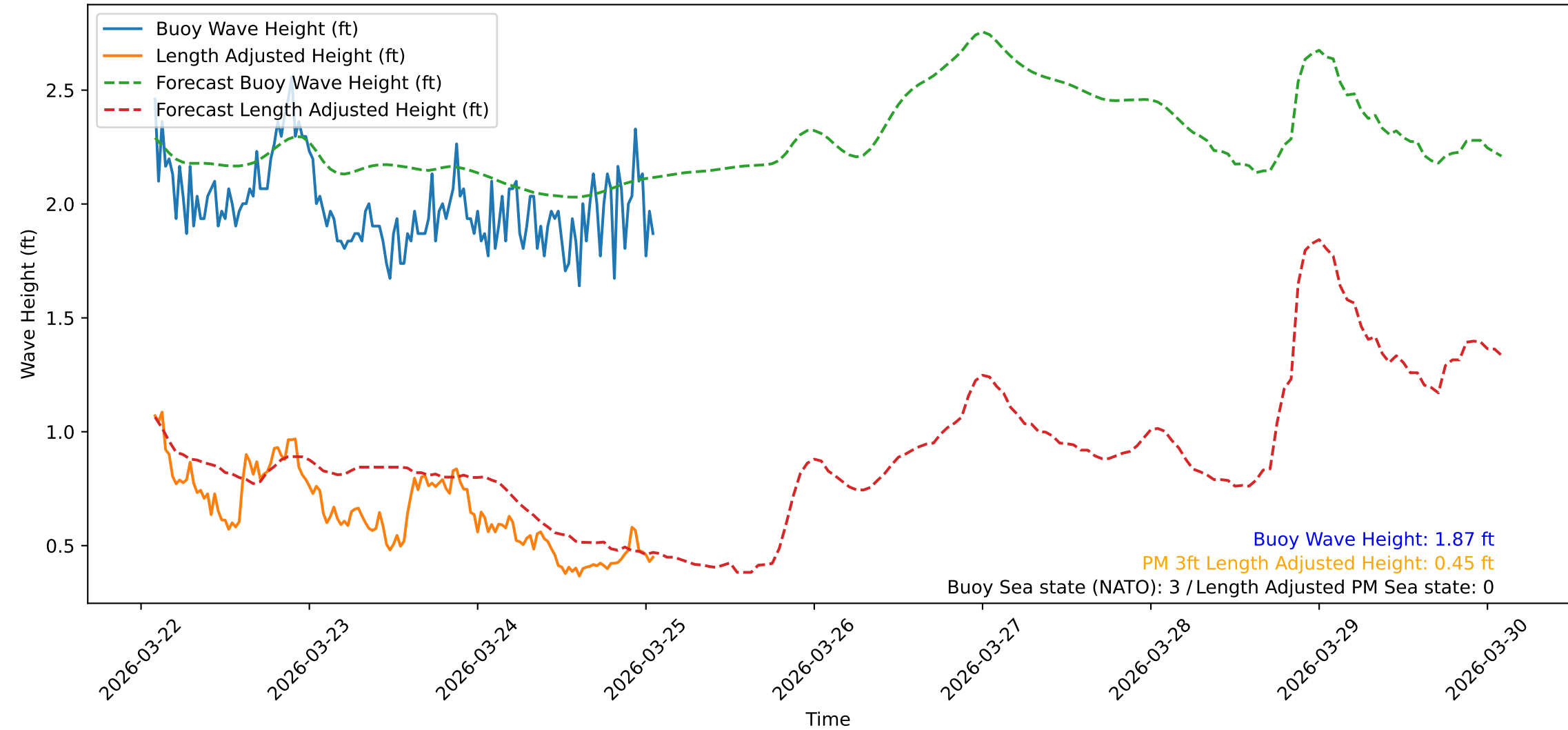
Wave Heights over Time for Red Beach at 2026-03-25 01:40:48
