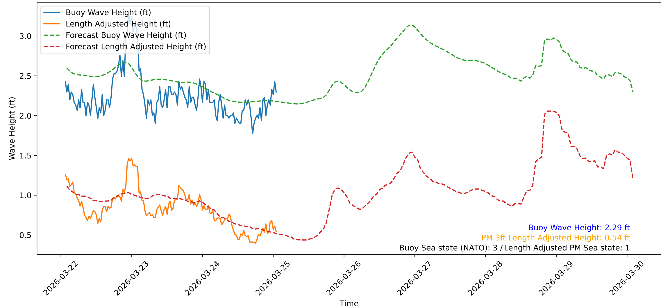
Wave Heights over Time for Green Beach at 2026-03-25 01:41:10
