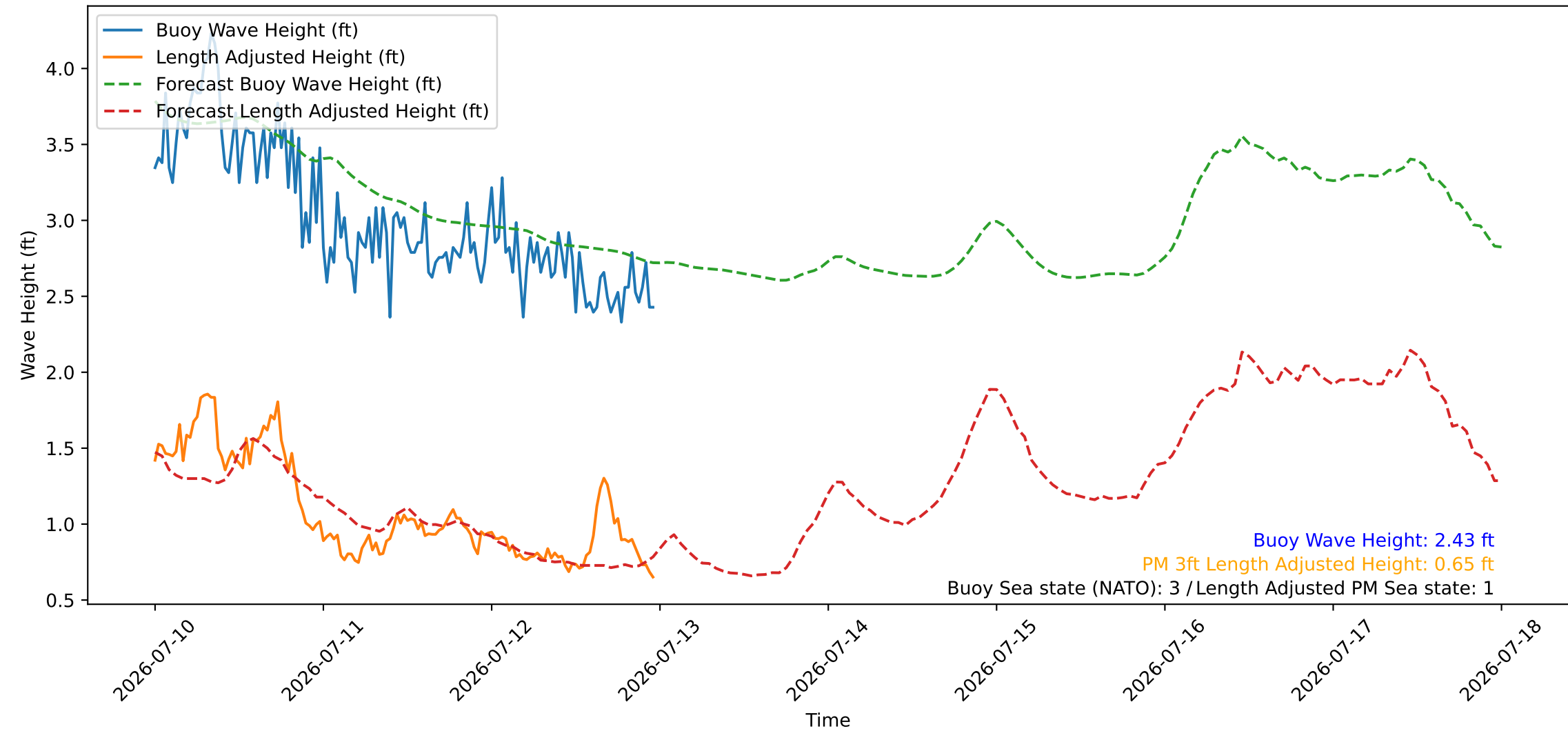
Wave Heights over Time for Oceanside Harbor at 2026-07-12 23:50:26
