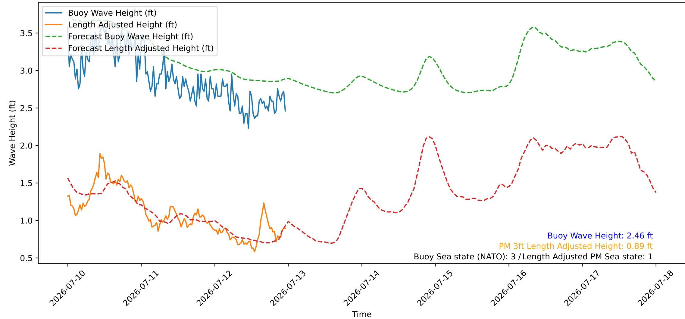
Wave Heights over Time for Green Beach at 2026-07-12 23:51:09
