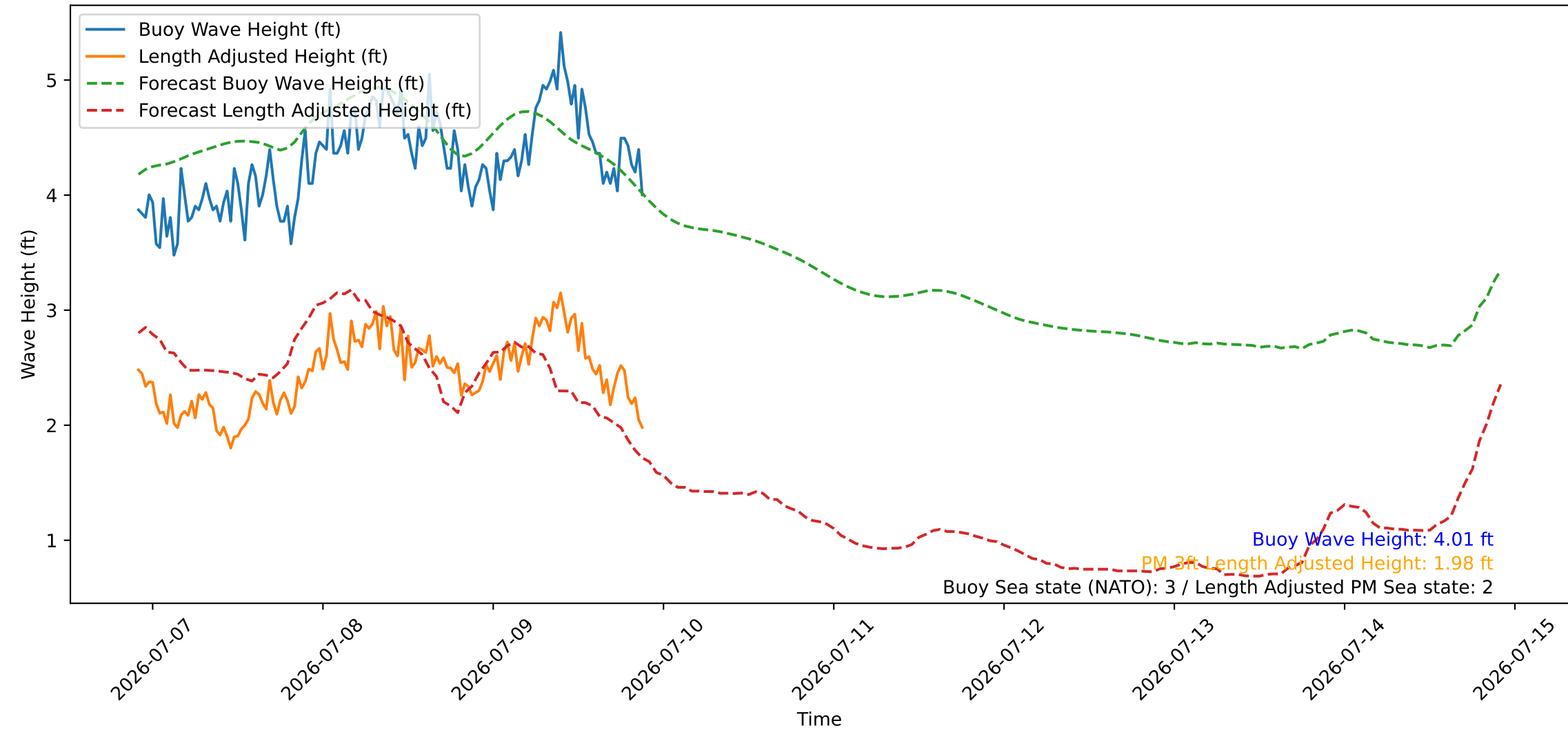
Wave Heights over Time for Oceanside Harbor at 2026-07-09 22:00:27
