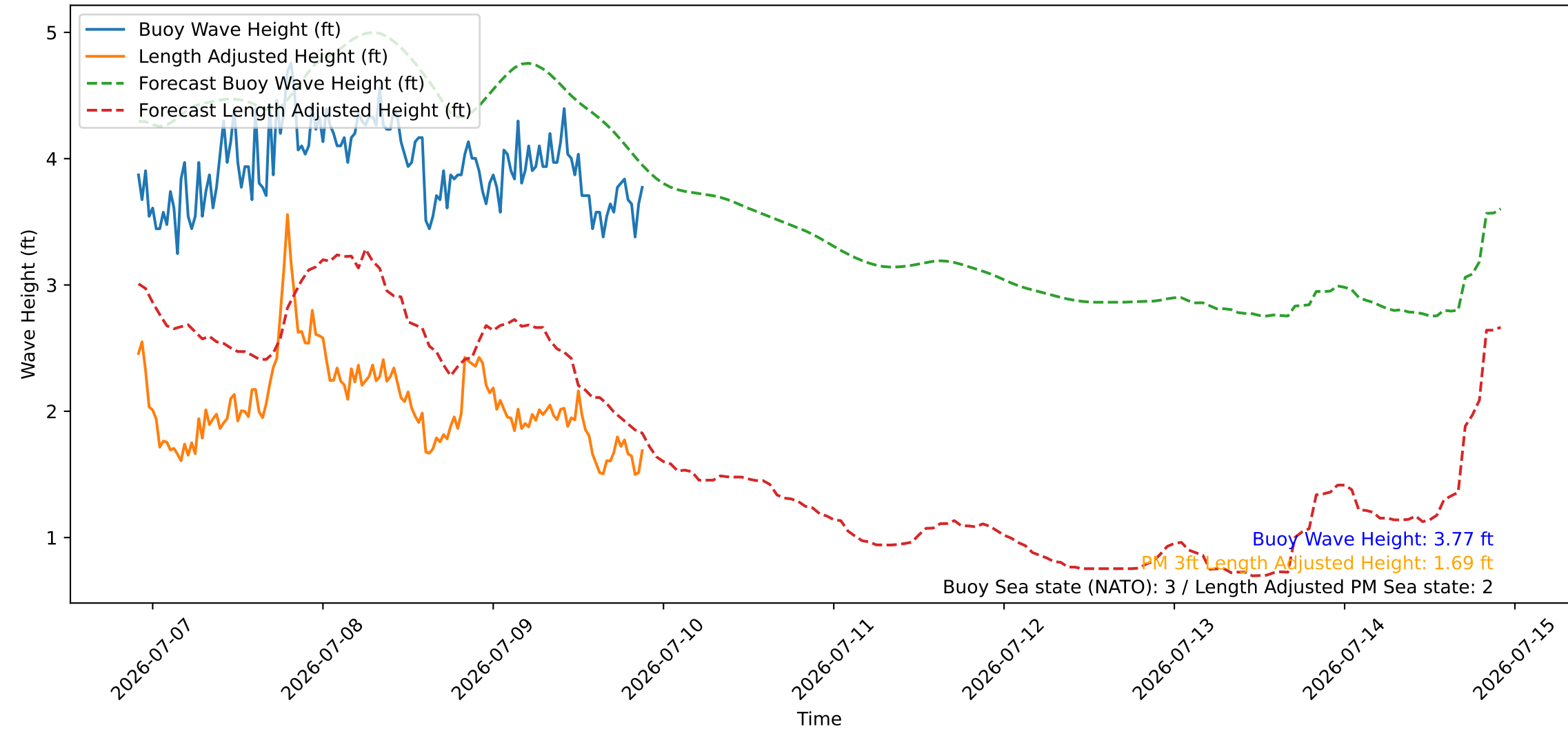
Wave Heights over Time for Green Beach at 2026-07-09 22:01:08
