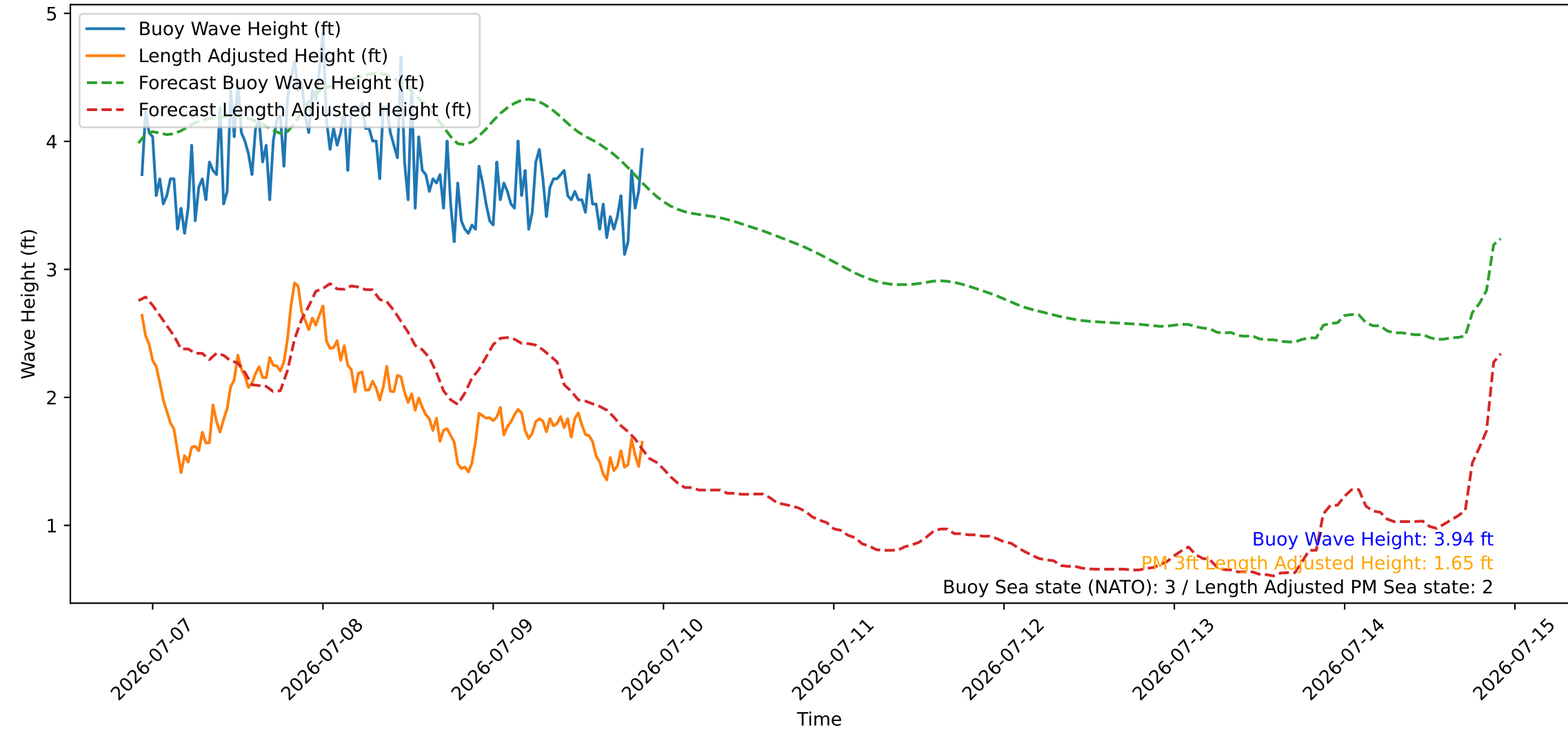
Wave Heights over Time for Red Beach at 2026-07-09 22:00:46
