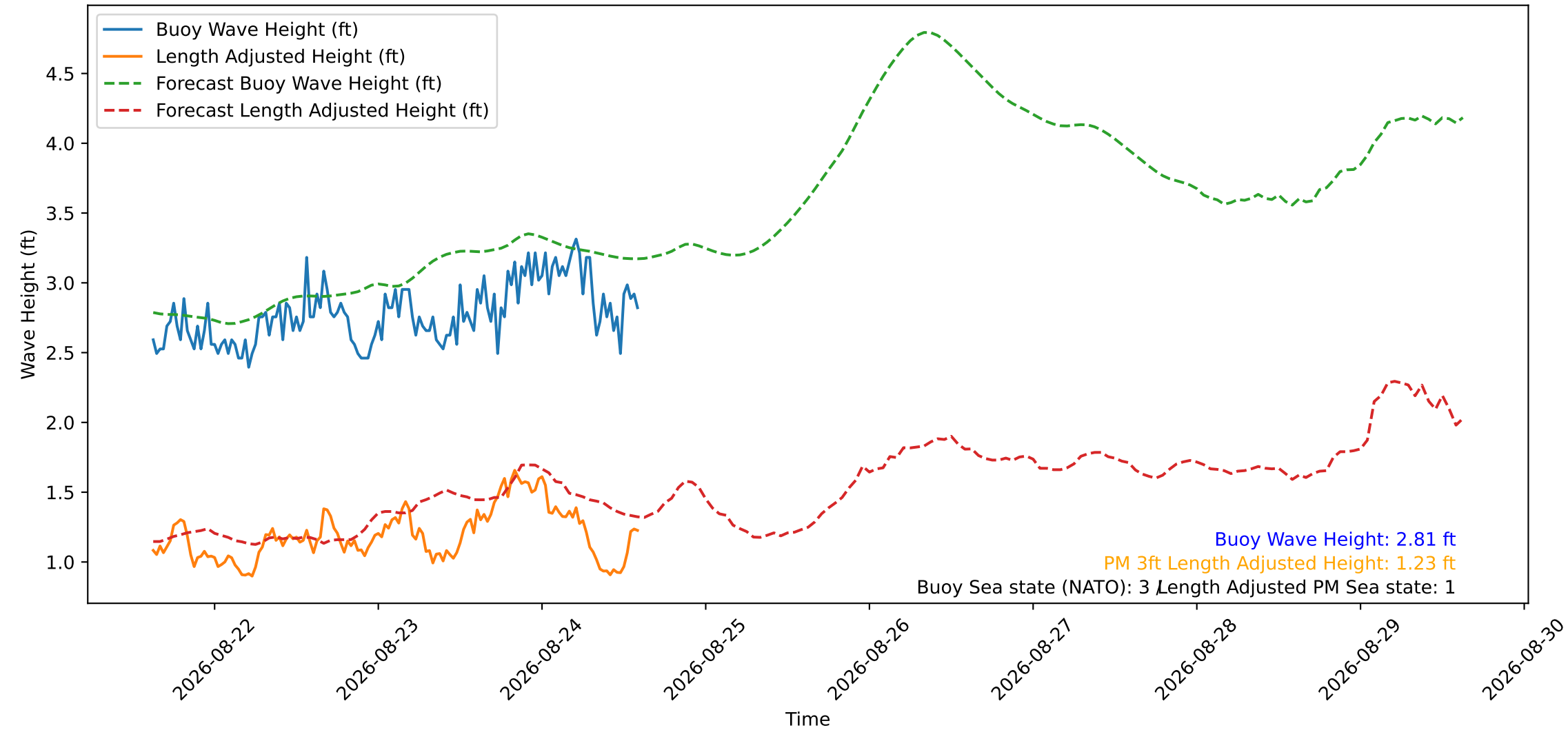
Wave Heights over Time for Green Beach at 2026-08-24 14:51:13
