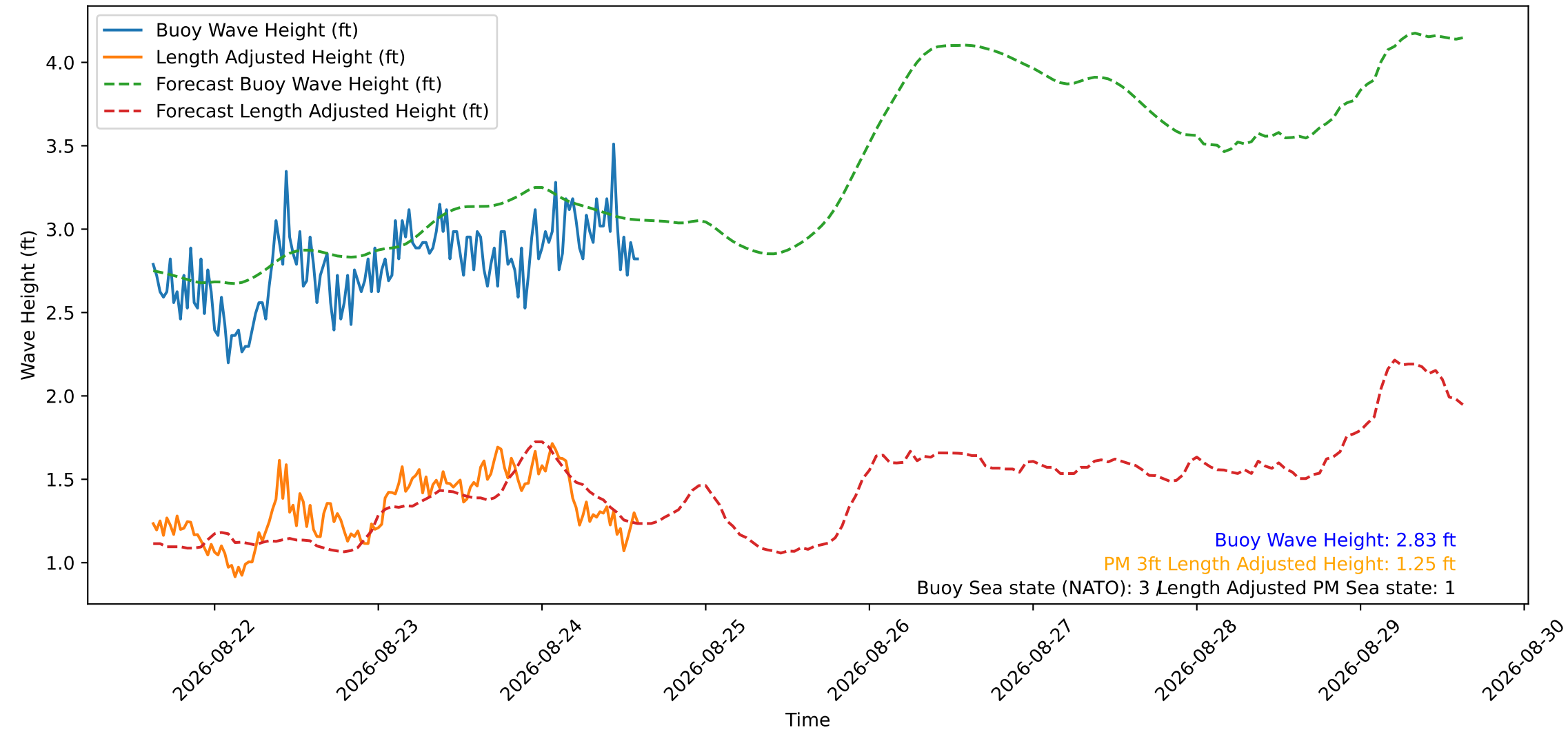
Wave Heights over Time for Oceanside Harbor at 2026-08-24 14:50:29
