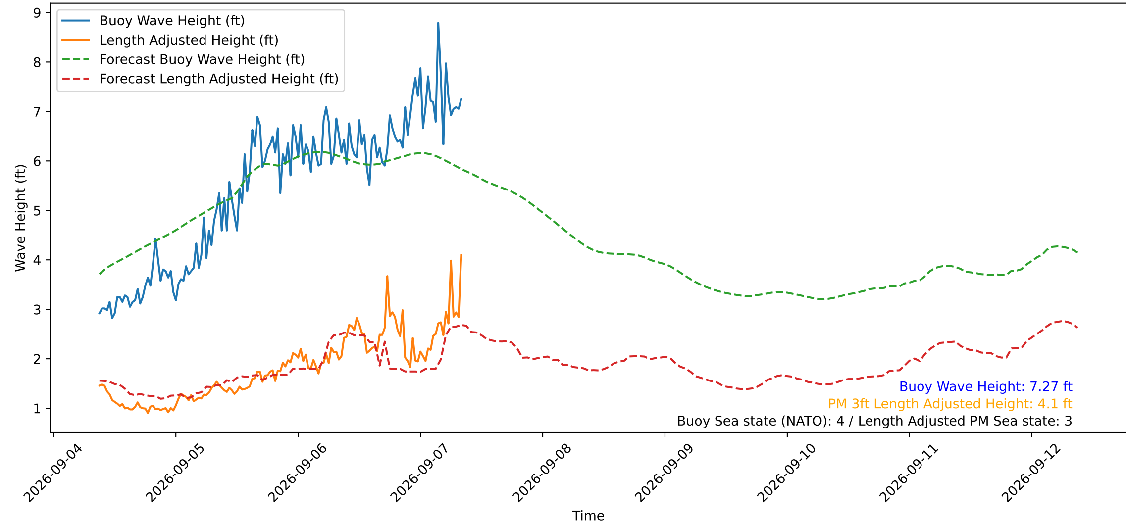
Wave Heights over Time for Green Beach at 2026-09-07 08:41:12
