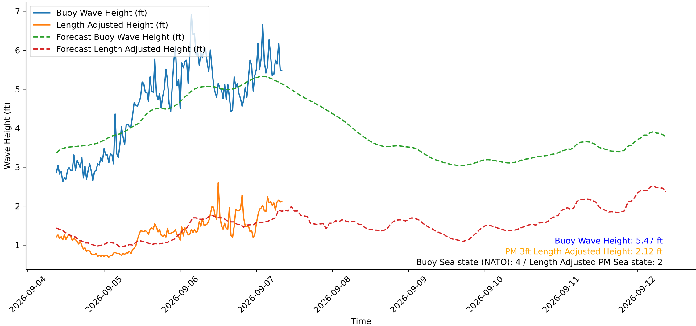
Wave Heights over Time for Red Beach at 2026-09-07 08:40:49
