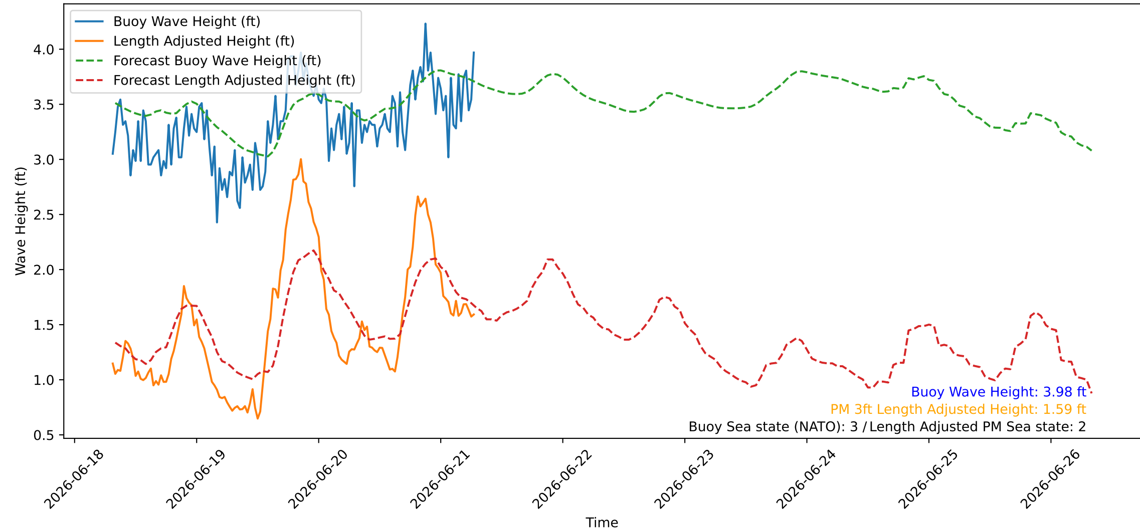
Wave Heights over Time for Green Beach at 2026-06-21 07:31:07
