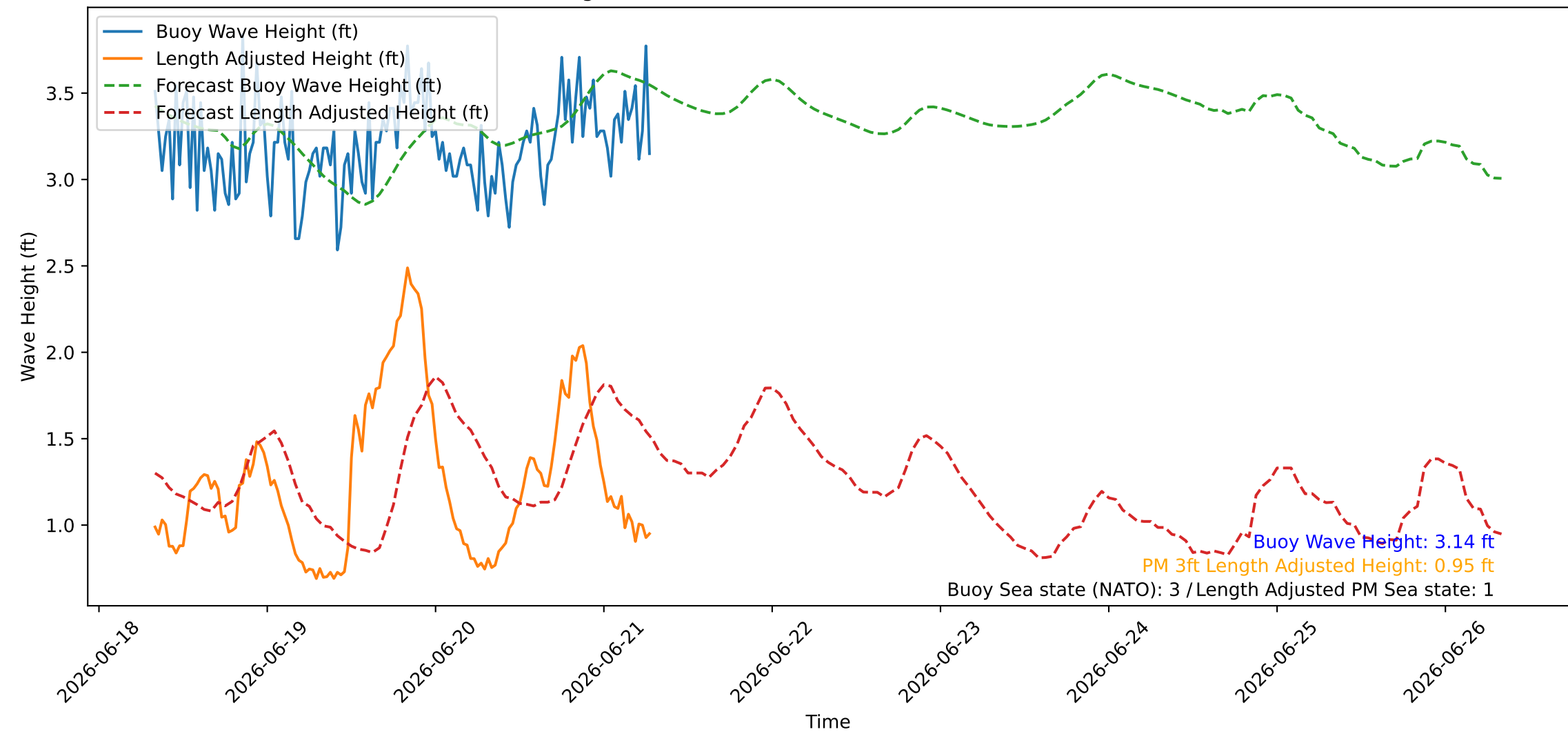
Wave Heights over Time for Red Beach at 2026-06-21 07:30:45
