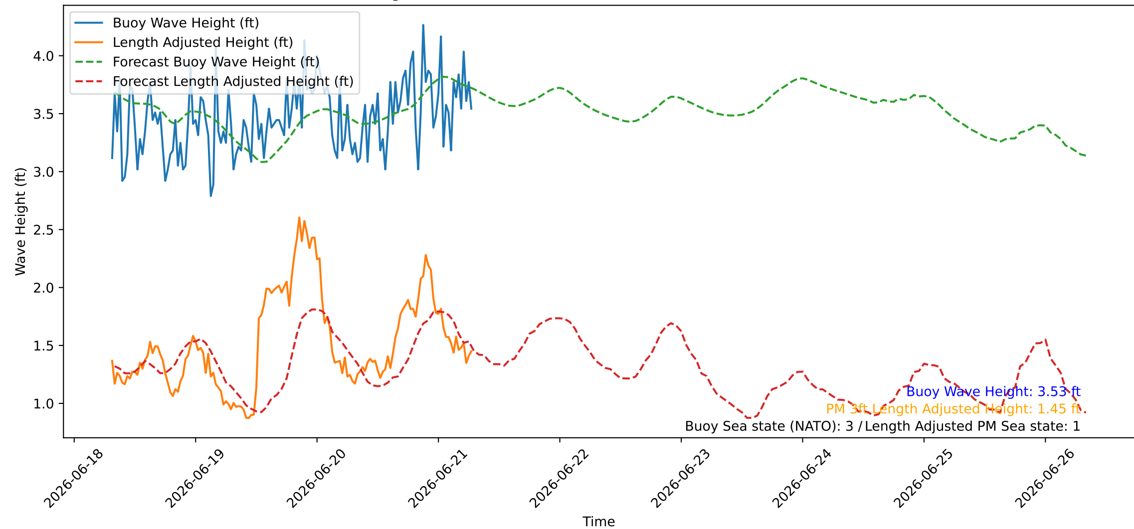
Wave Heights over Time for Oceanside Harbor at 2026-06-21 07:30:26
