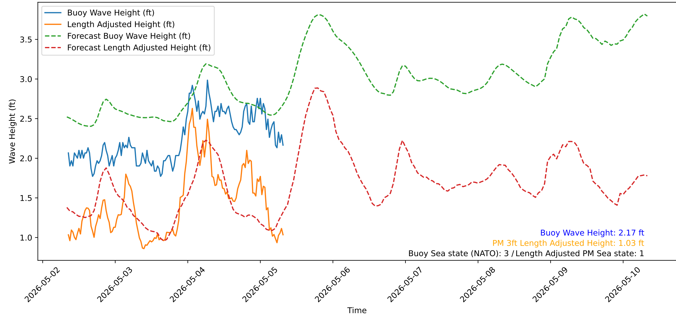
Wave Heights over Time for Green Beach at 2026-05-05 08:21:15
