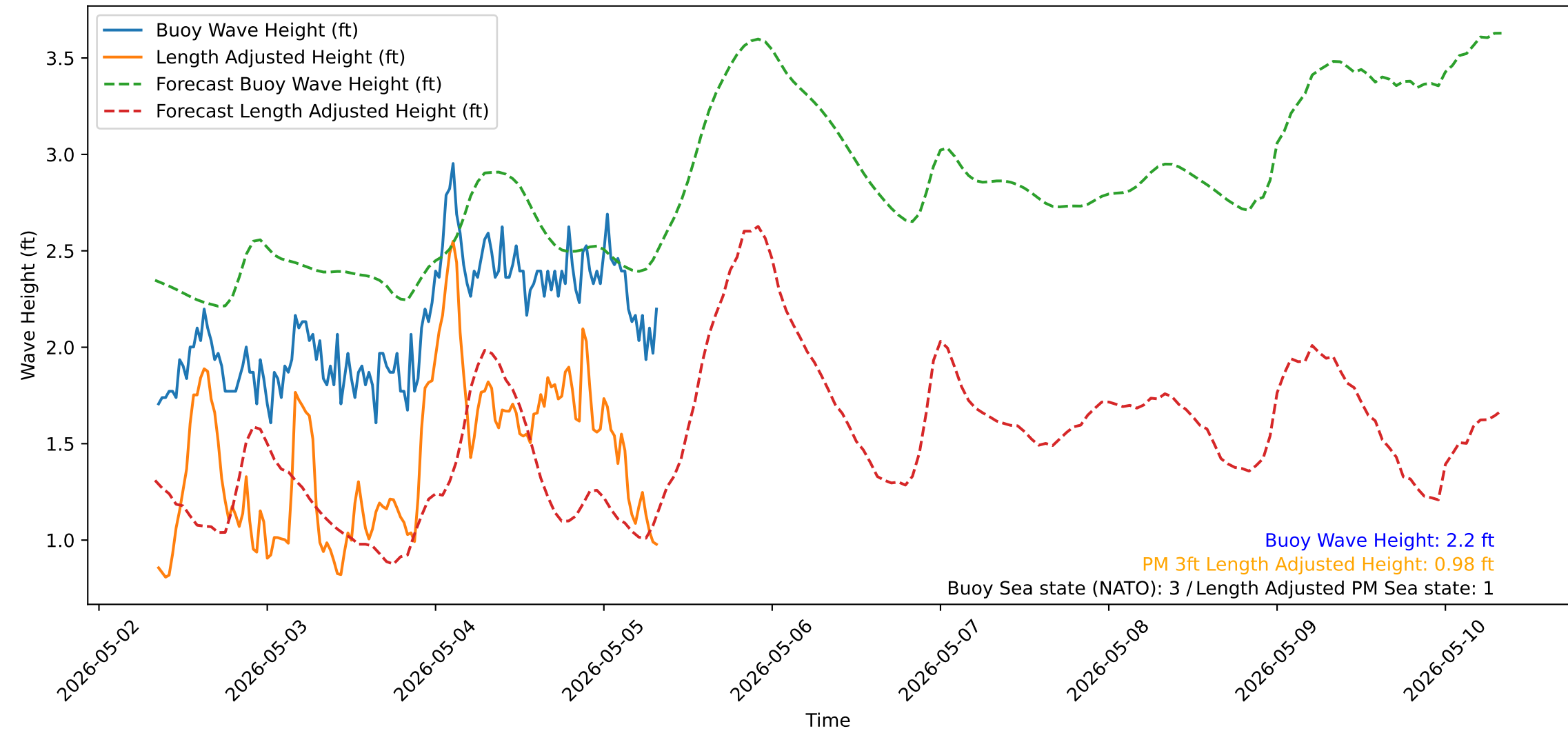
Wave Heights over Time for Red Beach at 2026-05-05 08:20:52
