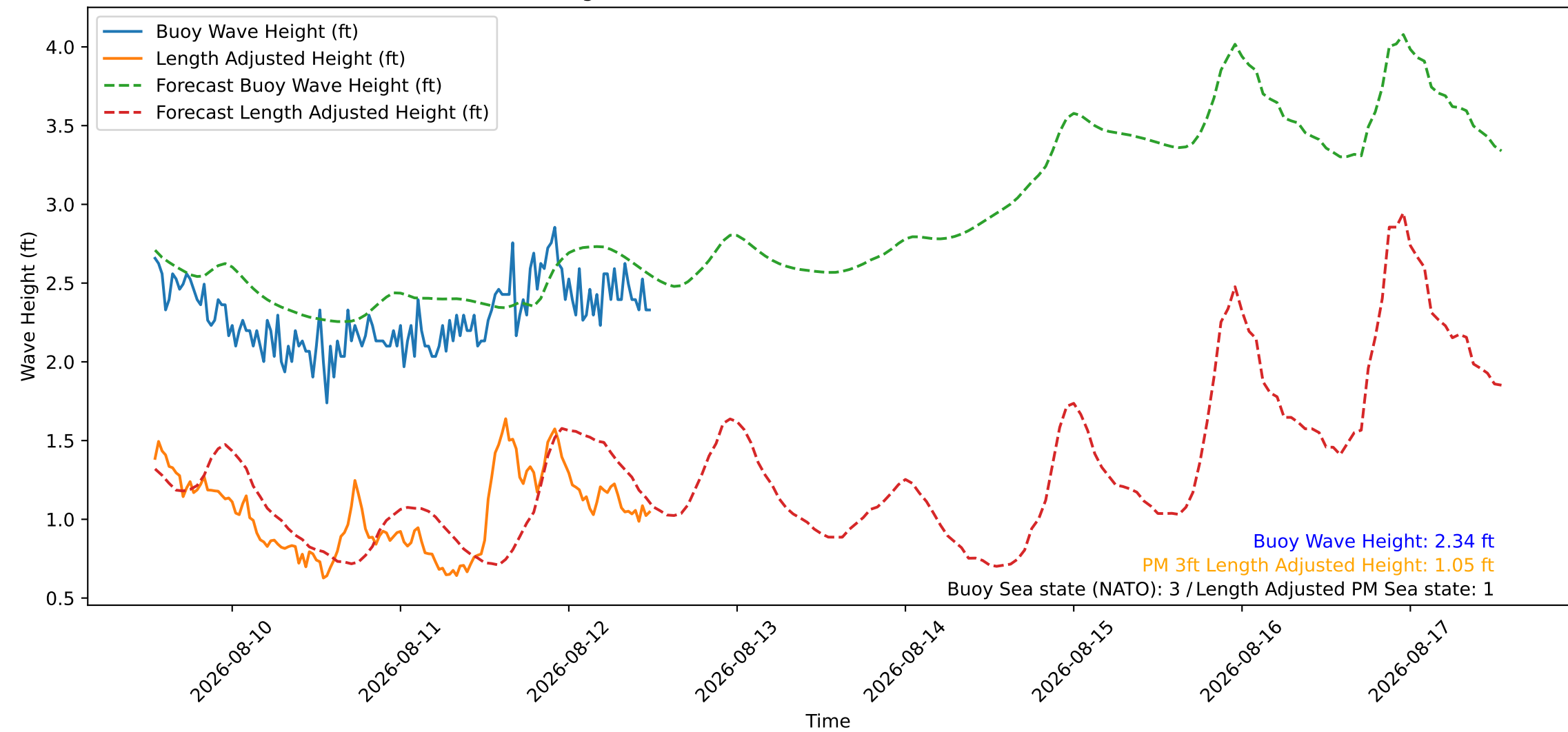
Wave Heights over Time for Red Beach at 2026-08-12 12:30:46
