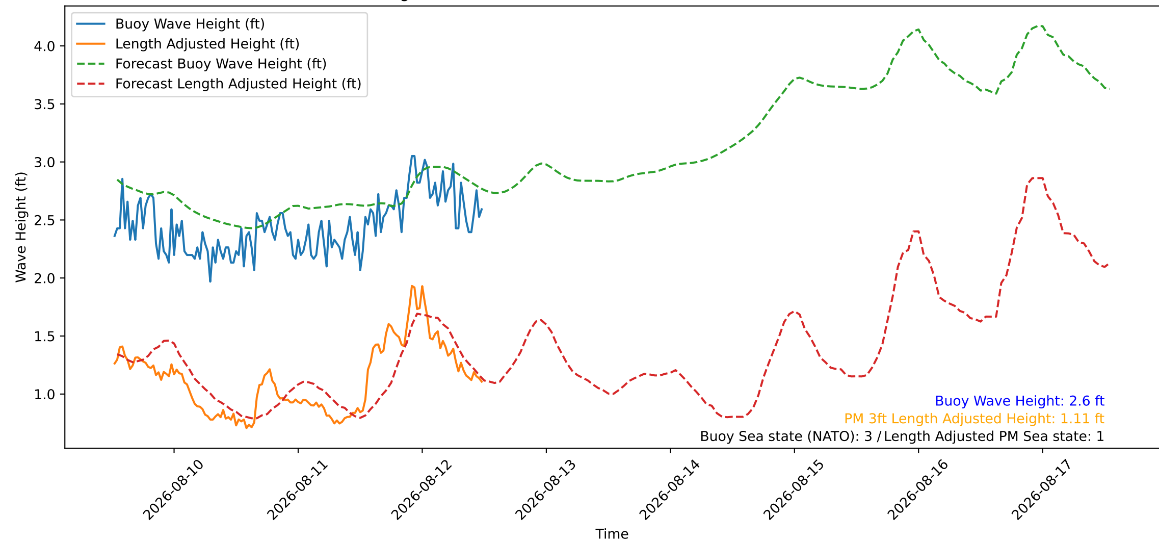
Wave Heights over Time for Oceanside Harbor at 2026-08-12 12:30:26
