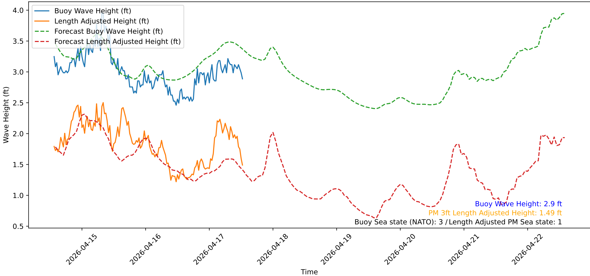
Wave Heights over Time for Green Beach at 2026-04-17 13:31:14
