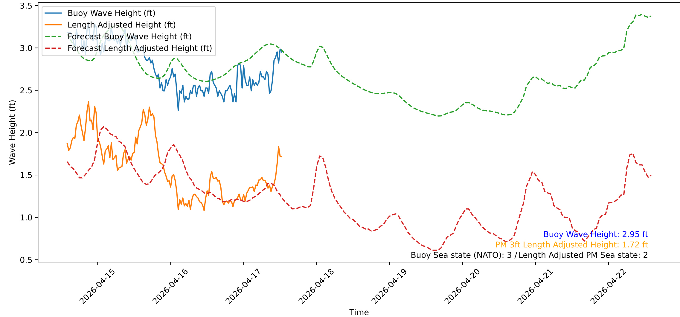
Wave Heights over Time for Red Beach at 2026-04-17 13:30:51
