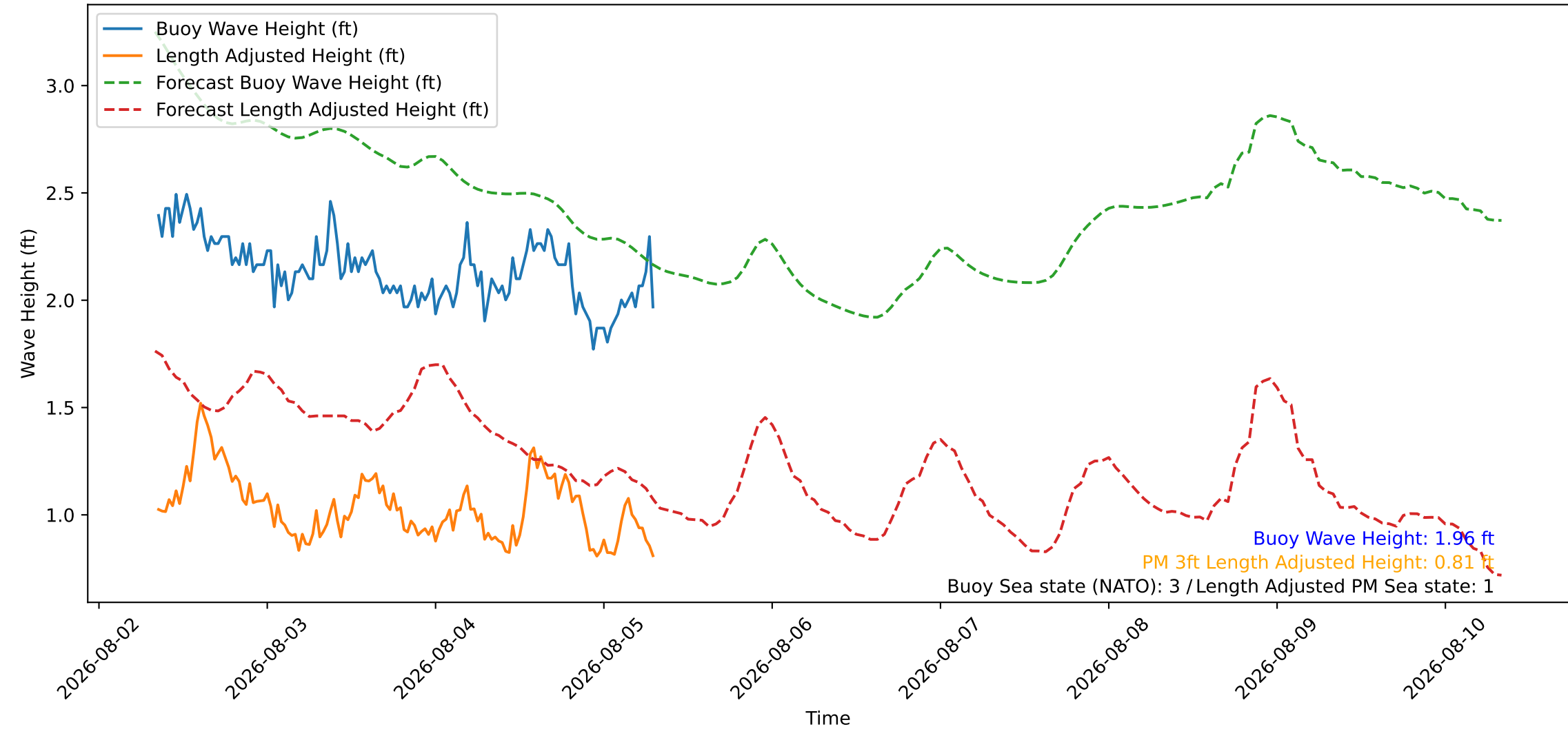
Wave Heights over Time for Red Beach at 2026-08-05 08:10:45
