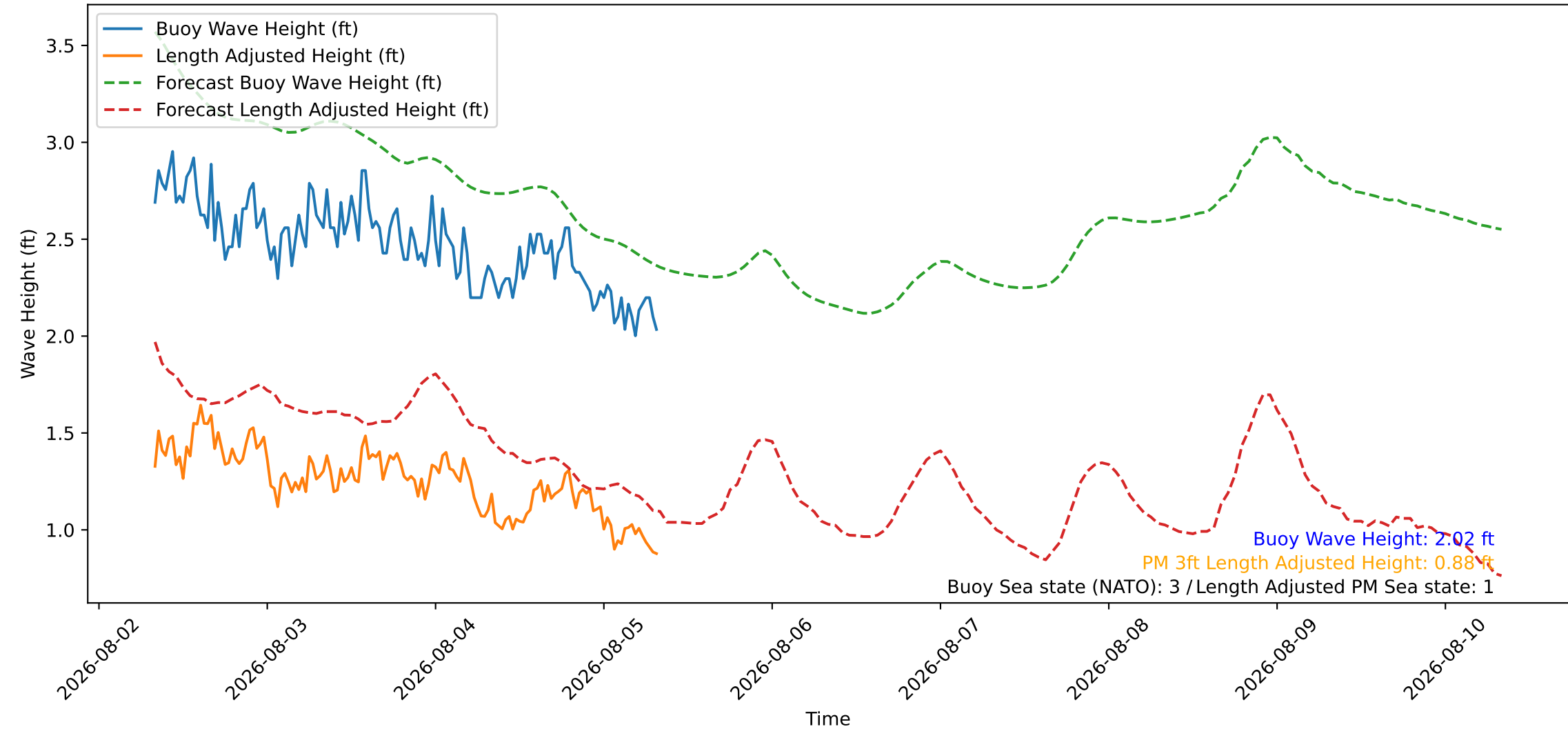
Wave Heights over Time for Oceanside Harbor at 2026-08-05 08:10:26
