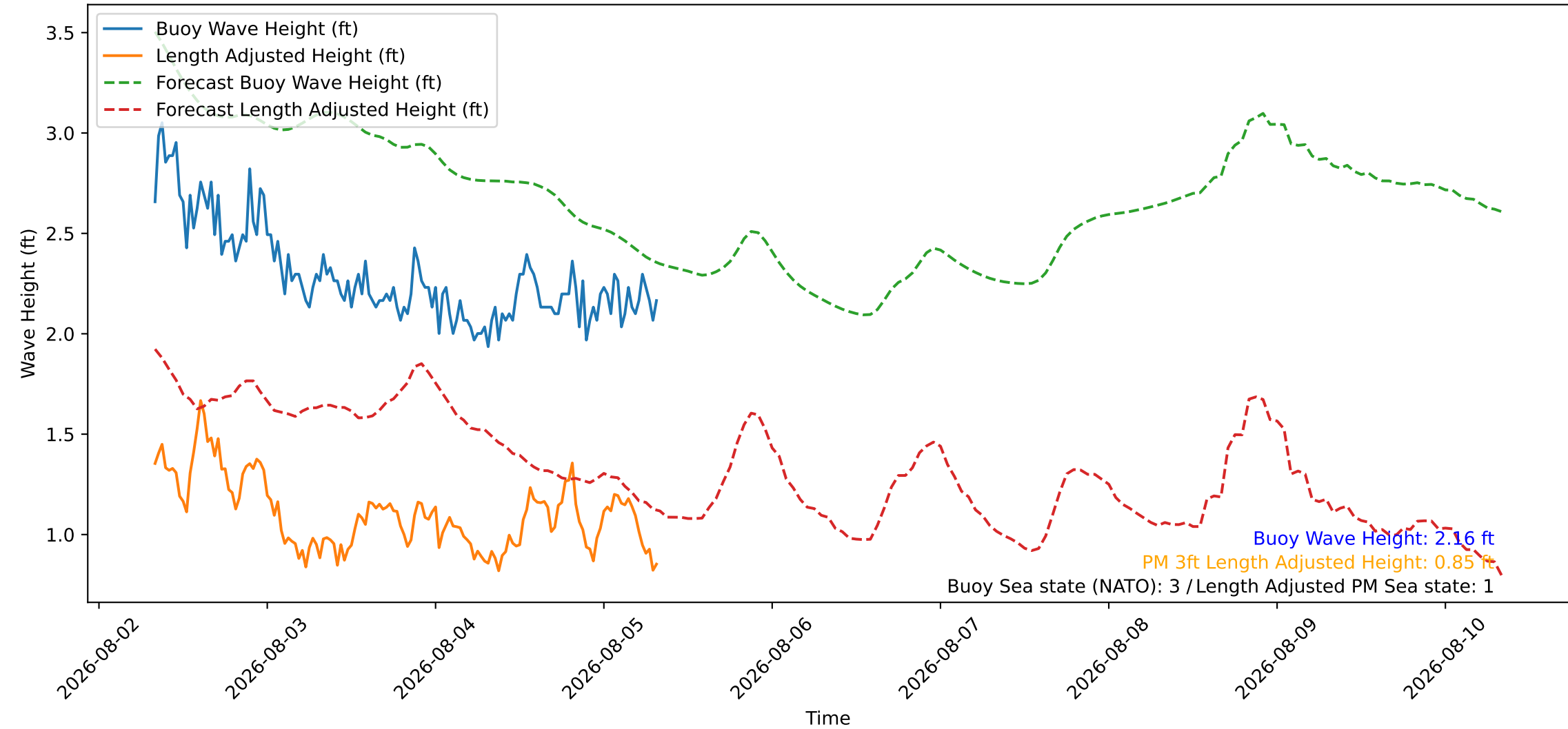
Wave Heights over Time for Green Beach at 2026-08-05 08:11:08
