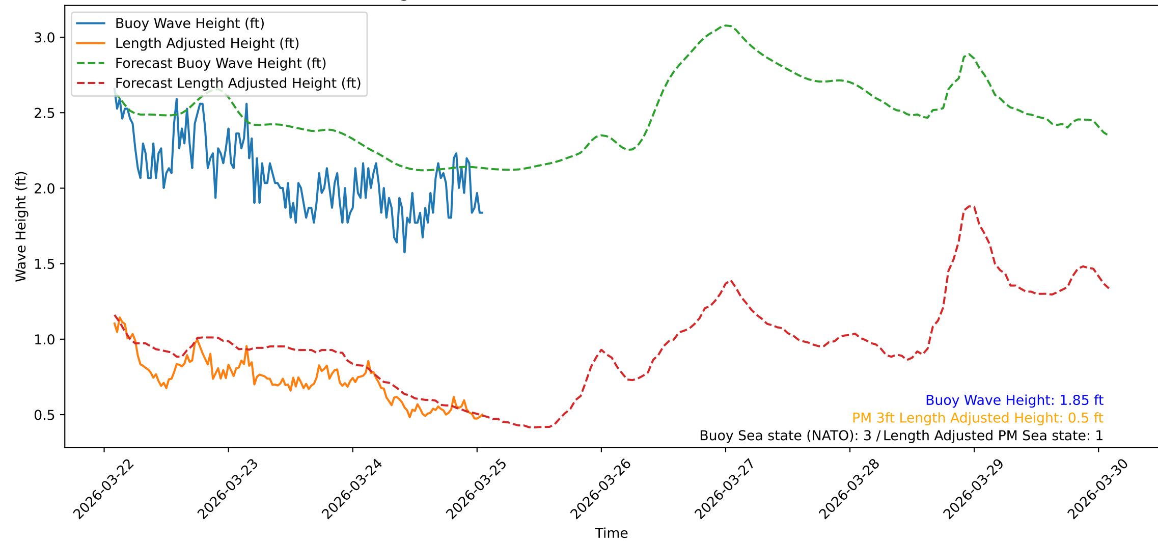
Wave Heights over Time for Oceanside Harbor at 2026-03-25 02:00:31
