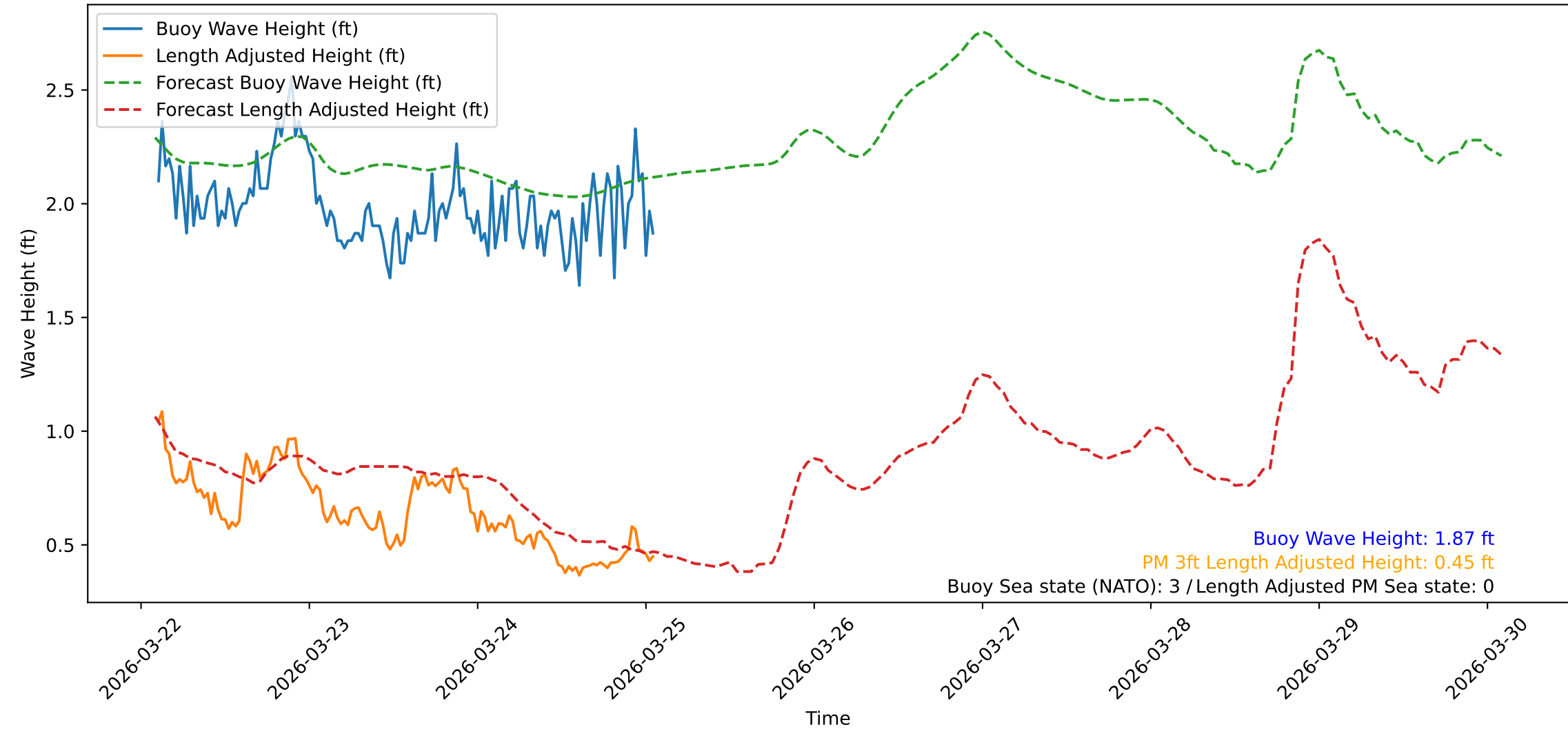
Wave Heights over Time for Red Beach at 2026-03-25 02:00:47
