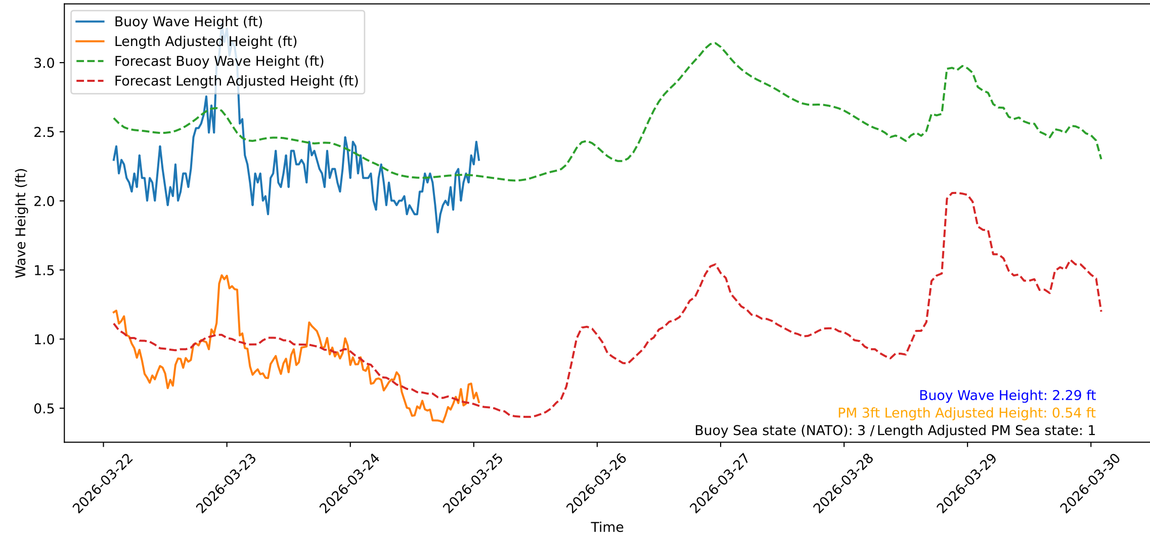
Wave Heights over Time for Green Beach at 2026-03-25 02:01:08
